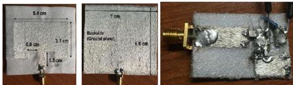
Figure 2.41: Rectenna fabricated onto fabric-based substrates [107].
