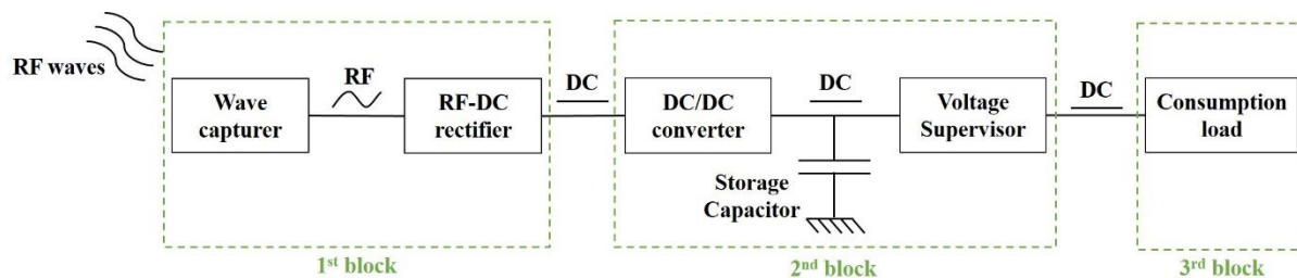
Figure 0.1: Schematic block of a RFEH
