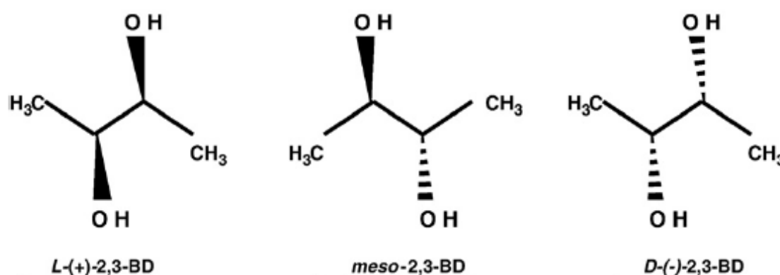
Figure 2.1 The stereoisomers of 2,3-butanediol (2,3-BD). (Celińska and Grajek, 2009).
