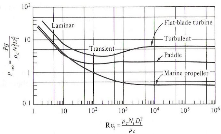
Figure A.1 The correlation between power number ( P_{no} ) and Reynolds number ( Re_i ).
