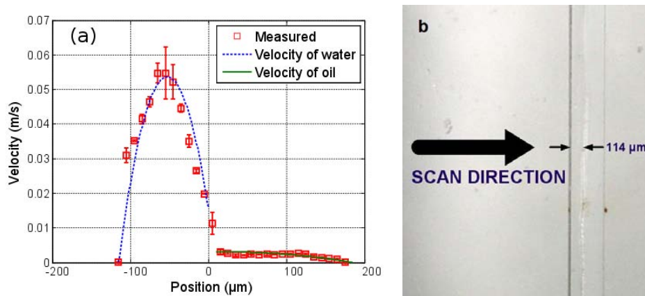
Fig. 4.18. Measured maximum velocity profile with the dual lens configuration and theoretical fitting for water pumped at 20 \mu\text{L}/\text{min} and oil pumped at 1.5 \mu\text{L}/\text{min} (a). Reference image indicating the scan (b).
