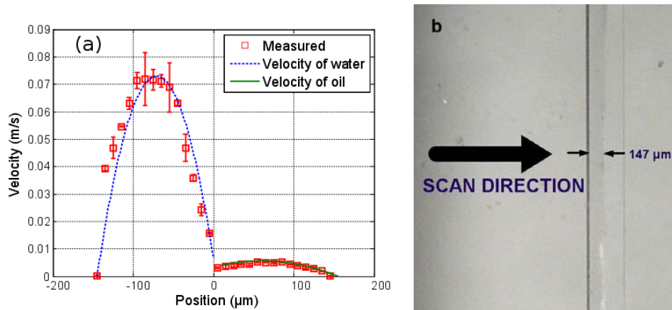
Fig. 4.16. Measured maximum velocity profile with the dual lens configuration and theoretical fitting for water pumped at 35 \mu\text{L}/\text{min} and oil pumped at 3 \mu\text{L}/\text{min} (a). Reference image indicating the scan (b).
