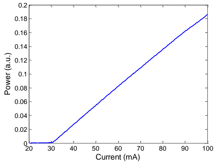
Fig. 2.8. Light-current curve of the laser L785P090. The power is represented by the photocurrent amplified through the first stage transimpedance amplifier, which has a gain of 1 k \Omega .
