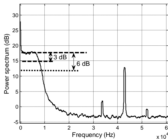
Fig. 3.15. Power spectrum of the OFI signal corresponding to a flow rate of 40 μl/min. The threshold levels below the plateau represent the cutoff frequencies used to generate the Fig. 3.14.
