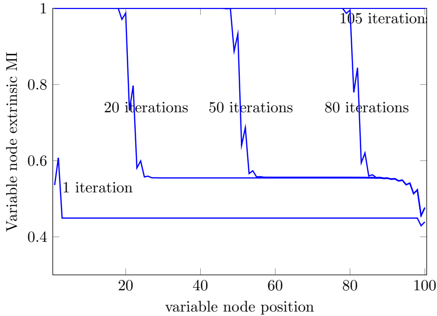
Figure D.4: VNs' MI evolution through iterations for DT (3,6)-regular LDPC code with MSEW mapping at E_b/N_0 = 5.18\text{dB} and L = 50
