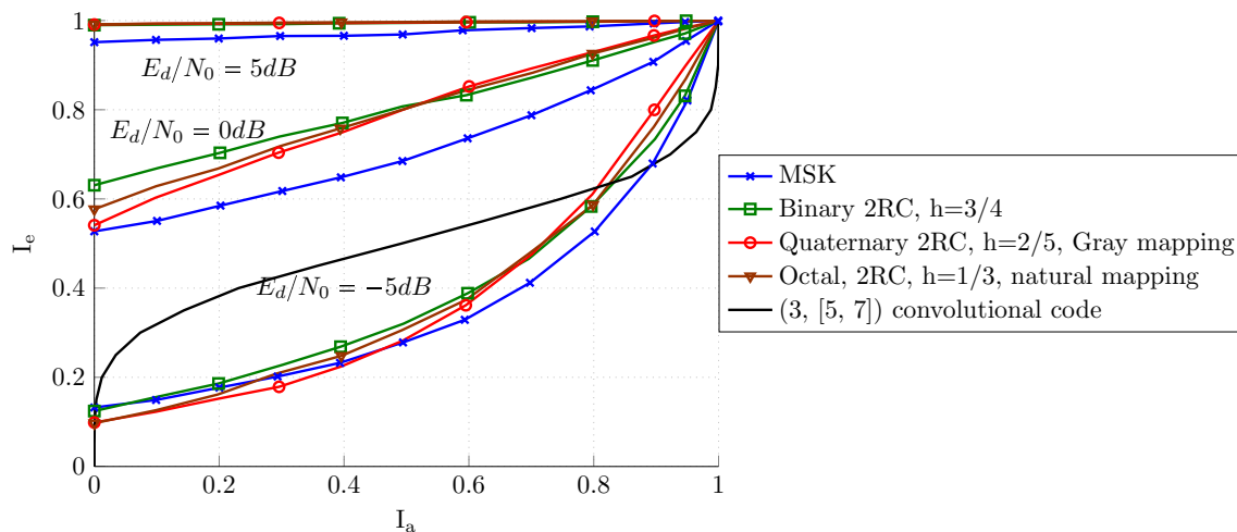
Figure 2.8: EXIT curves for various CPM systems. For reference the rate-1/2 [5, 7] convolutional code is also illustrated. The considered SNRs are E_d/N_0 = -5, 0 and 5 dB
