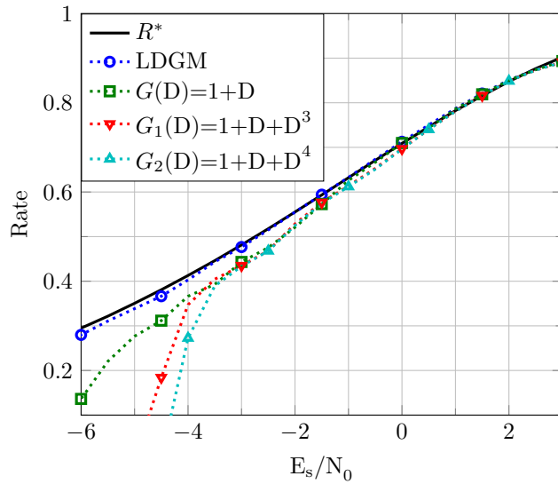
Figure 3.10: Achievable and optimized rates when VNs degrees are constrained to be \geq 1
