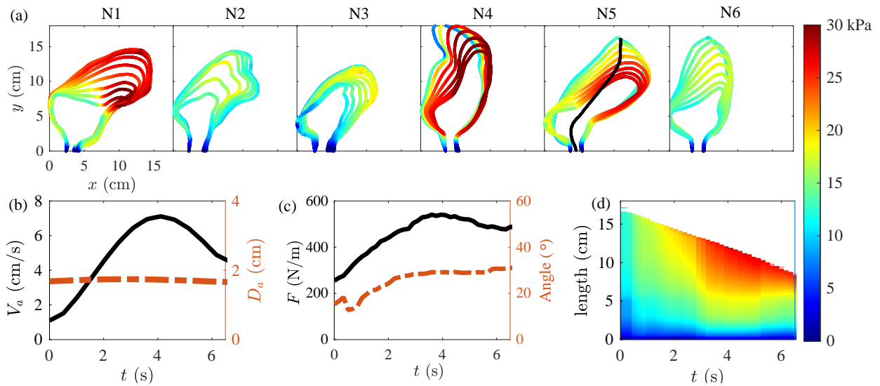
FIG. 2: Simulations of normal rectal evacuations through the open anal canal. (a) Evolution of the boundaries of the rectum during the evacuation of the neostool for 6 patients showing a normal rectal function. The color code shows the magnitude of the wall normal stress WNS. (b) Example of mean outlet velocity of the neostool through the anal canal V_a (plain lines, left axis) and diameter of the anal canal D_a (dashed lines, right axis) as a function of time (patient N5). (c) The evacuation force F (plain lines, left axis) and its angle with the y axis (dashed lines, right axis) as a function of time for patient N5 (d) Spatio-temporal map of the pressure variation along the length of a mid-line going from the anal canal (0 cm) to the proximal end at time 0 (black line in a-N5).
