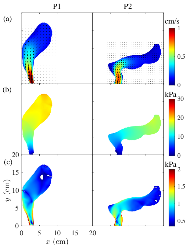
FIG. 5: Flow fields (a), pressure fields (b) and viscous stress fields (c) of 2 pathologic evacuations when the mean outlet velocity of the neostool through the anal canal V_a was maximal. White color in (c) corresponds to regions where the viscous stress is lower than the yield stress of the neostool.
