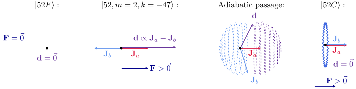
Figure IV.7: Simplified evolution of the classical atomic dipole \mathbf{d} throughout the preparation of a single atom. The atom is excited to |52F\rangle in zero electric field, such that the static dipole only emerges when ramping \mathbf{F} up, to branch the low- \ell state onto the state |52, m = 2, k = -47\rangle of the manifold, written in the parabolic basis. Then, the dipole is independent of \mathbf{F} and proportional to \mathbf{J}_a - \mathbf{J}_b . During the circularization, \mathbf{d} shrinks while precessing around the quantization axis as \mathbf{J}_b evolves ( m_b grows) to reach the circular state, where the static dipole is zero (up to first order in \mathbf{F} ). We suspect that the interactions between the classical dipoles of the two atoms in the pair lead to significant motion, induced before the adiabatic passage.
