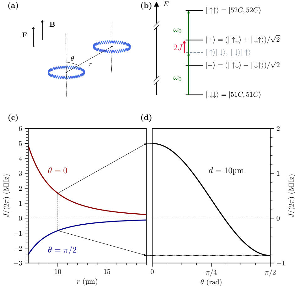
Figure I.4: (a) Geometry and parametrization of the system. The fields are taken to be F = 2 V/cm and B = 10 G for the energy computations. (b) Level scheme for the interacting pair states: the energy splitting between |+\rangle and |-\rangle is given by 2J . The two other states |\uparrow\uparrow\rangle and |\downarrow\downarrow\rangle lie tens of GHz away from them due to the bare atomic energies: \omega_0 is the single spin-flip energy, between |51C\rangle and |52C\rangle . (c) Variation of J with the distance r , for both \theta = 0 (red) and \theta = \pi/2 (blue). (d) Variation of J with the angle \theta , at a distance of 10\ \mu\text{m} . For \theta = \theta_0 \simeq 54.7^\circ , J = 0 and the two atoms do not interact.
