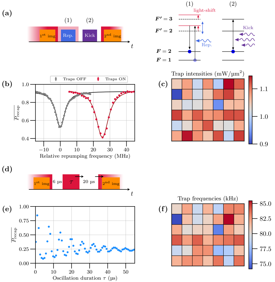
Figure II.7: Tweezer characterization. (a) Sequence of events and level evolution. The tweezer activation is shown in red, with the traps ON or OFF (dimmed red part in the experimental sequence) during the repumper pulse to measure the light-shift induced by each trap on the F = 1 \rightarrow F' = 2 transition. The fading red in the sequence indicates links with previous (preparation) and subsequent (re-initialization) manipulations of the trapped atoms. (b) Recapture probability averaged over all sites, with and without the tweezers, and fitted with Lorentzian peaks. The averaged data yields the mean intensity \bar{I} = 1.065 \pm 0.003 \text{ mW}/\mu\text{m}^2 . (c) Site-by-site result of peak intensity for each trap. (d) Release-recapture experiment to measure the transverse trapping frequencies of the tweezers. (e) Averaged signal, displaying oscillations at 166 KHz. (f) Site-resolved transverse trapping frequencies.
