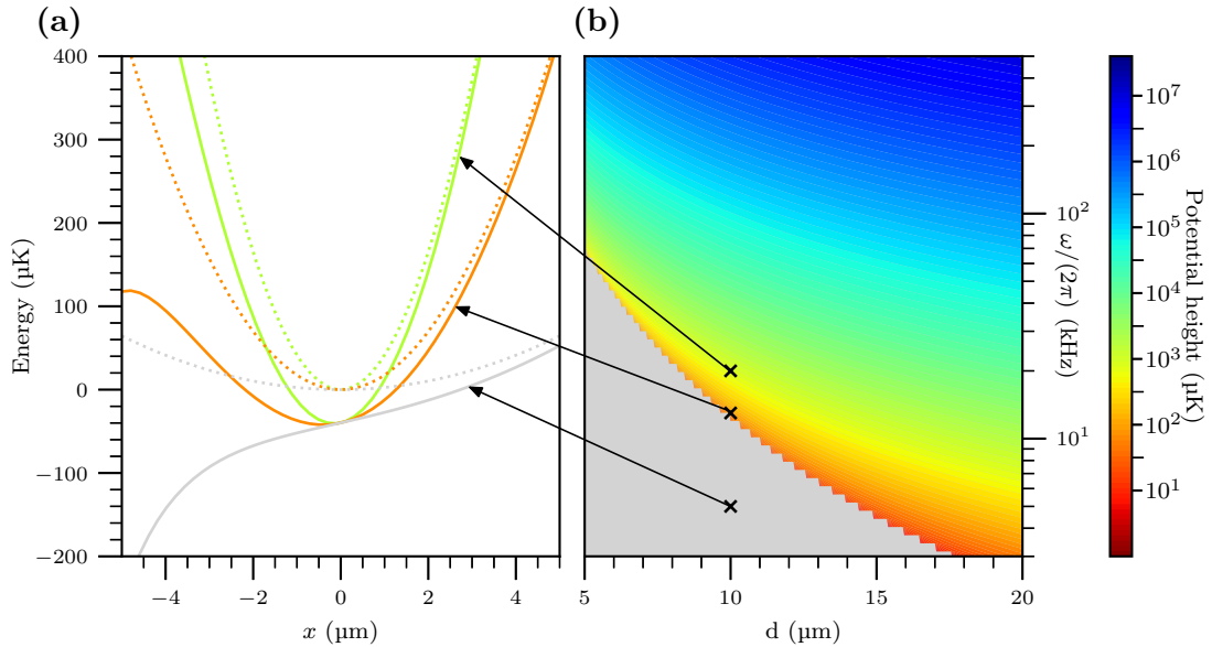
Figure B.1: Stability of the spin-phonon system, in the \Delta n = 1 and \theta = \pi/2 regime. (a) Bare harmonic traps (dotted lines) and effective potentials V_+ (solid lines), plotted as functions of the relative distance between the two atoms x , for three configurations illustrating the different behaviors of the system. At large trapping frequency (green), the interaction does not affect the shape of the trap at the relevant scales. In the intermediate regime (orange), the effective potential displays a “wall” of a few hundred \mu\text{K} . For a low trapping frequency (grey), the effective potential cannot trap atoms. (b) Map of the wall height as a function of d and \omega . The grey region indicates where the system is fully unstable. Experimental parameters should always be taken outside of this region.
