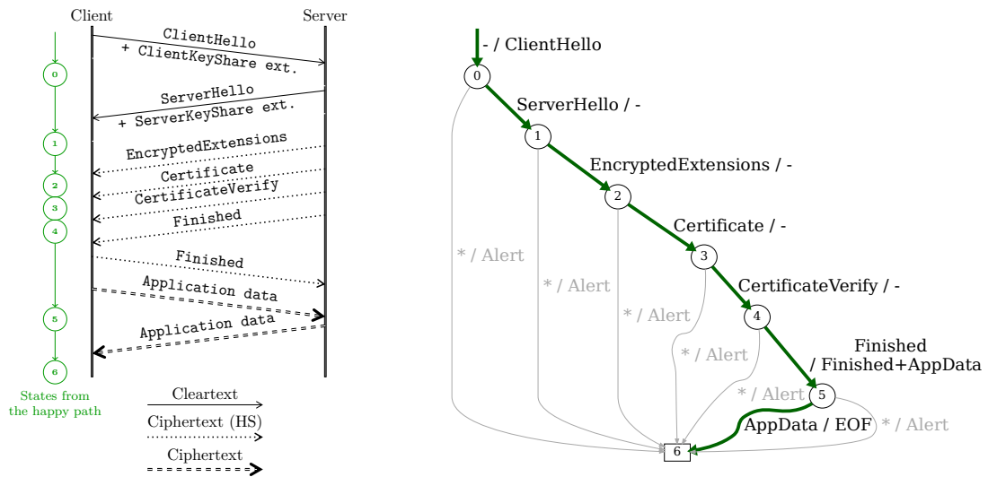
Figure 5.1: A typical TLS 1.3 connection and the corresponding expected client state machine.
