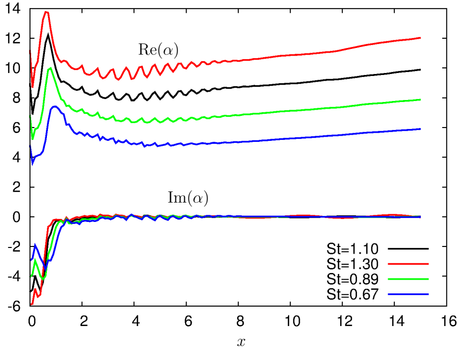
Figure 2.22: Axial distribution of the streamwise wave-number \alpha for different values of the Strouhal number, respectively 1.10, 1.30, 0.89, 0.67
