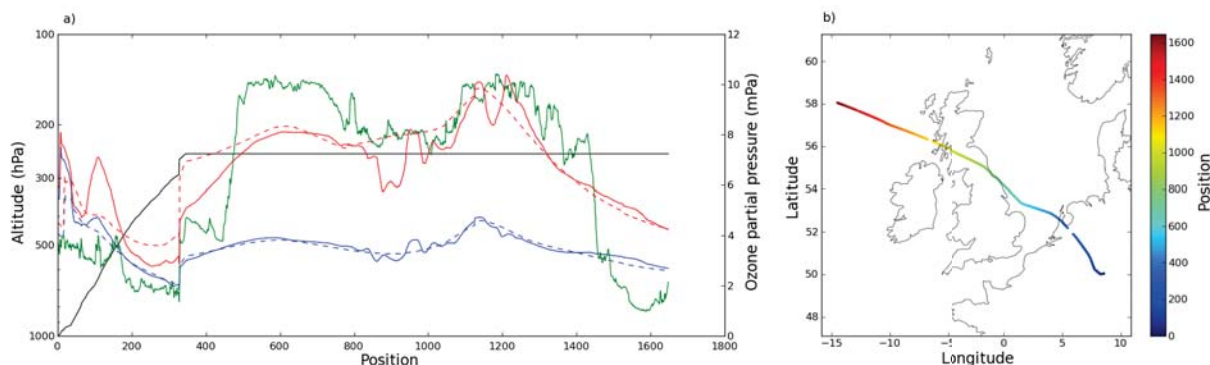
FIGURE 3.9 – Left hand side panel : ozone data from MOZAIC (green line), free MOCAGE run (blue lines) and analyses fields (red lines), units of mPa (right hand side y-axis); flight level (black line), units of hPa (left hand side y-axis). Low resolution ( 2^\circ ) and high resolution ( 0.2^\circ ) results are marked as dashed lines and solid lines, respectively. Right hand side panel : flight track on 17 July 2009. Position 0 to 1700 : starting at Frankfurt ( 50^\circ N, 8^\circ E, Germany, 11 :57 UT) to Atlanta ( 33^\circ N, 84^\circ , US).
