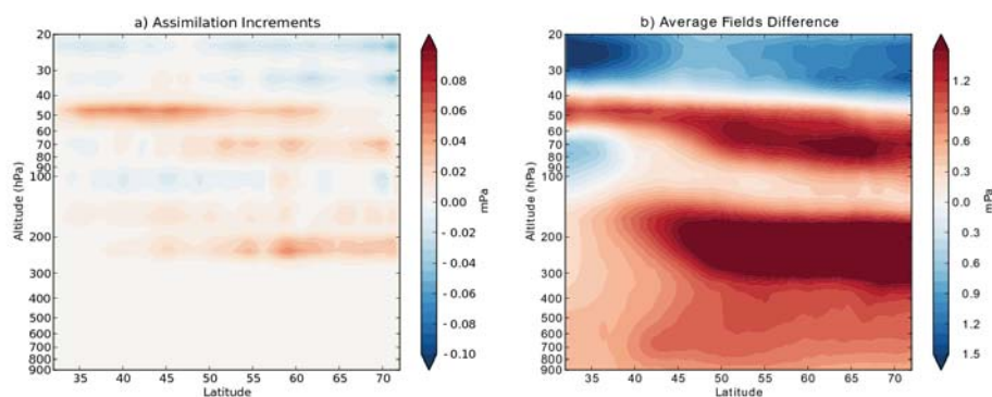
FIGURE 4.4 – (a) Zonal mean of increments of the MLS ozone analyses in partial pressure (mPa); (b) Zonal mean of the MLS ozone analyses minus the MOCAGE free run in mPa. Zonal means are performed for the month of July 2009 over Europe (longitudes from 15°W to 35°E).
