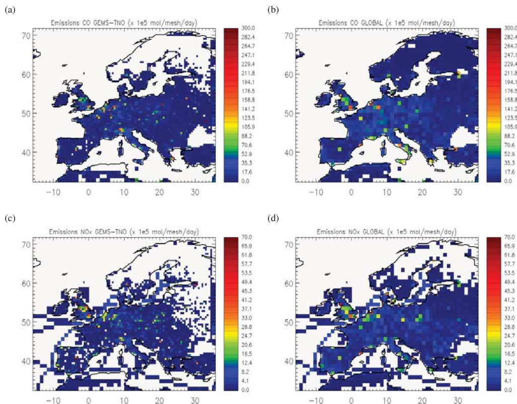
Fig. 1. Total CO emitted by day and by model mesh ( 0.5^\circ ) over Europe on 6 July 2009 with GEMS-TNO emission inventory (a) and global emission inventory (b). (c) and (d) are as (a) and (b) but for \text{NO}_x = \text{NO} + \text{NO}_2 .
