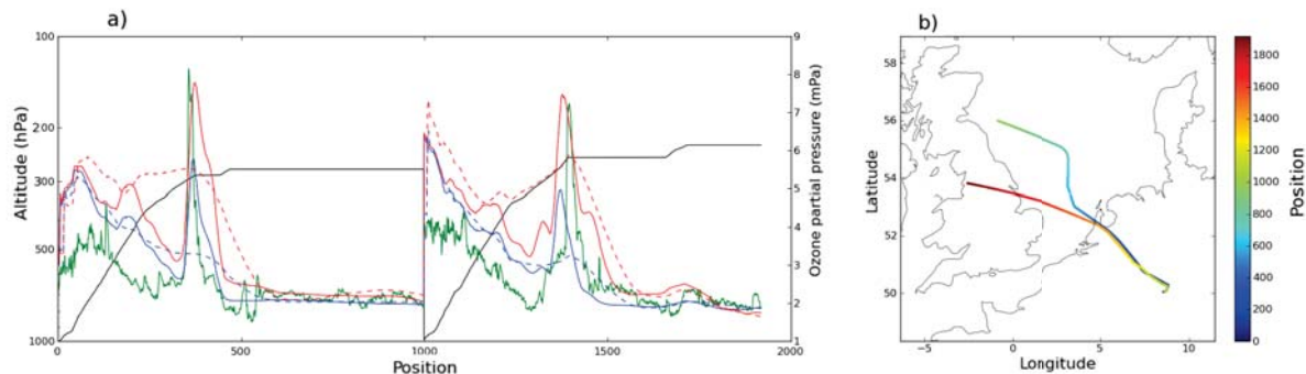
FIGURE 3.5 – Left hand side panel : ozone data from MOZAIC (green line), free MOCAGE run (blue lines) and analyses fields (red lines), in mPa ( 10^{-3} Pascals, right hand side y-axis); flight level (black line), in hPa ( 10^2 Pascals, left hand side y-axis). Low resolution ( 2^\circ ) and high resolution ( 0.2^\circ ) results are marked as dashed lines and solid lines, respectively. Right hand side panel : flight tracks on 23 June 2009. Position 0 to 1000 : starting at Frankfurt ( 50^\circ N, 8^\circ E, Germany, 08 :13 UT) to Calgary ( 51^\circ N, 114^\circ W, Canada). Position 1000 to 1900 : starting at Frankfurt ( 50^\circ N, 8^\circ E, Germany, 13 :00 UT) to Philadelphia ( 39^\circ N, 75^\circ W, US).
