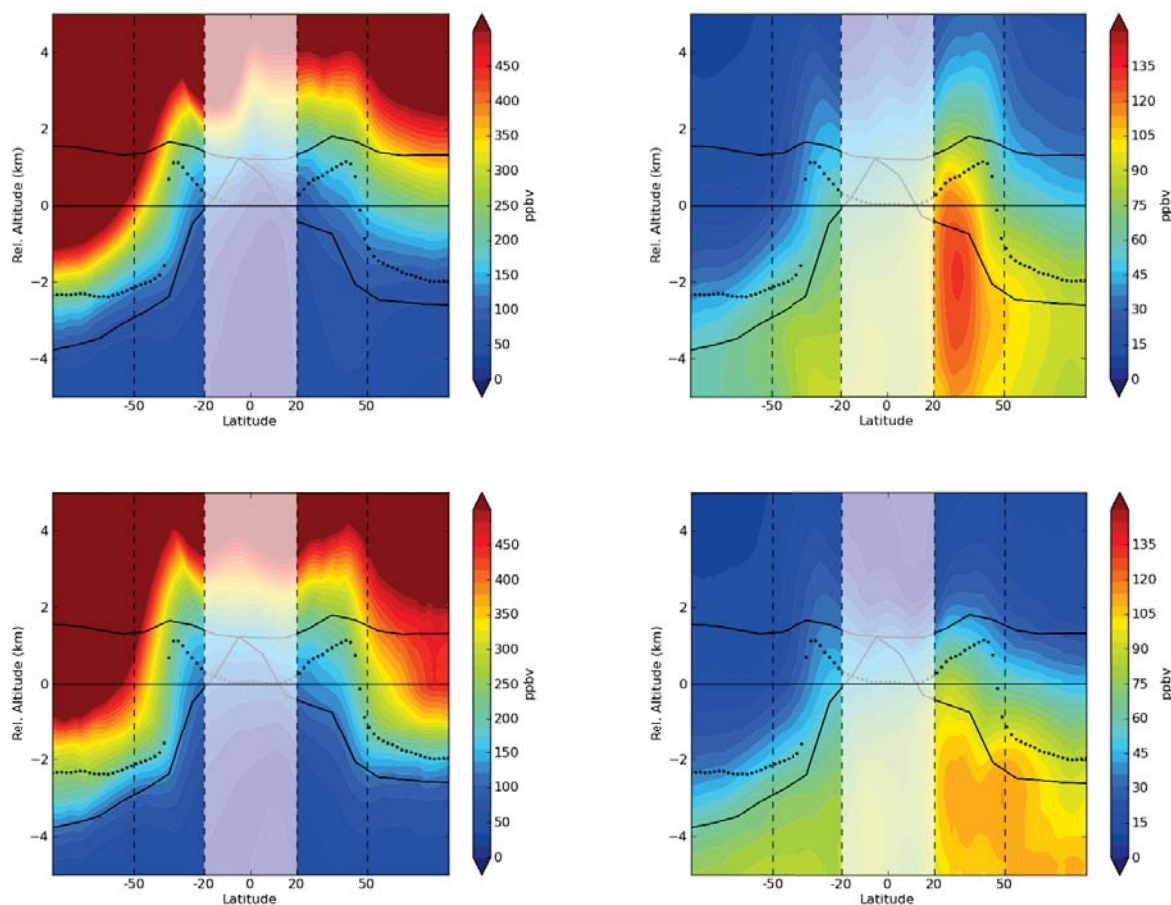
FIGURE 5.6 – Zonal averages for the month of August 2007 in relative altitudes (km) of model O 3 (a), model CO (b), O 3 analyses (c) and CO analyses (d). Dashed black vertical lines mark the regions of interest. The lowermost stratosphere bounds are represented by the 2-PVU contour in absolute value (lower black line), and the 380-K isentrope (upper black line). Black dots are the thermal tropopause relative altitudes. Tropical latitudes are not shown.
