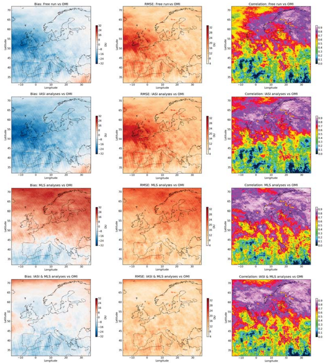
FIGURE 4.12 – Detailed statistics in each grid point for the month of July 2009. Top to bottom : Free model Run (Free-R), IASI analyses Run (IASI-R), MLS analyses Run (MLS-R), IASI and MLS combined analyses Run (Combined-R). Left to right : biases; Root Mean Square Error (RMSE); correlation coefficient ( R^2 ). Biases and RMSE are in Dobson Units (DU).
