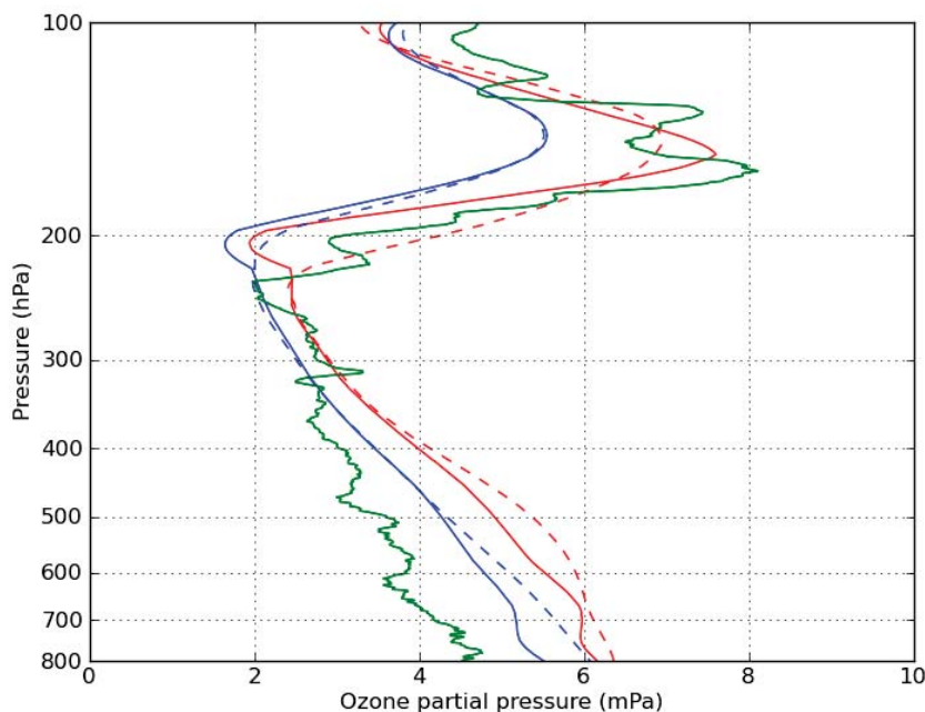
FIGURE 3.6 – Ozone profiles in mPa from a sonde over Legionowo (52.4° N, 21.97° E, Poland; green line, launched at 11 :17 UT on 24 June 2009), from the free MOCAGE run (blue lines) and from analyses (red lines). Low resolution (2°) and high resolution (0.2°) results are represented by dashed and solid lines, respectively.
