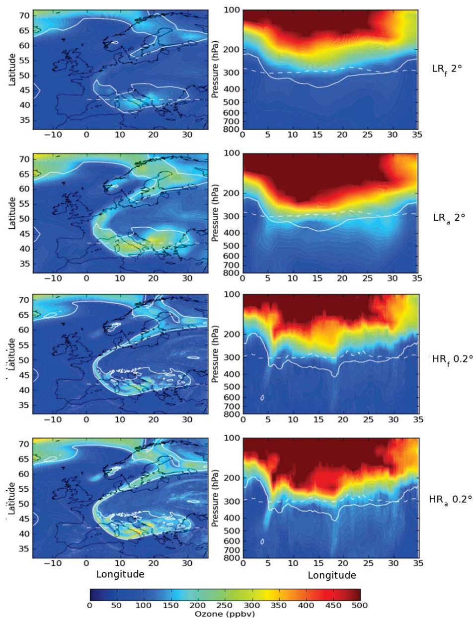
FIGURE 3.4 – Ozone fields for 23 June 2009, 12 :00 UT, in ppbv (parts per billion by volume) for various experiments : LR_f : Low Resolution ( 2^\circ ) free run ; LR_a : Low Resolution ( 2^\circ ) analyses ; HR_f : High Resolution ( 0.2^\circ ) free run and HR_a : High Resolution ( 0.2^\circ ) analyses. Left hand side panels show longitude-latitude fields for a given model level ; right hand side panels show longitude-pressure cross-sections. White dashed line associate vertical and horizontal distribution by showing the same location between left hand side and right hand side panels. The white solid lines identify the 2 PVU contour.
