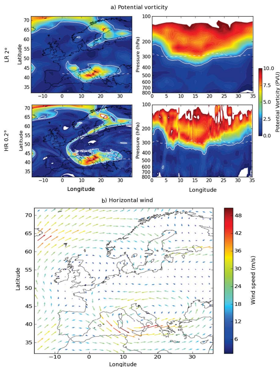
FIGURE 3.3 – Meteorological situation on 23 June 2009, 12 :00 UT from ARPEGE analysis. (a) Potential vorticity fields, in potential vorticity units ( 1\text{PVU} = 1 \times 10^6 \text{K kg}^{-1} \text{m}^2 \text{s}^{-1} ) from low ( 2^\circ ) horizontal resolution simulation (top) and high horizontal resolution ( 0.2^\circ ) simulation (bottom). Left hand side panels show longitude-latitude fields for a given model level ; right hand side panels show longitude-pressure cross-sections. The white dashed line associates the vertical and the horizontal distribution by showing the same location between left hand side and right hand side panels. The white solid lines identify the 2PVU contour. (b) Horizontal wind fields at LR near 300 hPa.
