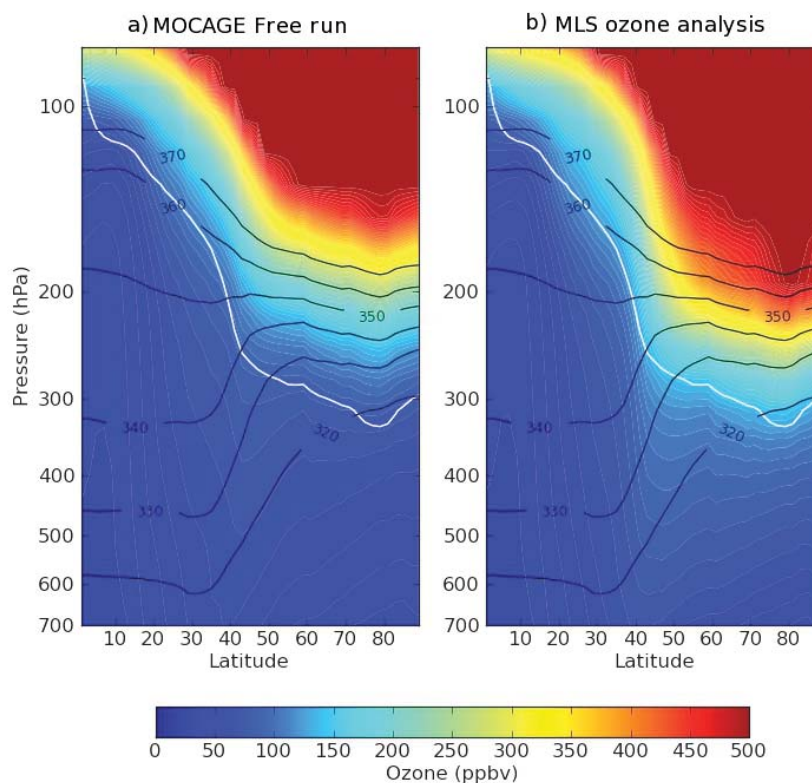
FIGURE 3.2 – Zonal means of ozone for the month of July 2009 in Northern Hemisphere (low resolution runs 2^\circ ). (a) MOCAGE free run, (b) MLS ozone analysis. Black lines are the potential temperature, the white line represents the 2 PVU iso-line (an estimate of the tropopause height).
