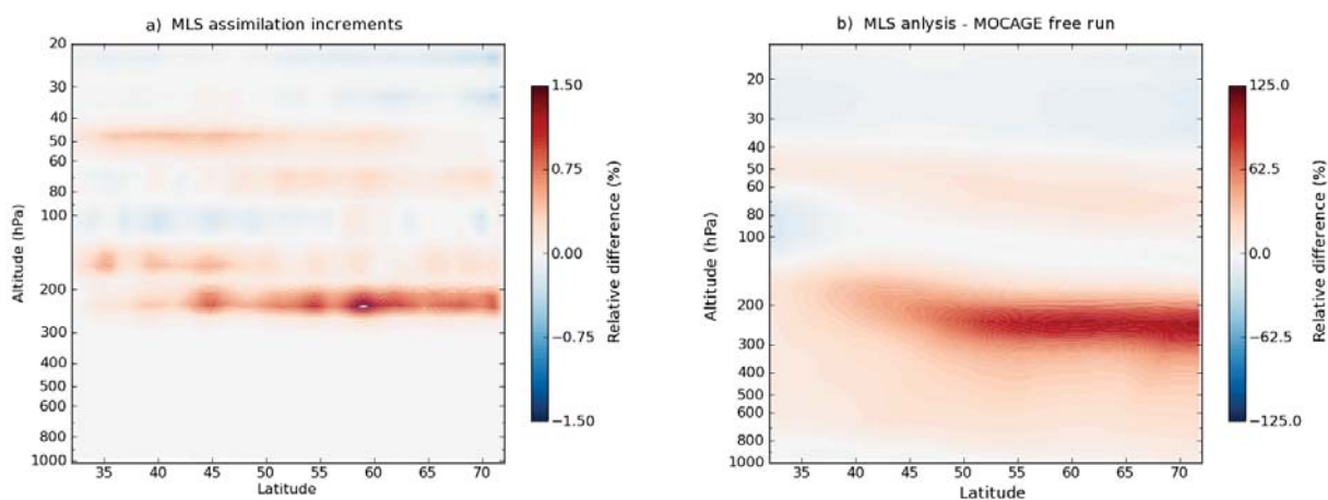
FIGURE 3.1 – (a) Zonal means of increments of MLS ozone analyses at high horizontal resolution ( 0.2^\circ ) in relative difference in %; (b) Zonal means of the MLS ozone analysis minus the associated equivalent MOCAGE free run at high horizontal resolution ( 0.2^\circ ) in relative difference in %. Zonal means are performed for the month of July 2009 over Europe.
