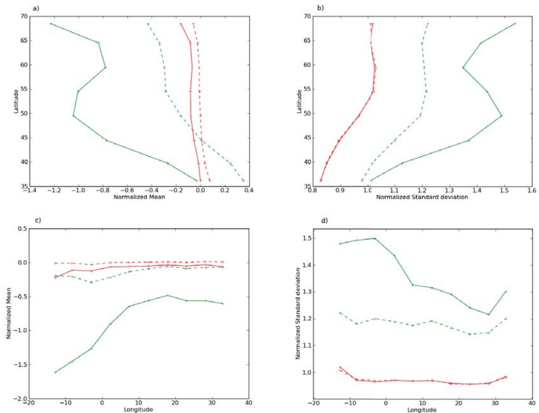
FIGURE 4.8 – Latitudinal and longitudinal variations of the mean ((a) and (c) respectively) of observations minus forecasts (OMF, green) and observations minus analyses (OMA, red) normalized by the observations errors concerning assimilated IASI O_3 . Latitudinal and longitudinal variations of the standard deviation ((b) and (d) respectively) of OMF (green) and OMA (red). Dashed lines represent the OMA, OMF of IASI or MLS single analyses and solid lines represent the OMA, OMF of IASI and MLS combined analyses. The diagnostics are performed for the month of July 2009 over Europe.
