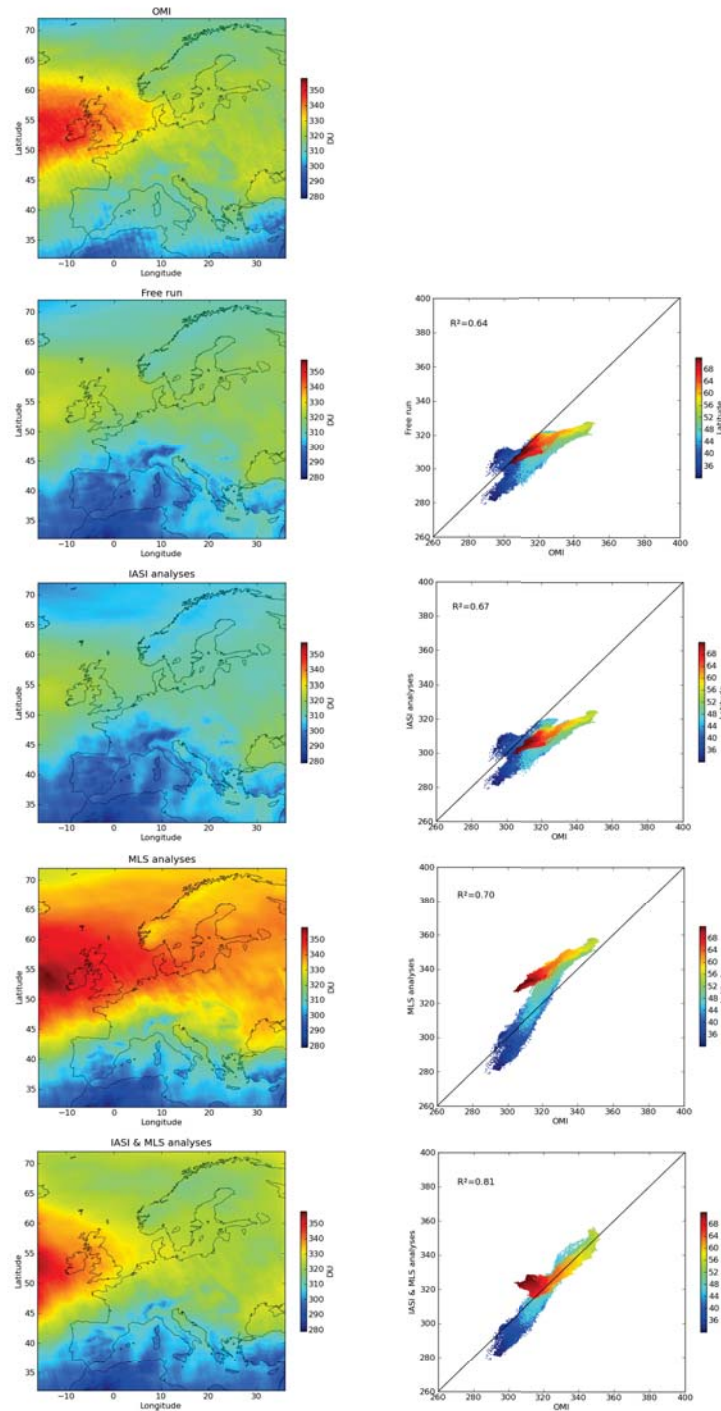
FIGURE 4.11 – Left hand side, top to bottom : ozone total column fields in Dobson Unit (DU) averaged on the month of July 2009 for OMI observations, Free model Run (Free-R), IASI analyses Run (IASI-R), MLS analyses Run (MLS-R), IASI and MLS Dual analyses Run (Combined-R). Right hand side : corresponding scatter plots of the assimilation experiments versus OMI observations with correlation coefficients ( R , R^2 ). Color of dots denotes the location in latitude.
