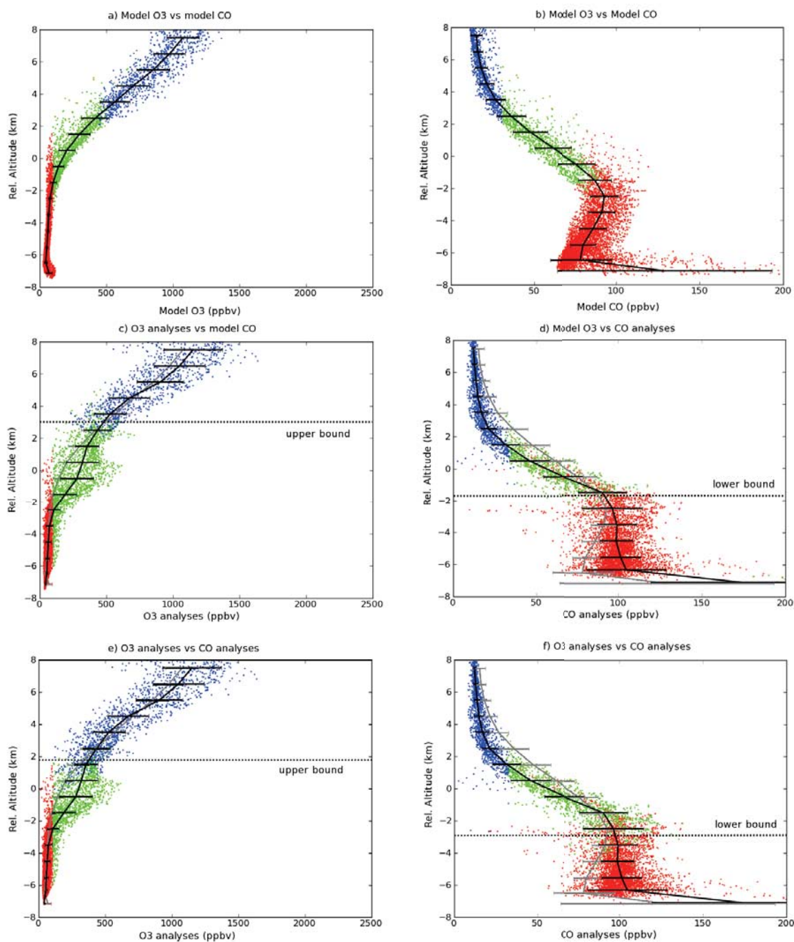
FIGURE 5.4 – O 3 and CO profiles in the region between 30°W - 10°E, 40°N - 65°N on 15 August 2007 at 12 :00 UT. O 3 profiles (ppbv) in altitude coordinates (km) relative to the 360-K level are provided for model O 3 vs model CO (a) , O 3 analyses vs model CO (c) and O 3 analyses vs CO analyses (e) . CO profiles (ppbv) in relative altitude coordinates (km) are provided for model O 3 vs model CO (b) , model O 3 vs CO analyses (d) and O 3 analyses vs CO analyses (f) . Following selection criteria, red and blue dots are identified as of tropospheric and stratospheric origin, respectively. The green dots are identified as the transitional layer between the stratosphere and the troposphere (see text for details). Black lines represent the mean profile every kilometer and horizontal error bars show the 1 \sigma standard deviation. Over-plotted gray lines and gray error bars (c-f) are the free model run mean and standard deviation values for O 3 and CO, respectively.
