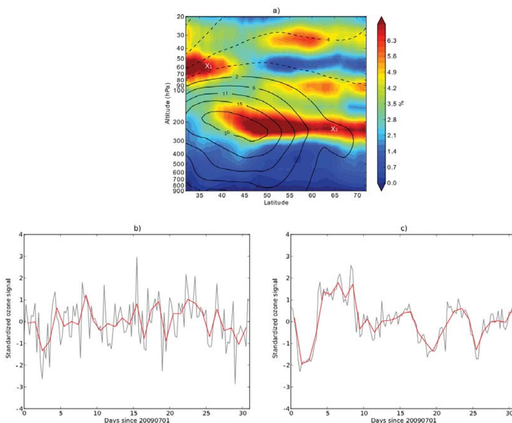
FIGURE 4.13 – (a) Zonal mean of the variability contribution of the total ozone column (see text for details) for the month of July 2009. Mean zonal winds are over-plotted in black, Eastward values are in solid lines and Westward values are in dashed lines. With X_1 and X_2 indicate the locations of the times series displayed in (b) and (c), respectively. (b) Time series located in 37^\circ\text{N} , 10^\circ\text{W} and 60 hPa : gray line is 6 hourly values and red line is daily values. (c) Time series located in 65^\circ\text{N} , 10^\circ\text{W} and 220 hPa : gray line is 6 hourly values and red line is daily values.
