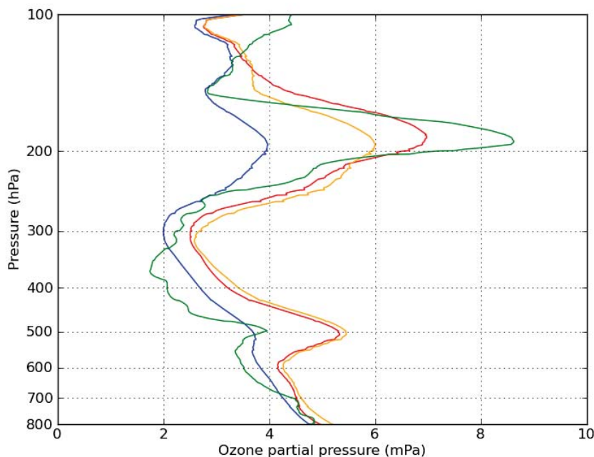
FIGURE 3.12 – Ozone profiles, mPa, from a sonde over Payerne ( 46.5^{\circ} N, 6.6^{\circ} E; green line, launched at 11 :00 UT on 17 July 2009), from the free MOCAGE run (blue line), from analyses (red line) and forecasted run initialised with MLS analyses at 00 :00 UT on 15 July 2009 (orange line). All experiments are from High Resolution ( 0.2^{\circ} ) runs.
