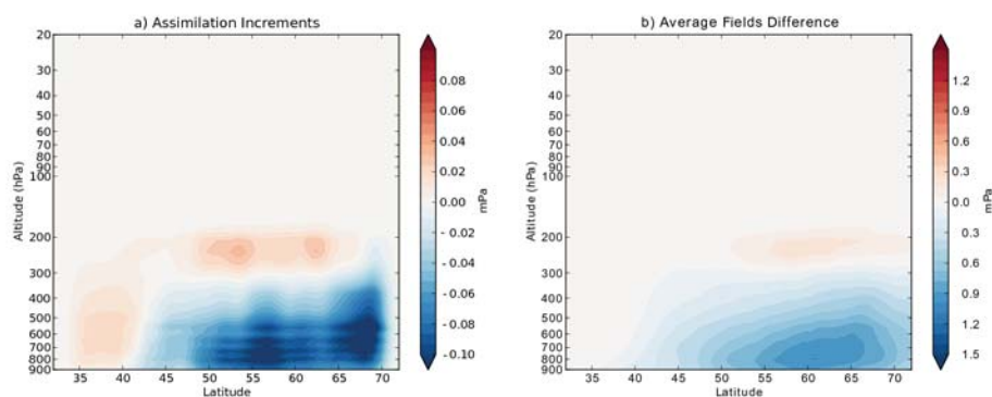
FIGURE 4.3 – (a) Zonal mean of the increments of the IASI ozone analyses in partial pressure (mPa); (b) Zonal mean of the IASI ozone analysis minus the MOCAGE free run in mPa. Zonal means are performed for the month of July 2009 over Europe (longitudes from 15°W to 35°E).
