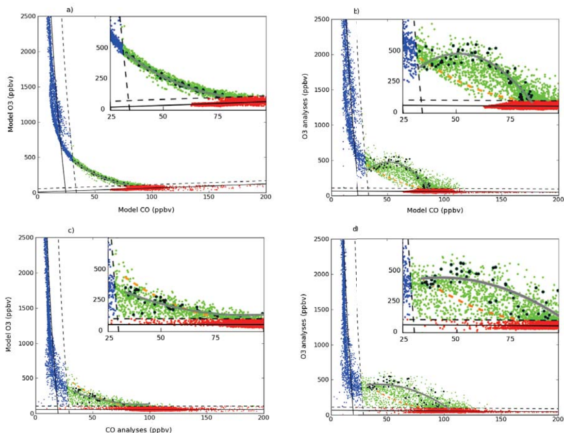
FIGURE 5.3 – Comparisons of the O 3 -CO relationships between model O 3 vs model CO (a), O 3 analyses vs model CO (b), model O 3 vs CO analyses (c) and O 3 analyses vs CO analyses (d) in the area between 30°W - 10°E, 40°N - 65°N on 15 August 2007 at 12 :00 UT. In all cases, red and blue dots are identified as tropospheric and stratospheric model grid points, respectively. Black solid lines indicate fits to tropospheric and stratospheric values and the dashed lines are the +3 \sigma values (where \sigma is the standard deviation of the selected data) from those fits. The green dots are identified as the transition between stratospheric and tropospheric air. The transitional points between 20°W and 0°W on the 59°N vertical plane are in black and are fitted by the gray line. The model O 3 vs model CO fit is over-plotted on (b-d) in dashed orange (see text for details). Within each plot box a zoom of the transition region is provided (top-right) on each panel.
