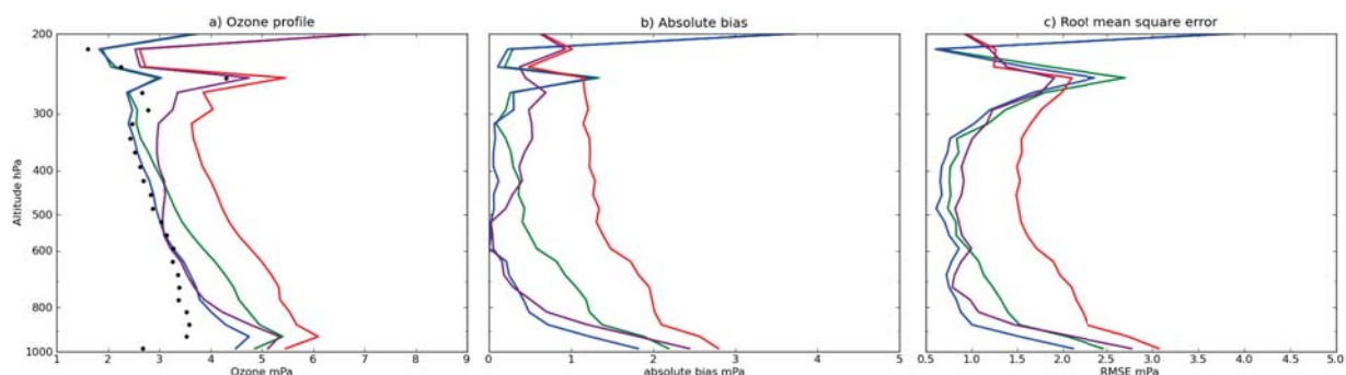
FIGURE 4.10 – (a) Comparisons between the averaged vertical profile of IAGOS aircraft (black dots) and averaged assimilation experiments profiles : green : Free model run (Free-R), blue : IASI analyses (IASI-R), red : MLS analyses (MLS-R), purple : combined MLS and IASI analyses Run (Combined-R). 75 profiles are averaged. (b) Absolute bias between IAGOS and assimilation experiments : green Free-R, blue IASI-R, red MLS-R, purple Combined-R. (c) Root mean square error between IAGOS and assimilation experiments : green Free-R, blue IASI-R, red MLS-R, purple Combined-R. Values are in partial pressure (mPa).
