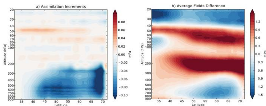
FIGURE 4.5 – (a) Zonal means of increments of MLS plus IASI combined ozone analyses in partial pressure (mPa); (b) Zonal means of the MLS plus IASI ozone analyses minus the MOCAGE free run in mPa. Zonal means are performed for the month of July 2009 over Europe (longitudes from 15°W to 35°E).
