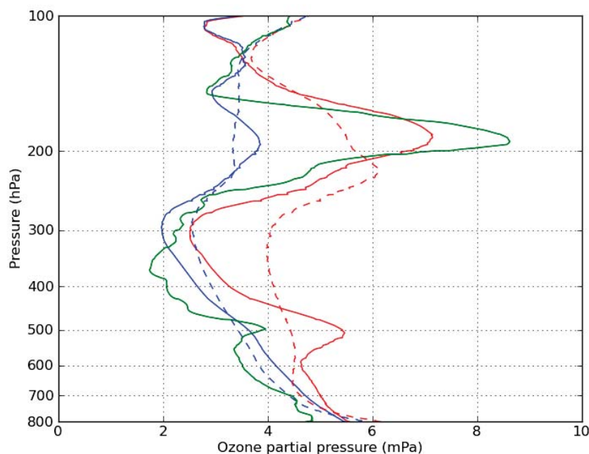
FIGURE 3.10 – Ozone profiles, mPa, from a sonde over Payerne ( 46.5^{\circ} N, 6.6^{\circ} E; green line, launched at 11 :00 UT on 17 July 2009), from the free MOCAGE run (blue lines) and from analyses (red lines). Low resolution ( 2^{\circ} ) and high resolution ( 0.2^{\circ} ) results are represented by dashed and solid lines, respectively.
