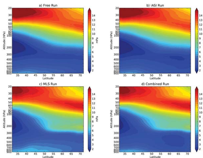
FIGURE 4.1 – Zonal mean of the ozone field (mPa) of the free model run (a), the IASI analyses (b), the MLS analyses (c) and the Combined IASI and MLS analyses (d) for the month of July 2009 over Europe (longitudes from 15°W to 35°E).
