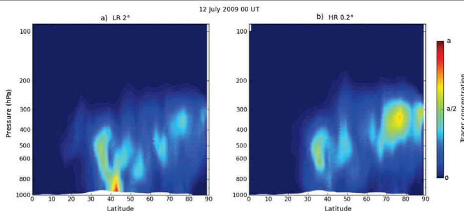
FIGURE 3.11 – Zonal means of a tracer initialised backward trajectories. (a) Low Resolution (LR 2^\circ ), (b) High Resolution (HR 0.2^\circ ). Tracer concentration values are arbitrary : from 0 to a (the maximum value).
