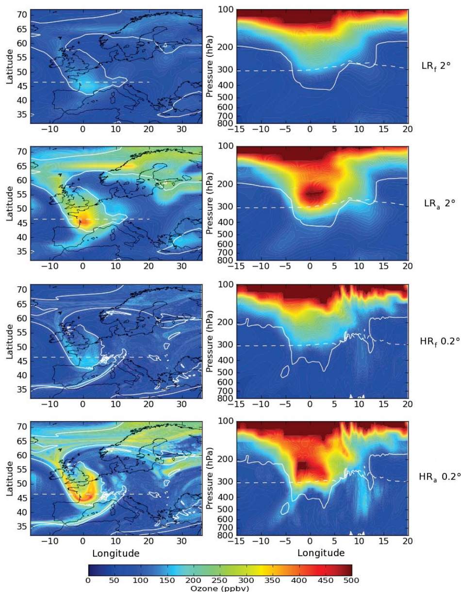
FIGURE 3.8 – Ozone fields for 17 July 2009, 15 :00 UT, in ppbv (parts per billion by volume) for various experiments : LR_f : Low Resolution ( 2^\circ ) free run ; LR_a : Low Resolution ( 2^\circ ) analyses ; HR_f : High Resolution ( 0.2^\circ ) free run and HR_a : High Resolution ( 0.2^\circ ) analyses. Left hand side panels show longitude-latitude fields for a given model level ; right hand side panels show longitude-pressure cross-sections. White dashed line associate vertical and horizontal distribution by showing the same location between left hand side and right hand side panels. The white solid lines identify the 2 PVU contour.
