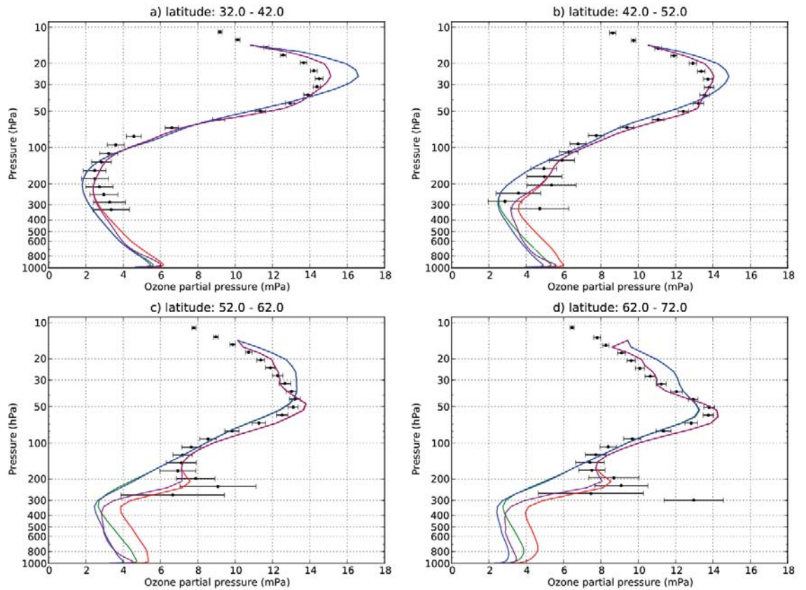
FIGURE 4.9 – Zonally averaged vertical profiles by 10^\circ of latitude for the month of July 2009 over Europe. Latitudes ranges from top to bottom and left to right : 32^\circ\text{N} to 72^\circ\text{N} by 10^\circ intervals ( a-d ). Black dots : MIPAS dataset, green : free model run (Free-R), blue : IASI analyses (IASI-R), red : MLS analyses (MLS-R), purple : combined MLS and IASI analyses (Combined-R). Values are in partial pressure (mPa). Error bars provide the averaged error of the MIPAS measurements.
