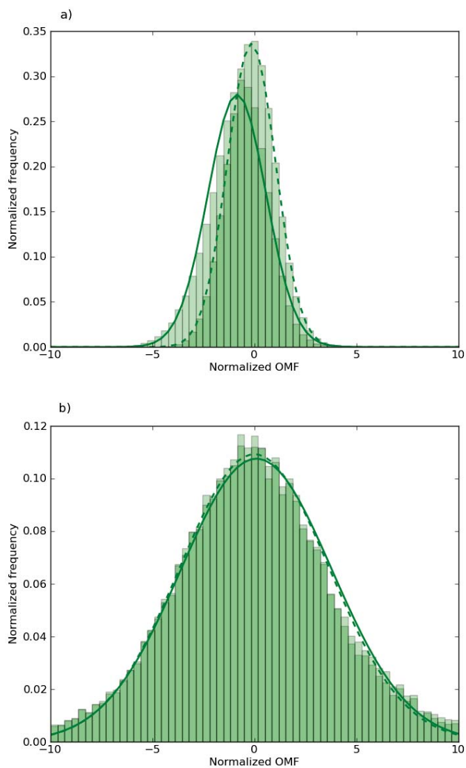
FIGURE 4.7 – Distributions of observations minus forecasts (OMF) normalized by the observations errors for assimilated IASI O 3 (a) and assimilated MLS O 3 (b). Dashed lines represent the Gaussian fit of OMF for IASI or MLS single analyses and solid lines represent the Gaussian fit for OMF of IASI and MLS combined analyses. The frequency values are normalized by the total number of observations. The diagnostics are performed for the month of July 2009 over Europe.
