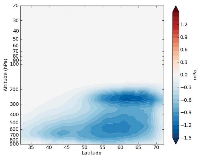
FIGURE 4.6 – Zonal means of [\text{Combined-R}] + [\text{Free-R}] - [\text{IASI-R}] - [\text{MLS-R}] in mPa. Zonal means are performed for the month of July 2009 over Europe (longitudes from 15^{\circ}\text{W} to 35^{\circ}\text{E} ).
