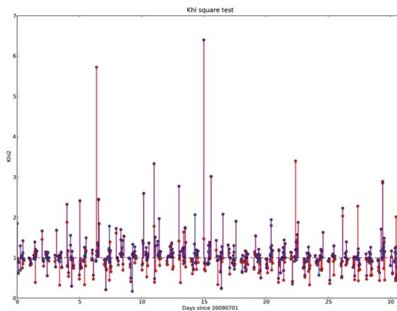
FIGURE 4.2 – Plots of \chi^2 as a function of time for the month of July 2009 over Europe. Each value is calculated for one assimilation window (1 hour) for IASI O 3 analyses (red), MLS O 3 analyses (blue) and combined MLS and IASI O 3 analyses (purple) over Europe (see text for a discussion of this test). \chi^2 values are omitted when no IASI or MLS data are available.
