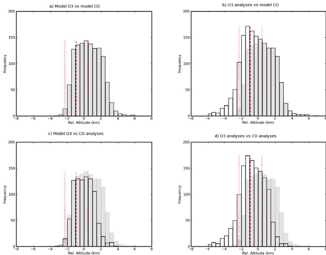
FIGURE 5.5 – Histograms showing the distributions of the ExTL in relative altitude space in the region between 30°W - 10°E, 40°N - 65°N on 15 August 2007 at 12 :00 UT. model O 3 vs model CO (a) , O 3 analyses vs model CO (b) , model O 3 vs CO analyses (c) and O 3 analyses vs CO analyses (d) are displayed in black and model O 3 vs model CO distribution is over-plotted in gray on the plots. Red dashed and dotted vertical lines line show the mean and the standard deviation of the location of the thermal tropopause, respectively. The histograms display the absolute frequencies.
