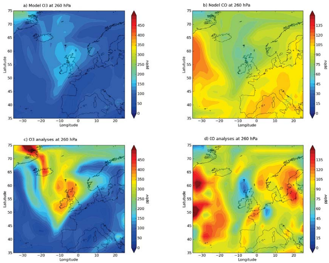
FIGURE 5.1 – Longitude-latitude maps at 260 hPa of model O 3 (a), model CO (b), O 3 analyses (c) and CO analyses (d) for 15 August 2007 at 12 :00 UT
