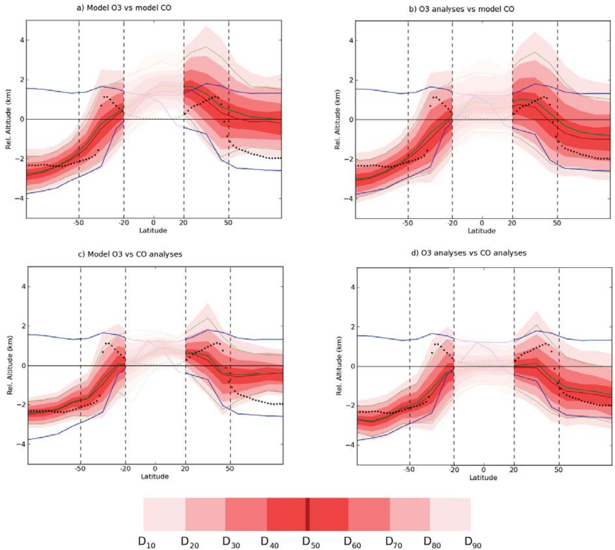
FIGURE 5.7 – Latitudinal height variations in altitude coordinates (km) relative to the 360-K level of the ExTL distribution for model O 3 vs model CO (a), O 3 analyses vs model CO (b), model O 3 vs CO analyses (c) and O 3 analyses vs CO analyses (d) in August 2007. Red filled contours provide the decile altitudes of the distribution. Red and green lines are the median and mean altitudes, respectively. Blue lines show the lowermost stratosphere bounds : the lower line provides the 2-PVU contour in absolute value, the upper line provides the 380-K isentropic contour. Black dots show the location of the thermal tropopause. Tropical latitudes are not shown.
