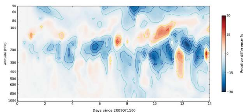
FIGURE 3.13 – Hovmuller diagram of the profile : (Forecast-MLS ozone analyses) in %, averaged between 44° N–48° N and 5° W–9° W (Switzerland). Forecast is initialised from MLS ozone analyses on 15 July 2009 00 :00 UT.
