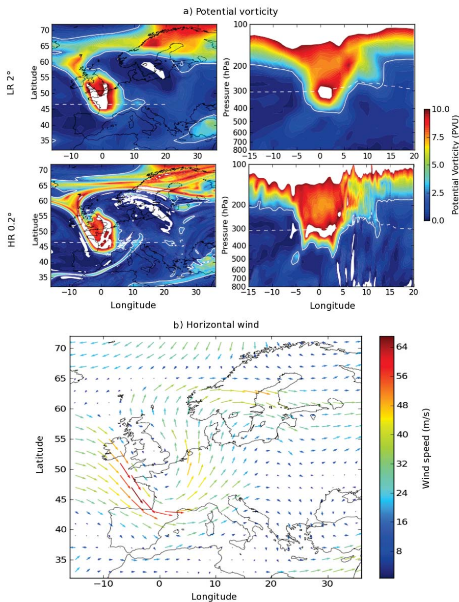
FIGURE 3.7 – Meteorological situation on 17 July 2009, 15 :00 UT from ARPEGE analysis. (a) Potential vorticity fields, in potential vorticity unit ( 1 \text{ PVU} = 1 \times 10^6 \text{ K kg}^{-1} \text{ m}^2 \text{ s}^{-1} ) from low horizontal resolution ( 2^\circ ) simulation (top) and high horizontal resolution ( 0.2^\circ ) simulation (bottom). Left hand side panels show longitude-latitude fields for a given model level; right hand side panels show longitude-pressure cross-sections. The white dashed line associates the vertical and the horizontal distribution by showing the same location between left hand side and right hand side panels. The white solid lines identify the 2 PVU contour. (b) Horizontal wind fields at LR near 300 hPa.
