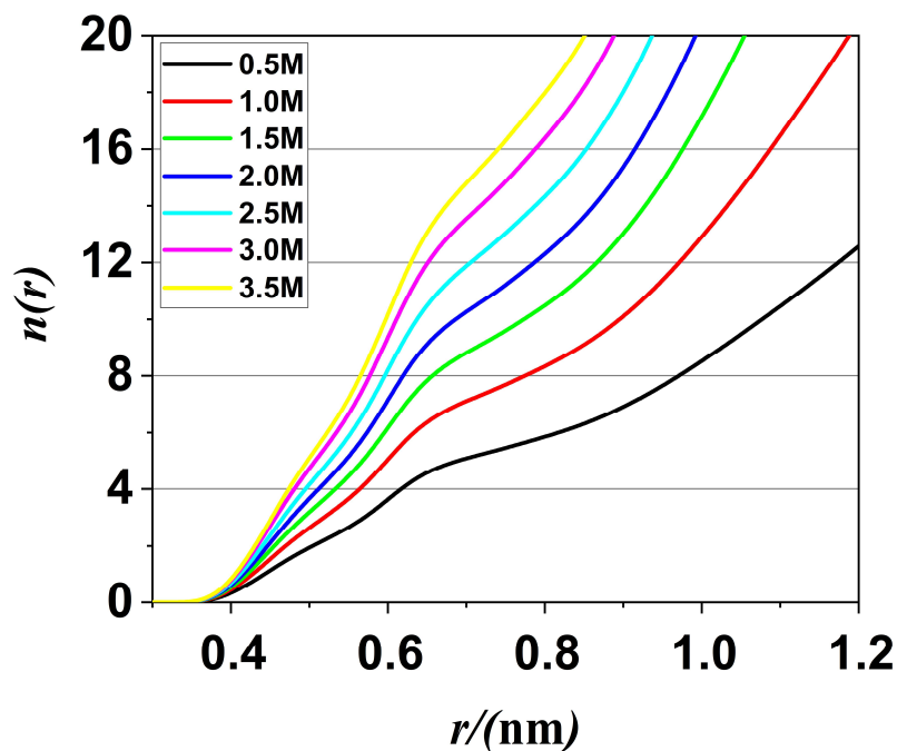
Figure 2.2. Example of cation-anion (N-F) running coordination numbers at various molar concentrations of SBPBF 4 in AN mixture.
