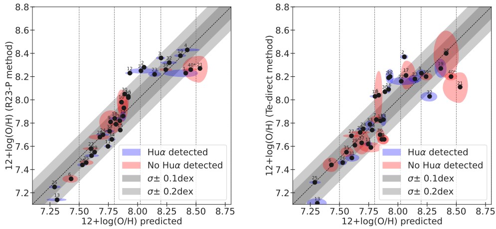
Figure 8.5: Left: Predicted metallicity as compared to metallicity estimate from the R23-P method (Pilyugin & Thuan 2005). No measurements are available for 4 galaxies (HS0017+1055, HS0052+2536, HS2352+2733 and Mrk1089). Right: Predicted metallicity as compared to metallicity estimate from the T_e -direct method (Izotov et al. 2006). No measurements are available for 2 galaxies (Haro11 and He2-10). The 1\sigma contours of the SUEs are calculated with a dispersion corresponding to the measured uncertainty for the y-axis.
