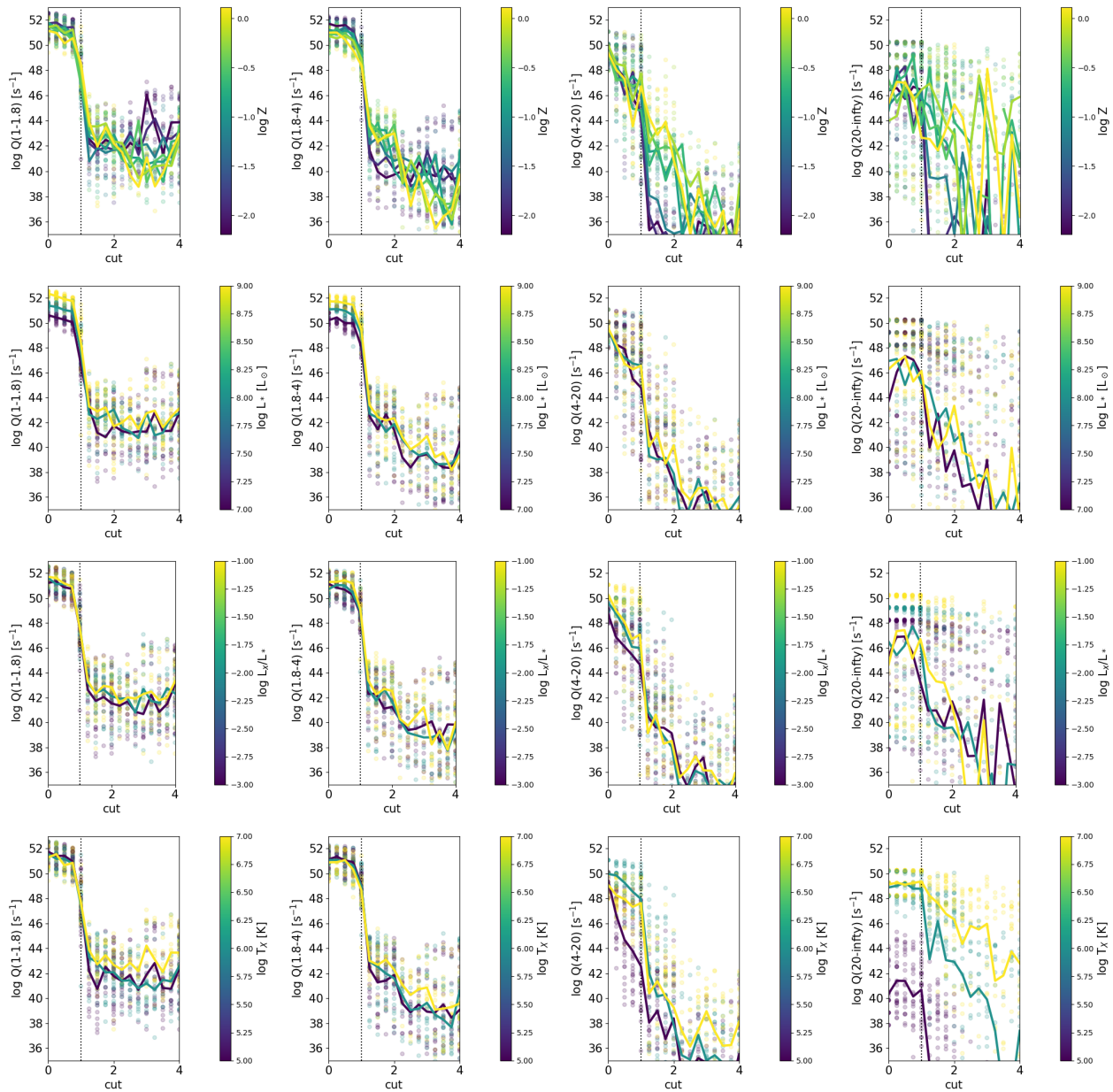
Figure 9.7: Q vs. \text{cut} relation in different energy ranges: 1-1.8 Ryd (1 st column), 1.8-4 Ryd (2 nd column), 4-20 Ryd (3 rd column), and 20- \infty Ryd (4 th column).
