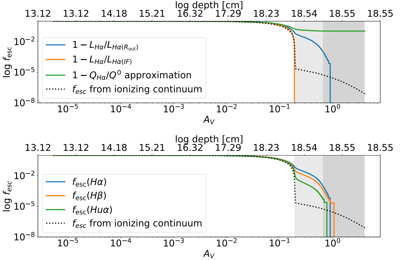
Figure 9.3: Comparison of different proxies to estimate f_{\text{esc}} . Top: Evolution of f_{\text{esc}} vs. A_V for different proxies. The tests are run for a solar-metallicity model, without any X-ray source, and run up to N_{\text{H}}=10^{22} \text{ cm}^{-3} . The shaded areas mark the PDR location (light-gray) and the \text{H}_2 molecular zone (dark-gray). Bottom: Comparison of the escape fractions estimated from different hydrogen recombination lines: \text{H}\alpha , \text{H}\beta and \text{H}\alpha .
