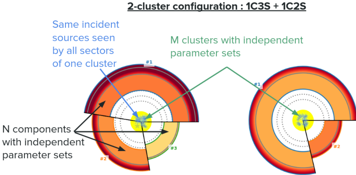
Figure 4.2: Multicenter, multisector representative topology with the same representation as in Figure 4.1.
