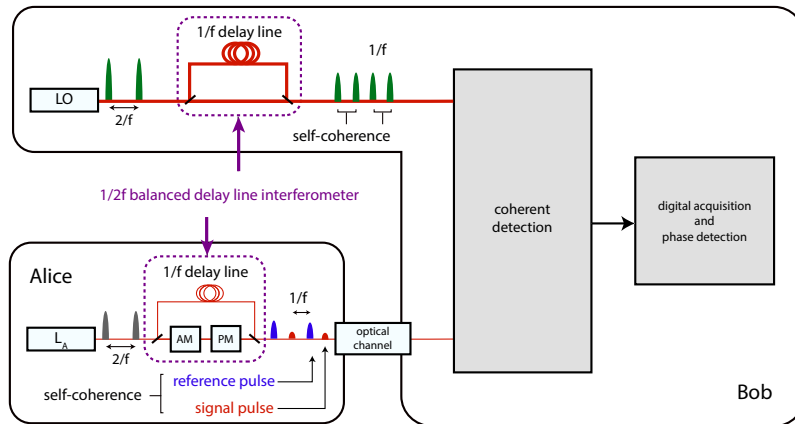
Figure 3.3: (color) LLO-delayline design. Alice sends consecutive phase coherent signal/reference pulses pairs to Bob based on a balanced delay line interferometer. On his side, Bob uses his own laser as the LO for coherent detections using the same delay line technique to produce phase coherent LO pulses. Phase estimation and phase correction are digitally performed after measurement acquisition.
