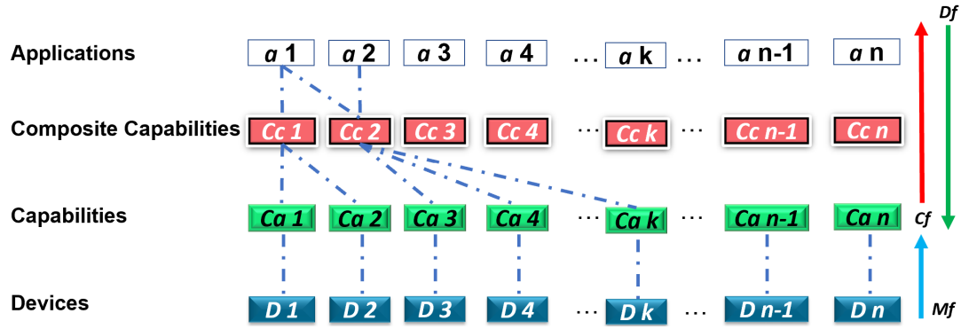
FIGURE 2.2: Modeling, composition, and decomposition layers and functions
