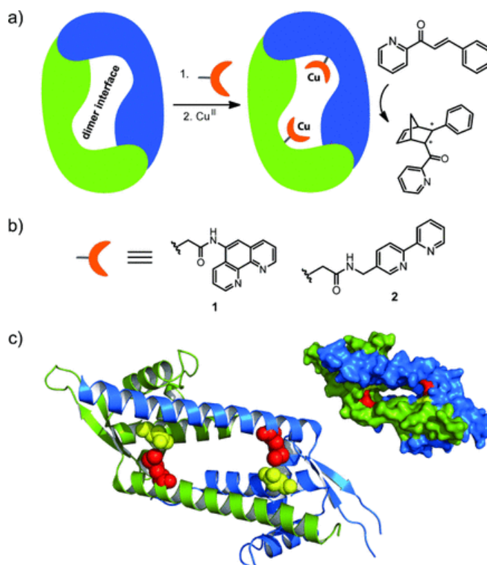
Figure 11: a) Schematic representation of the proposed artificial metalloenzyme in which a Cu II complex is grafted on the dimer interface of a protein. b) Ligands used for grafting on the dimer interface. c) Pymol representations of dimeric LmrR in a ribbon and a space-filling model (protein data bank (pdb) code: 3F8B). Either position 89 (red) or 19 (yellow) were used for the covalent binding of ligand 1 or 2. From Bos et al. Angew. Chem. Int. Ed. 2012, 51, 7472–7475.
