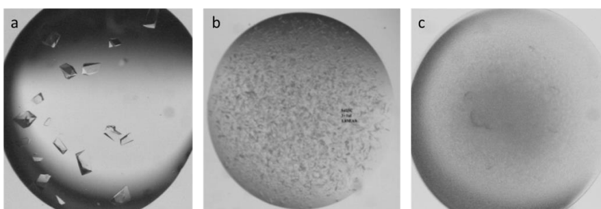
Figure 34: crystallization results at optimized conditions: (a)- Nika-WT at 160 \mu M with 1.5 M of AS (b)- Nika-S415C at 160 \mu M and 1.8 M of AS (c)-- Nika-A1C at 160 \mu M with 1.5M of AS (Ammonium sulfate)
