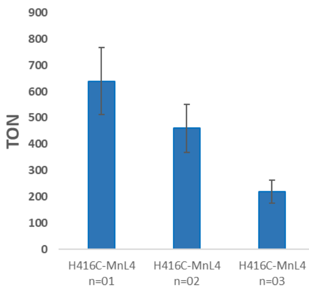
Figure 56: Evolution of the global TON on styrene epoxidation using CLEC H416C-MnL4 throughout three consecutive runs at room temperature. [cat] = 21 \mu M, H416C-MnL4/styrene/PAA of 1/2000/4000 for 16 h at r. t.
