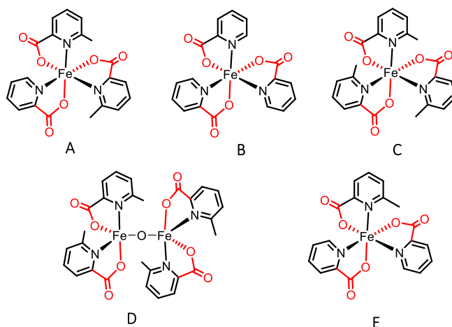
Figure 27: iron picolinate species used in this study
