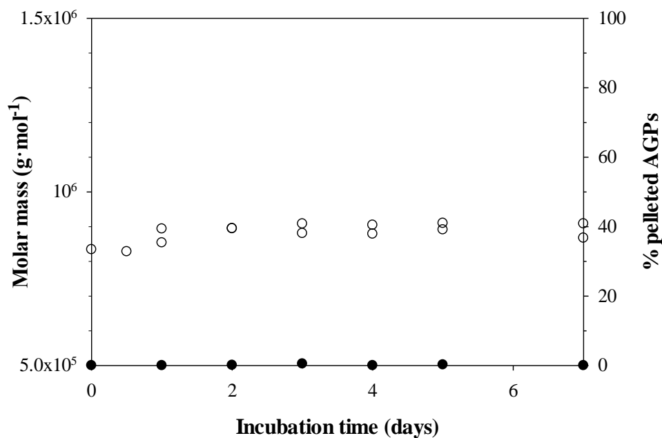
Figure III.12. Calculated mean molar mass ( \circ ) determined by SEC MALLS experiments from AGPs, and pelleted fraction ( \bullet ) of GA incubated between 0 and 7 days at 40°C.
