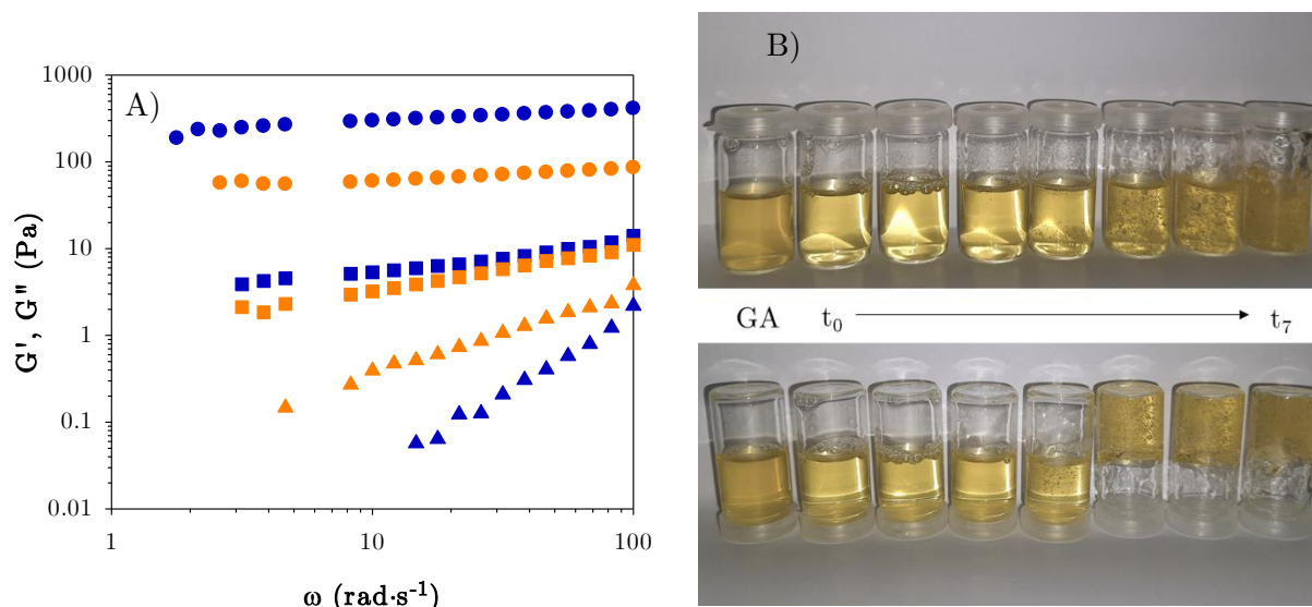
Figure VI.3. A) Storage G' (blue) and loss G'' (orange) moduli of 15wt% arabic acid powder dispersions at different incubation stages: before ( \blacktriangle ), and after incubation of powders for 2 days ( \blacksquare ), and 7 days ( \bullet ) at 40^\circ\text{C} . All experiments were performed at 1% strain. B) Visual observation of 15wt% aqueous dispersions of GA, arabic acid ( t_0 ) and arabic acid AGP aggregates (from left to right: t_1, t_2, t_3, t_4, t_5, t_7 ).
