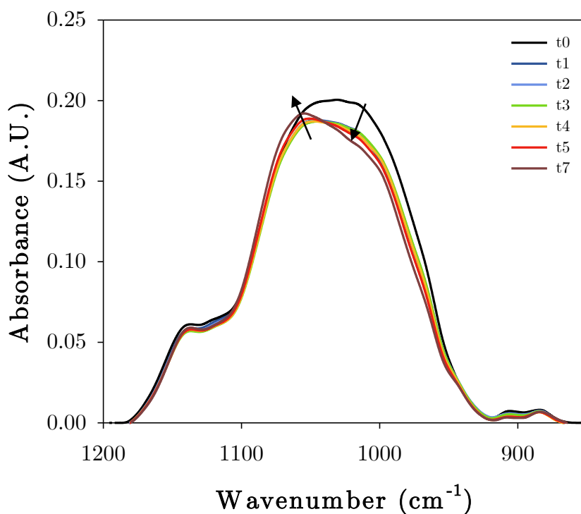
Figure V.10. Fourier transform infrared (FTIR) spectra of arabic acid and aggregated arabic acid samples in the spectral IR region from 850 to 1200 \text{ cm}^{-1} .
