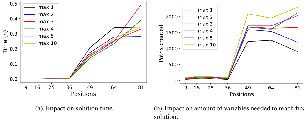
Figure 4.9: Analysis of the impact of changing the number of new variables (paths) added to the master problem per iteration of the column generation.
