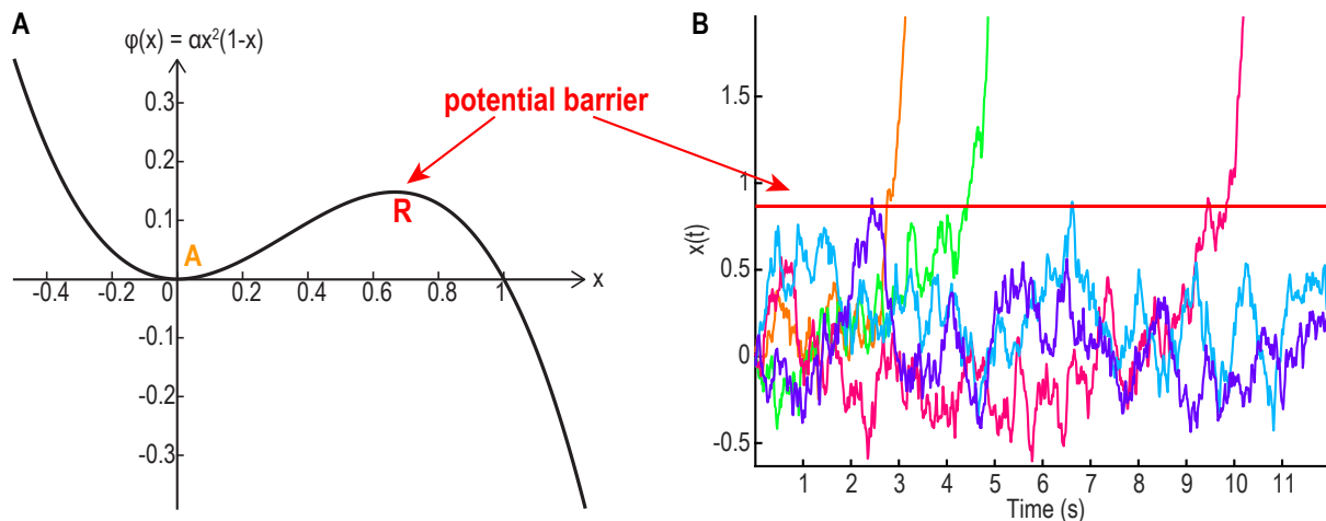
Figure 9: A. Potential well defined by the function \psi(x) = \alpha x^2(1-x) with one stable attractor A (yellow) and a repulsive equilibrium R (red) which defines the barrier of potential to cross to escape. B. Trajectories x(t) satisfying \dot{x} = -\frac{d\psi(x)}{dx} + \sigma\dot{w} where \dot{w} is a Gaussian white noise and \sigma its amplitude. The presence of noise can induce escape from the basin of attraction of A when the trajectories reach the boundary of the basin of attraction (red line).
