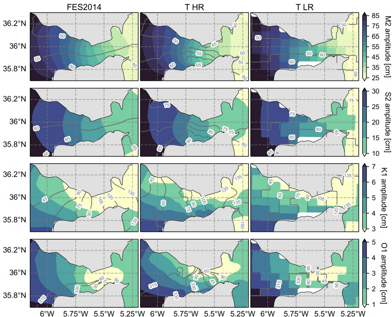
Figure 4.3: In shades from top to bottom, M2, S2, K1 and O1 tidal harmonics elevation amplitudes. We display in contours the associated phases. From left to right, we represent the global tidal atlas FES2014, the high-resolution and low-resolution tidal NEMOMEDGIB simulations. For NEMO simulations, tidal amplitudes and phases are estimated from hourly outputs of instantaneous (not averaged) sea level elevation over 2013 using the “Utide” Python package (version 0.2.5). FES2014 fields are interpolated on the high-resolution model grid through bilinear interpolation, following Xu (2018).
