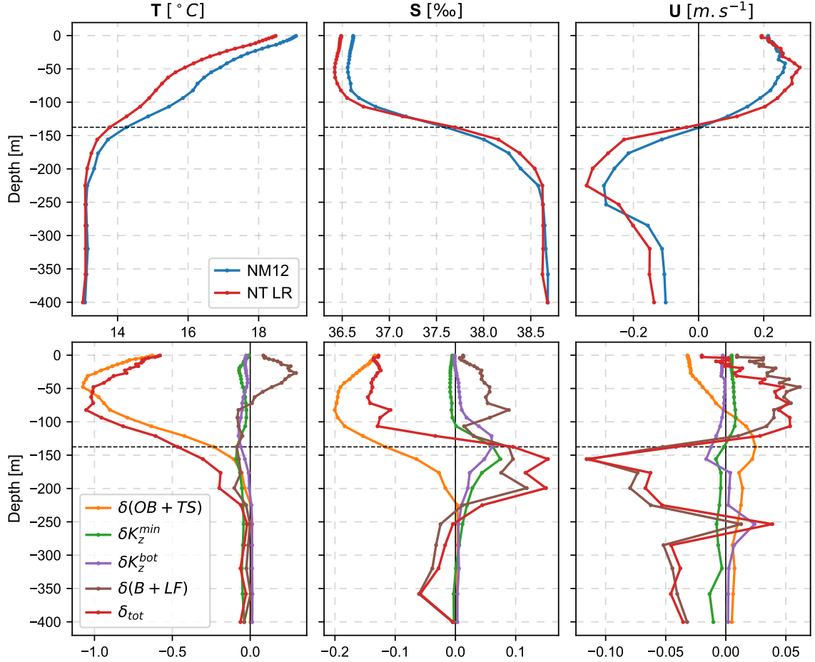
Figure A.1: Upper panels display vertical profiles of temperature, salinity, and zonal velocity for NEMOMED12 (NM12) and NEMOMEDGIB (NT LR) simulations, averaged at the SoG (6.1°W-5.25°W). Lower panels display the anomaly NT LR - NM12 ( \delta_{tot} ) and its decomposition into four components, associated with the main physical differences between both configurations. We consider four main steps of the NEMOMED12 modifications: the replacement of the Atlantic buffer zone with open boundary conditions and the addition of time splitting (OB + TS), the decrease of background vertical mixing coefficients and the modification of the TKE mixing length-scales formulation ( K_z^{min} ), the removal of background tidal TKE energy and the activation of logarithmic bottom friction formulation ( K_z^{bot} ), the modification of NEMOMED12 bathymetry at the SoG and the decrease of lateral friction (B+ LF). The total anomaly between both configurations is displayed in red ( \delta_{tot} ). The horizontal dashed line represents the depth of the zero velocity interface in the NEMOMED12 simulation.
