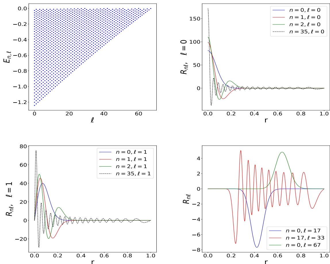
Figure 5.1. Energy levels E_{nl} in the (l, E_{nl}) plane ( upper left panel ), for the gravitational potential (5.35). Eigenmodes \mathcal{R}_{nl}(r) for l = 0 ( upper right panel ), l = 1 ( lower left panel ) and some large values of n or l ( lower right panel ).
