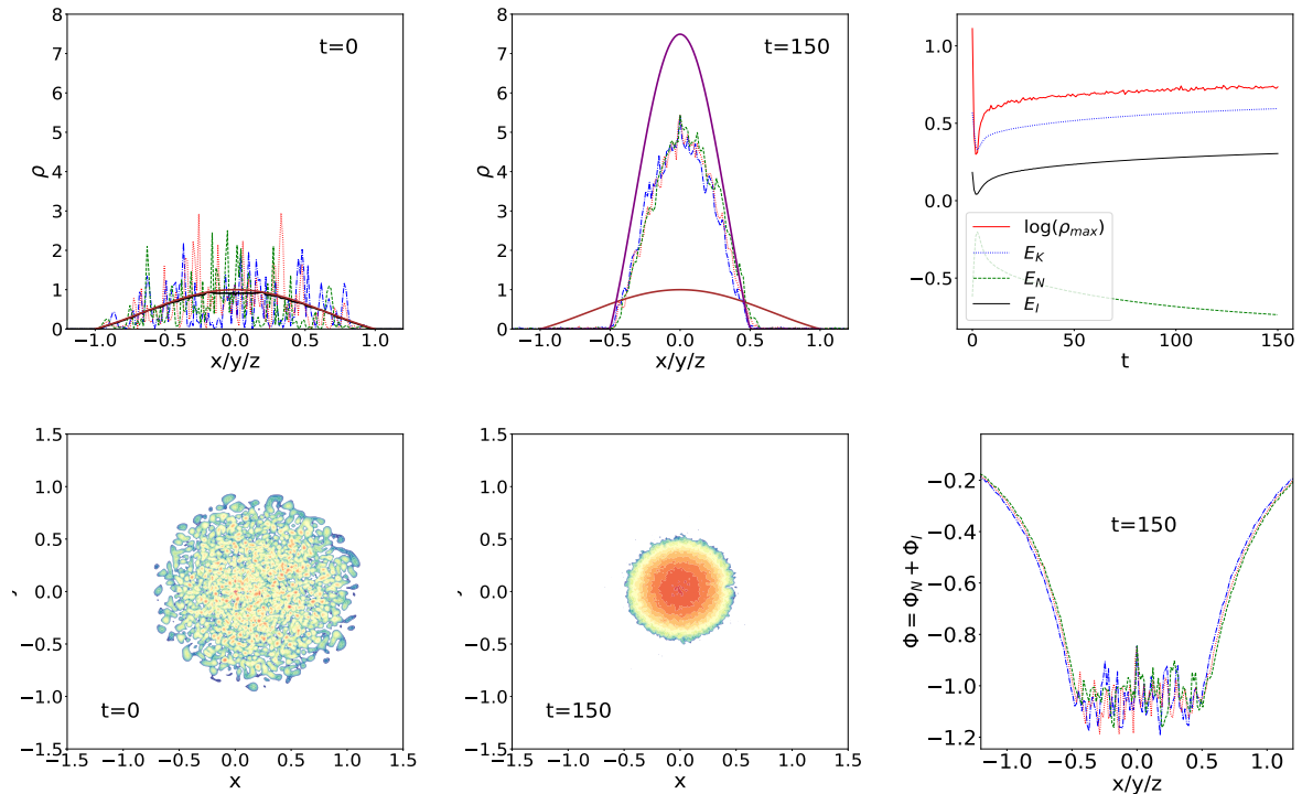
Figure 5.2. [ R_{sol} = 0.5 , \rho_{0sol} = 0 .] Upper left panel: Initial density \rho along the x (blue dash-dot line), y (red dotted line) and z (green dashed line) axis running through the center of the halo. The smooth brown solid line is the target density profile (5.35) and the black wiggly solid line is the averaged density \langle \rho_{halo} \rangle of Eq.(5.24) (they can hardly be distinguished in the figure). There is no central soliton in this initial condition. Upper middle panel: density profile along the x , y and z axis that run through the point \vec{r}_{max} where the density is maximum, at time t = 150 . The lower brown solid line is the initial target density profile as in the upper left panel, while the upper purple solid line is the density profile of a soliton (5.14) that would contain all the mass of the system. Upper right panel: evolution with time of the maximum density and of the kinetic, gravitational and self-interaction energies. Lower left panel: initial density profile on the 2D (x, y) plane at z = 0 . Lower middle panel: density profile at time t = 150 on the 2D (x, y) plane centered on \vec{r}_{max} . Lower right panel: total potential \Phi = \Phi_N + \Phi_I at t = 150 , along the x , y and z axis passing through \vec{r}_{max} .
