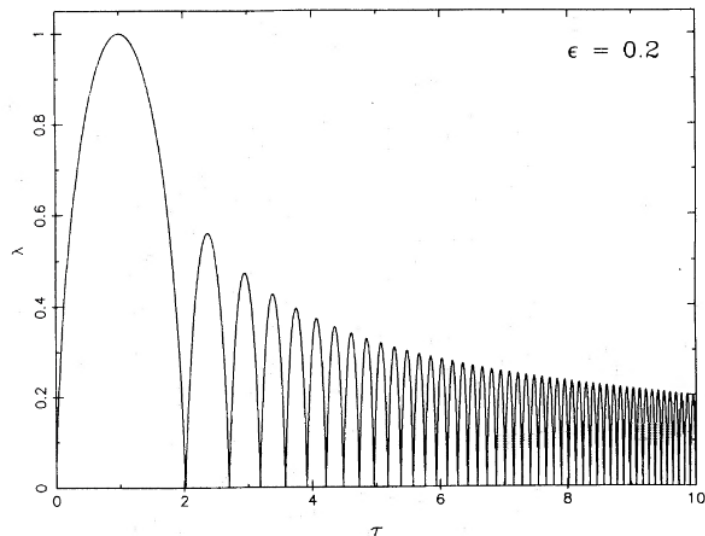
Figure 3.11. Figure from Fillmore & Goldreich (1984) . CDM self-similar particle trajectory for \epsilon=0.2 ( \gamma in (3.85))
