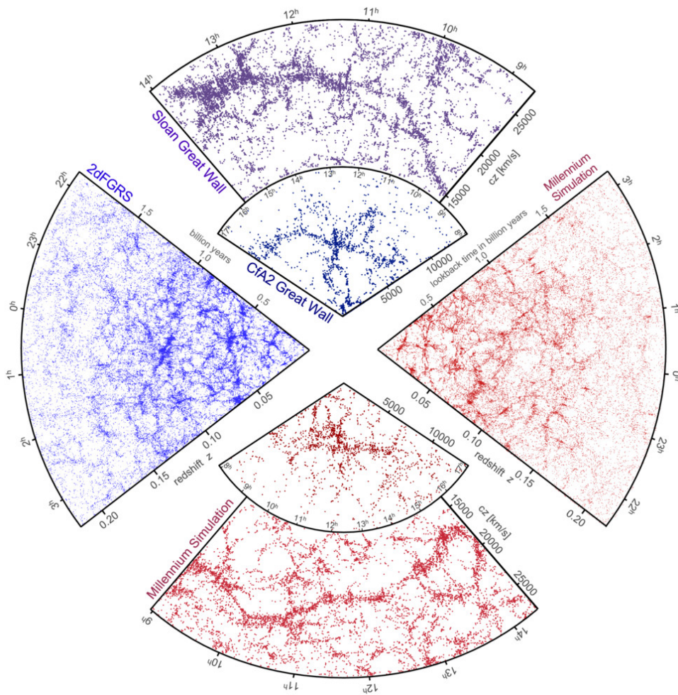
Figure 1.9. Figure from https://wwmpa.mpa-garching.mpg.de/millennium/ . Large scale structure of the Universe. In blue, observations by the 2dF Galaxy Redshift Survey (Colless et al., 2001), the Sloan Digital Sky Survey (Gott et al., 2003) and the CfA Redshift Survey (Geller & Huchra, 1989). Each point represents a galaxy as a function of R.A. and redshift. The three redshift survey are accompanied by the corresponding N-body Millenium-II simulations considering the \Lambda CDM in red.
