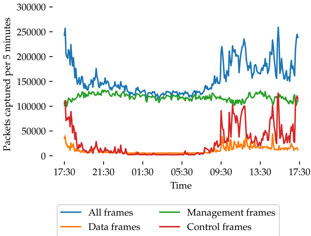
Figure 4.5. – Traffic load for the whole duration of 24 hours. The traffic is split into the data, management, and control frames, per 5 minutes each.
