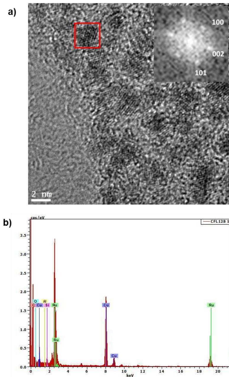
Figure 3.10. a) HREM image of \text{Ru}@C_{66}(\text{COOH})_{12} 6/1; inset: Fast Fourier Transform (FFT) with the corresponding orientation of the Ru lattice; and b) EDX of \text{Ru}@C_{66}(\text{COOH})_{12} .
