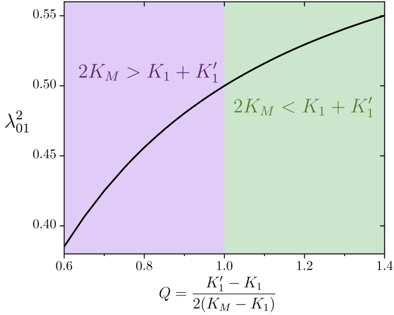
Figure 3.11: Variations of the S_M = 0 weight \lambda_{01}^2 as a function of the dimensionless parameter Q (see equation (3.6)) in the second lowest lying triplet state (see equation (3.5)) for a Td compound characterised by K_1 = K_2 and K'_1 = K'_2 . The mixing is maximal ( \lambda_{11}^2 = \lambda_{01}^2 = 1/2 ) for Q = 1 (i.e. 2K_M = K_1 + K'_1 ).
