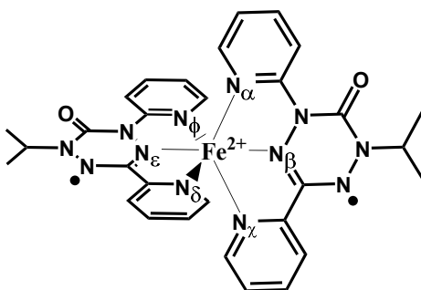
Figure 3.18: [\text{Fe}(\text{dipyvd})_2]^{2+} compound 3 from Ref [263]. The Xray Fe- N_i distances i = \alpha - \phi are 1.98, 1.84, 1.95, 2.00, 1.85, and 1.98 Å, respectively.
