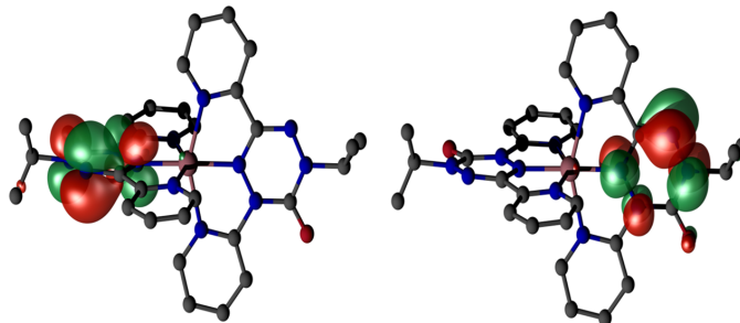
Figure 3.14: CAS[2,2] triplet MOs of the fictitious compound 2 , Zn analogue of 1 .
