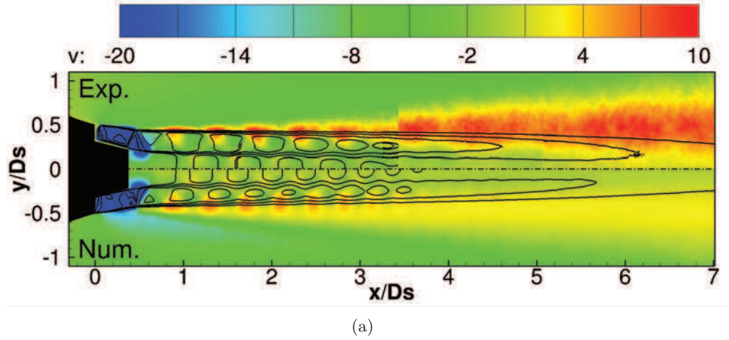
Figure 6.8: (a) Radial velocity \bar{v}_r contours of the mean field from PIV (top) and LES (bottom). The black solid lines represent the Mach number from 0.9 to 1.4 with an interval of 0.1.
