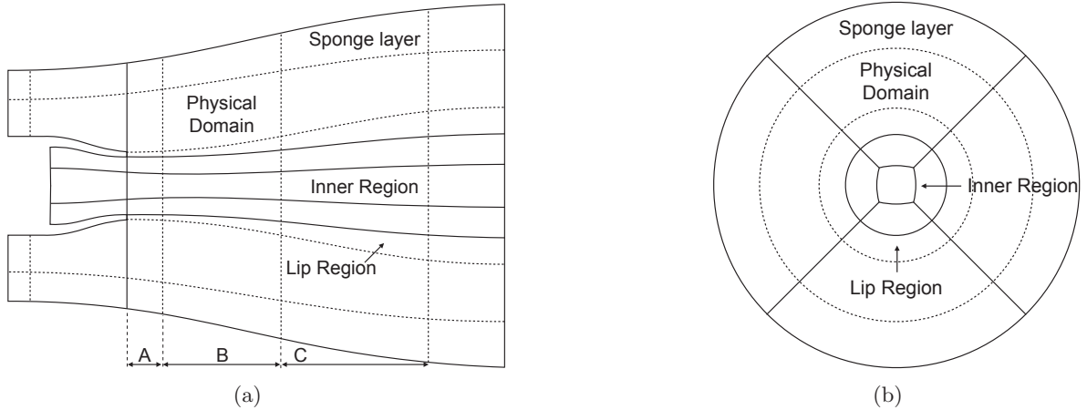
Figure 3.2: Sketch of a domain for a jet. In solid lines are represented the block boundaries and in dashed lines the different regions inside each block. (a) axial representation. (b) radial representation.
