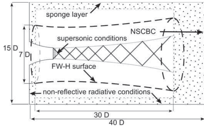
Figure 5.3: Sketch of the domain representing the different boundary conditions and dimensions.
