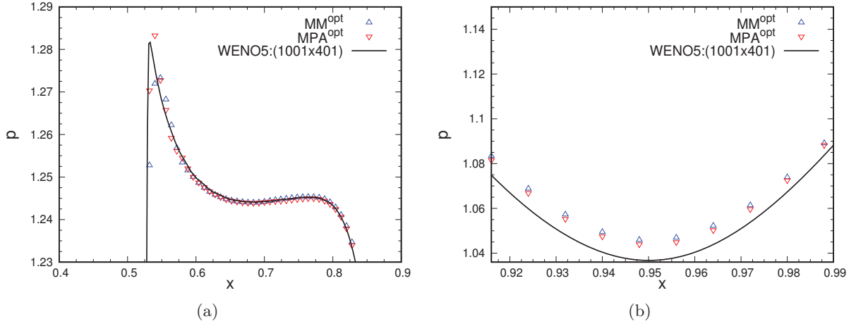
Figure 7.15: Comparison of pressure profiles for MM^{opt} and MPA^{opt} filters with reference WENO5 scheme (a) downstream of the shock, and (b) center of the vortex core at y = 0.5 cross-section and t = 0.6 . Filtering magnitude \sigma^{sc} is evaluated using Ducros sensor (see Eq. 7.7).
