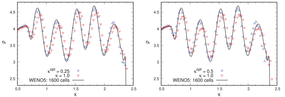
Figure 7.12: Comparison of density profiles of \kappa^{\text{opt}} and \kappa = 1.0 for (a) minmod and (b) MPA filters with the reference WENO5 scheme at t = 1.8 . Parameter \tilde{\delta} = 1.0 for both cases.
