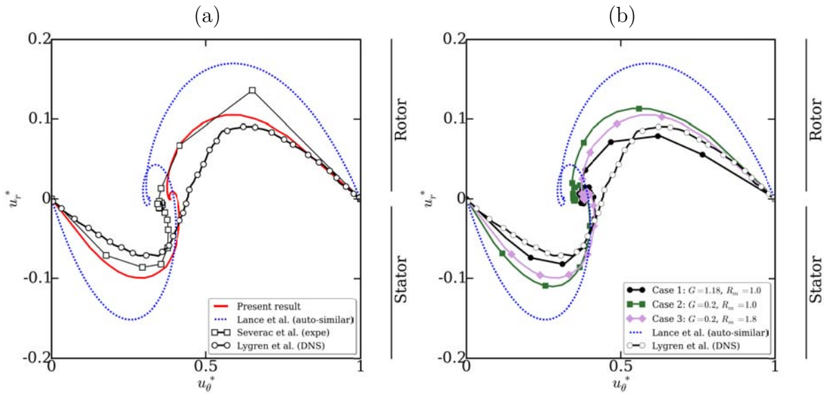
Figure 3.5 – Polar plot of the dimensionless mean velocity distribution at r^* = 0.5 . (a) Comparison between (—) the LES results, (—□—) the LDV data by Séverac et al. (2007), (—) the auto-similar solution by Rogers & Lance (1962) and (—○—) the DNS results by Lygren & Andersson (2001). (b) Comparison between the results from (—●—) Case 1 , (—■—) Case 2 and (—◆—) Case 3 , along with the (—) auto-similar solution by Rogers & Lance (1962) and (—○—) the DNS results by Lygren & Andersson (2001).
