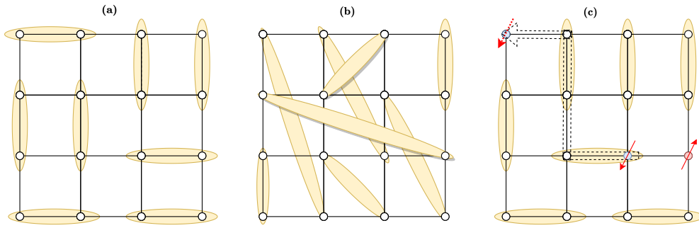
FIGURE 4.1: (a) An example of nearest neighbor valence bond configuration. The NN-RVB state is the equal-weight superposition of all such configurations. (b) A VBS with long-range dimers. (c) A spinon excitation in a NN VBS state. The dotted line corresponds to the path taken by a spinon.
