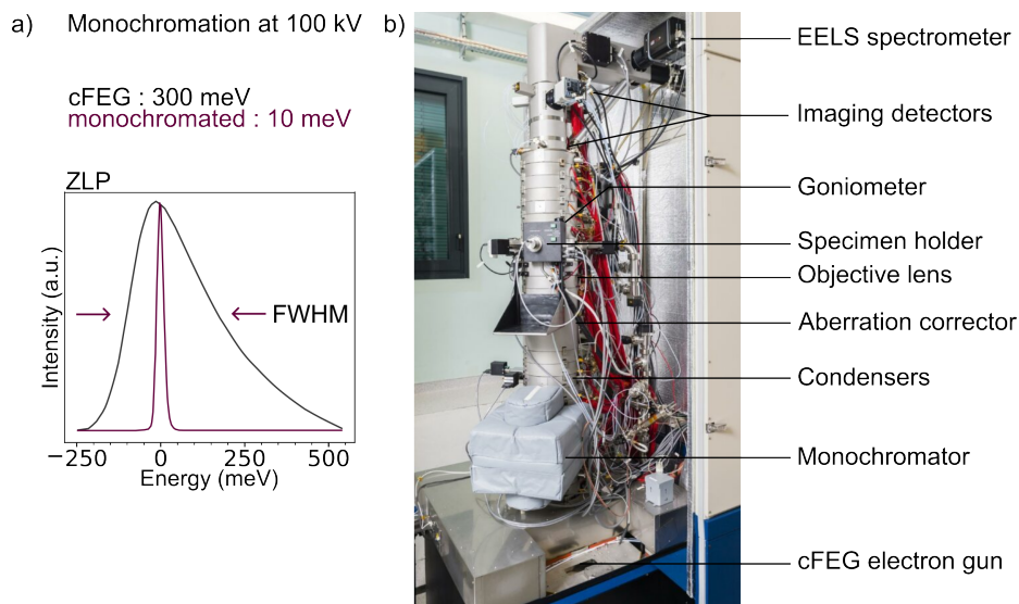
Figure 2.6: a) Example of the monochromatization: before monochromatization, the energy spread of the cFEG reaches 300 meV, while it is narrowed to 10 meV after monochromatization (measured at the Full Width Half Maximum, FWHM). b) Photograph of the Cs aberration-corrected Nion Hermes 200-S microscope, equipped with a monochromated cFEG electron gun.
