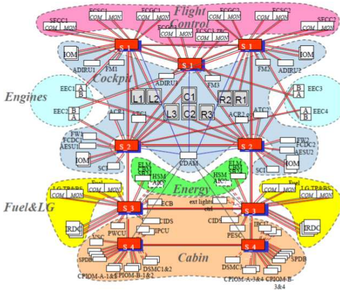
Figure 6.2: AFDX network architecture (Courtesy of: ARTIST2 - IMA A380)
