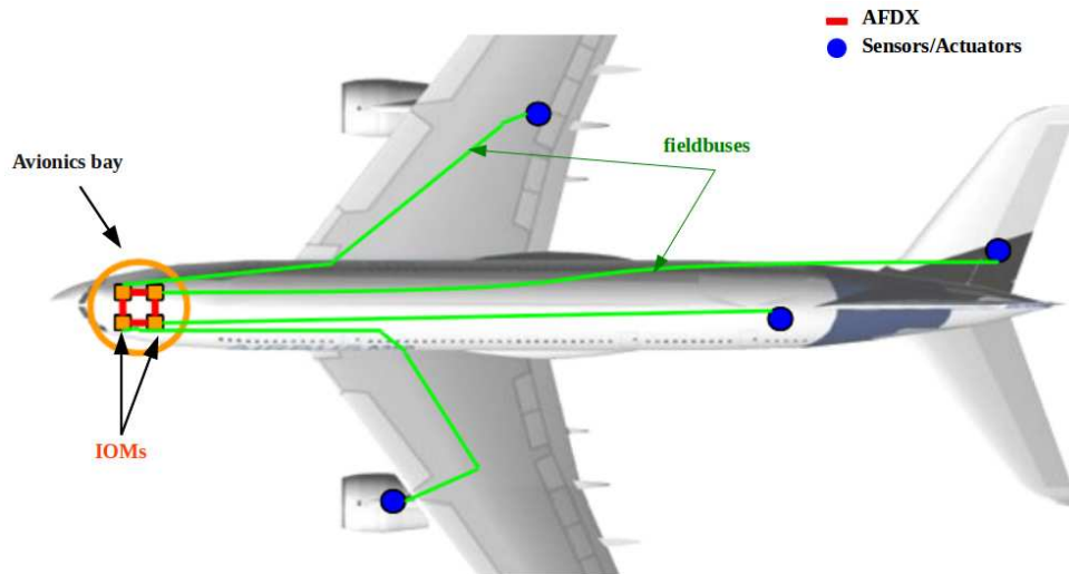
Figure 1.2: Centralized avionic architecture
