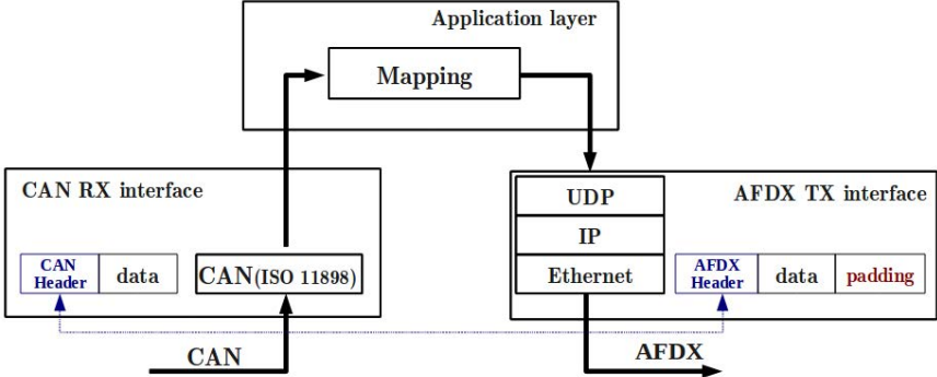
Figure 3.3: The current CAN-AFDX RDC: (1:1) strategy
