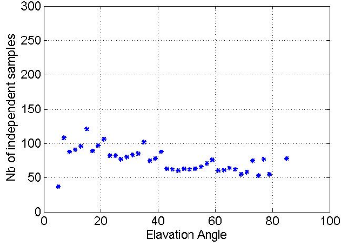
Figure 46 – Number of independent samples per bin, with unique bin for elevation >80^\circ , for GPS
