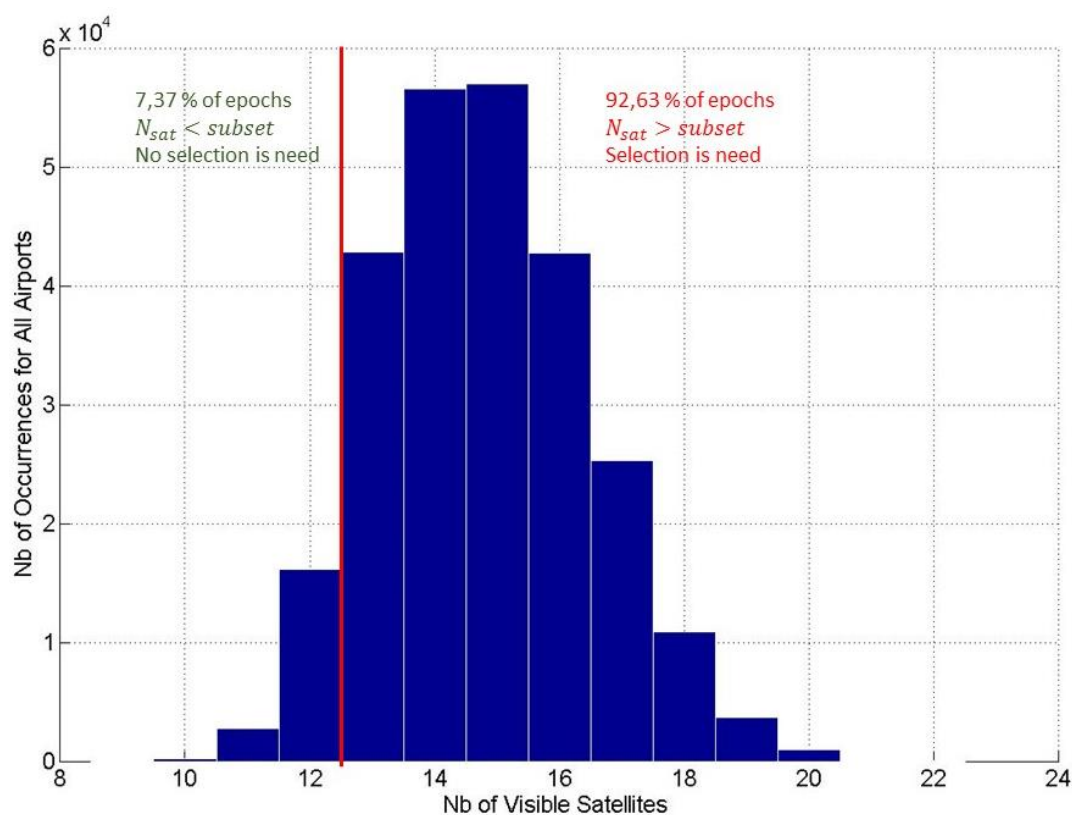
Figure 53 – Histogram of satellites number across all airports and epochs with percentage of use of satellite selection for subset 12
