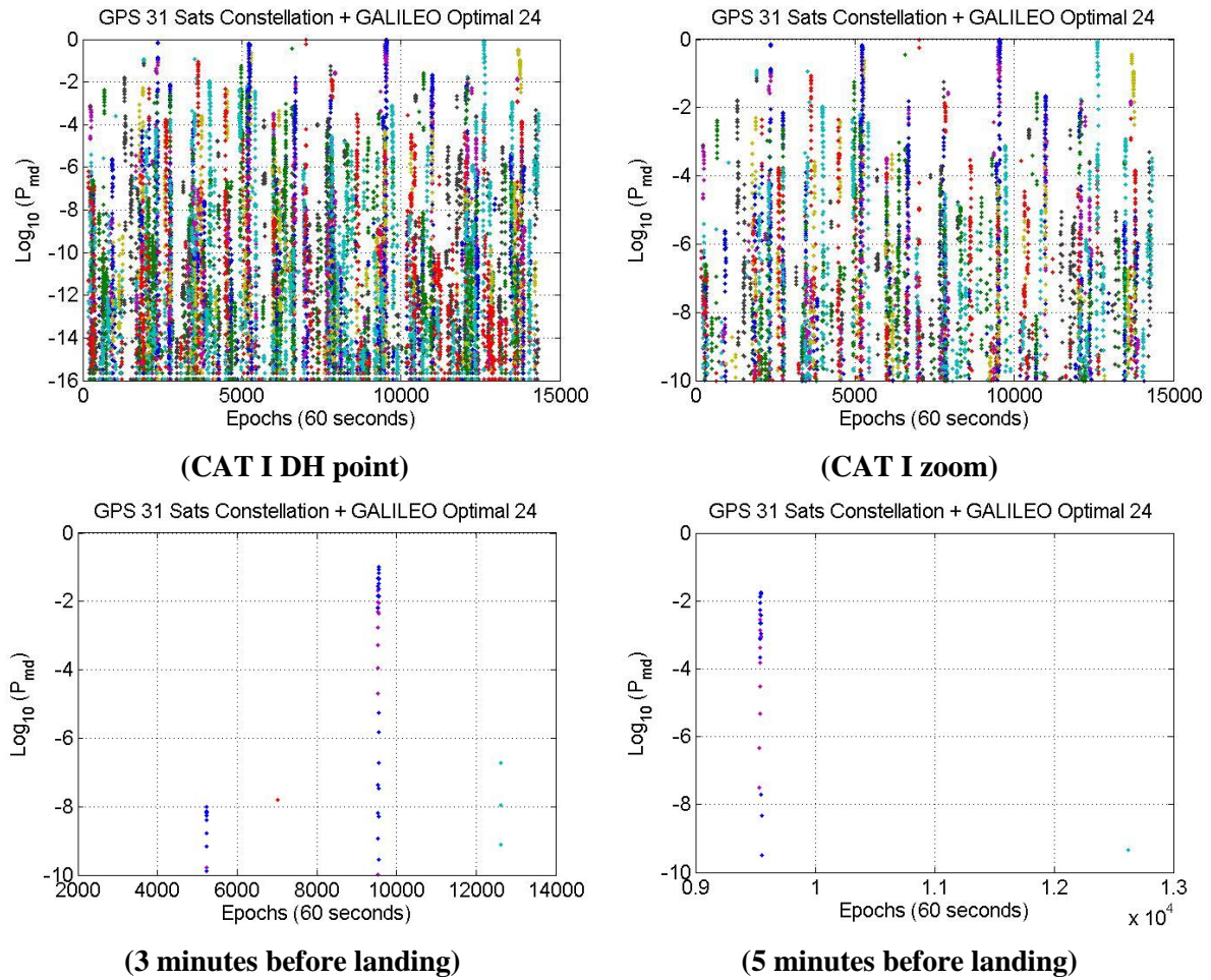
Figure 104 – DRAIM P_{md} for an ionospheric front induced error for GPS 31 satellites and Galileo Optimal 24 and \Delta v = 70 m/s for all airports
