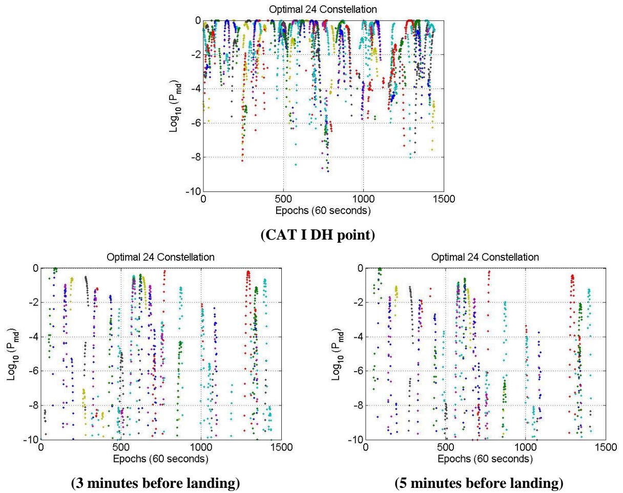
Figure 96 – DRAIM P_{md} for ionospheric front induced error for GPS optimal 24 and \Delta v = 35 \text{ m/s} for all airports
