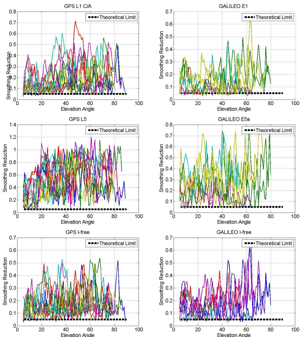
Figure 134 – Real Vs. theoretical smoothing gain for GPS (left side) and Galileo (right side) signals for Toulouse Blagnac 03/04/2016 on RR1
