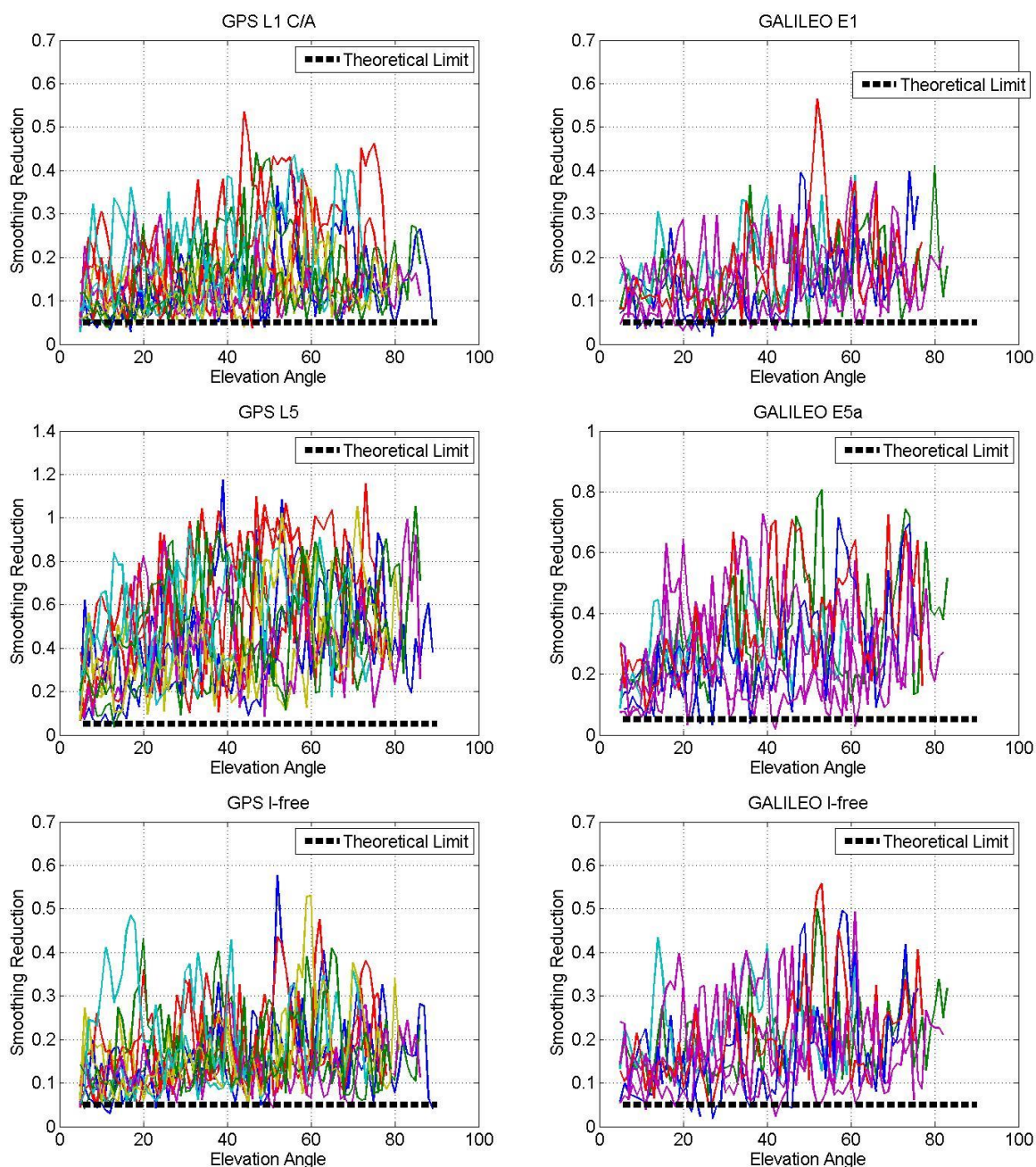
Figure 136 – Real Vs. theoretical smoothing gain for GPS (left side) and Galileo (right side) signals for Toulouse Blagnac 06/04/2016 on RR1
