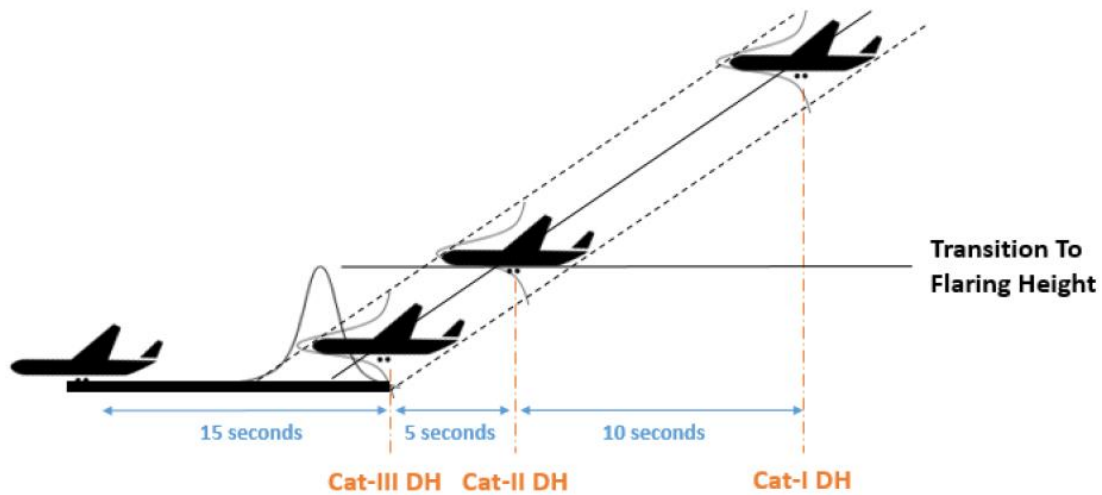
Figure 111 – Autoland method
