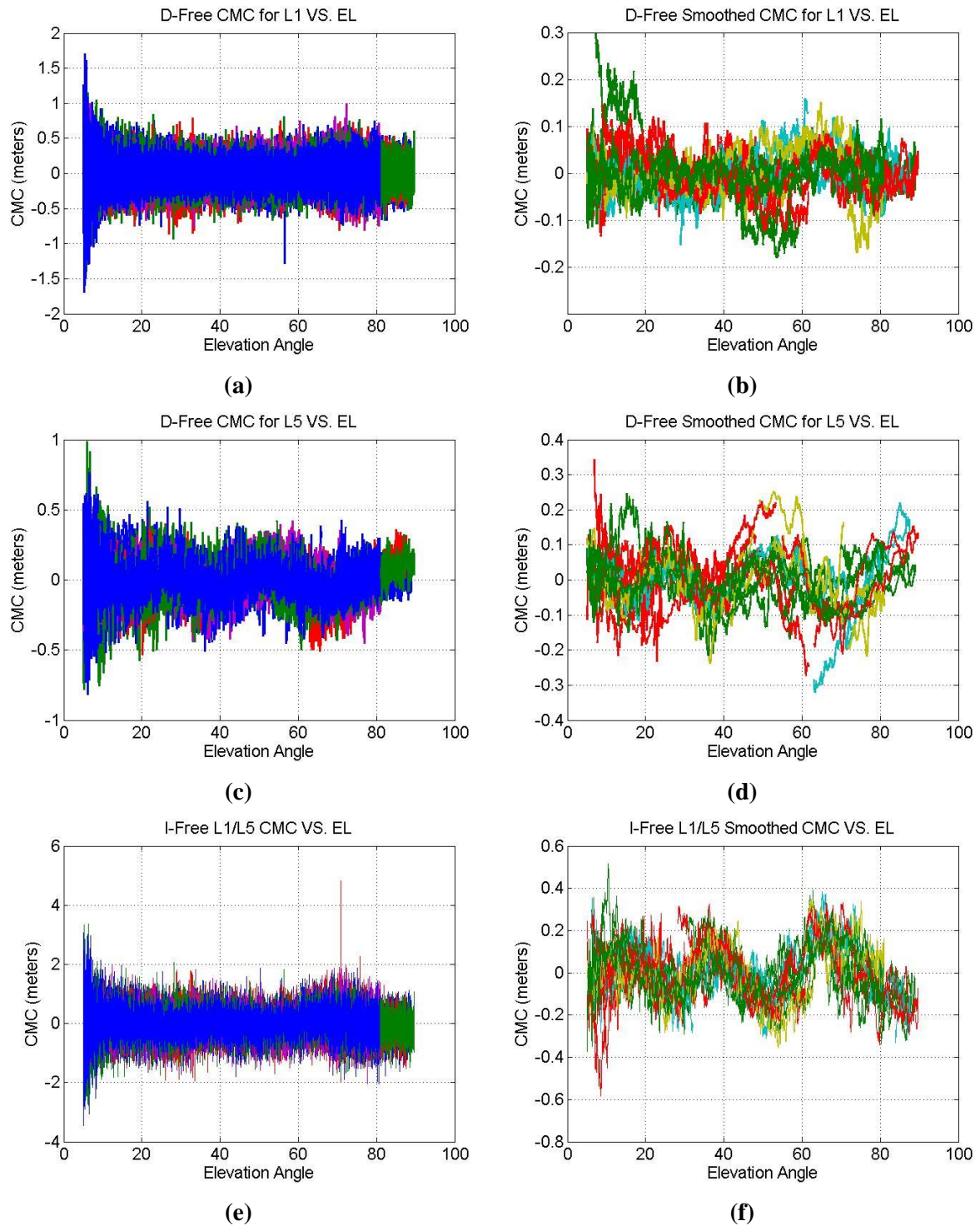
Figure 112 – GPS L1 C/A, GPS L5 and I-Free raw and smoothed CMC for all satellites Pattonville 50 m. case
