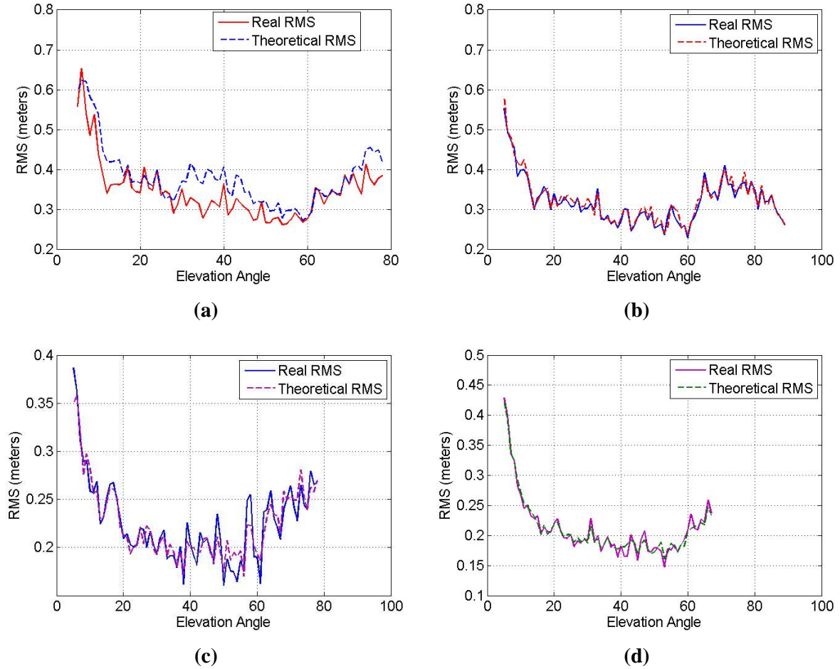
Figure 37 – Real and theoretical I-free CMCs RMS comparison on GPS for PRN 3 (a) PRN 8 (b) and Galileo PR8 (c) and PRN 26 (d)
