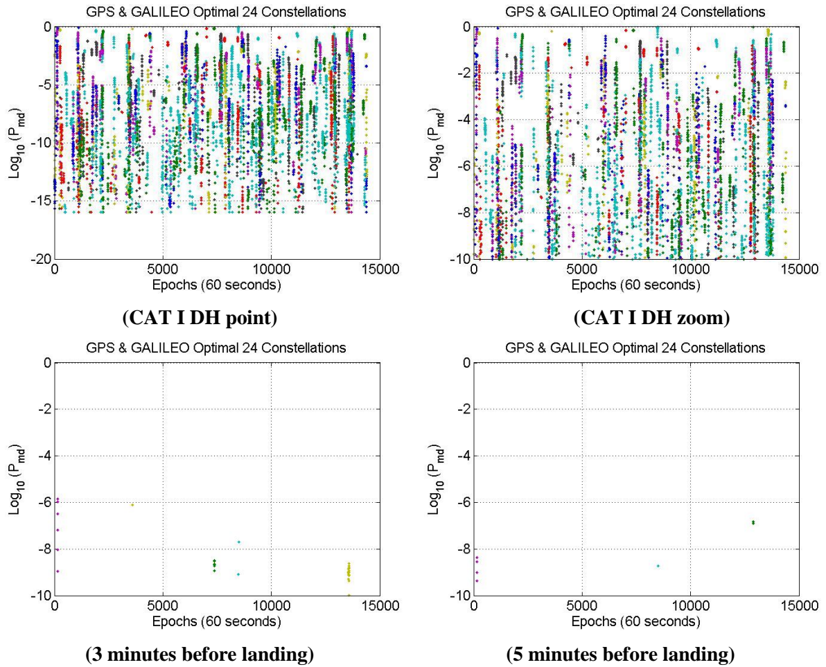
Figure 105 – DRAIM P_{md} for an ionospheric front induced error for GPS & Galileo Optimal 24 and \Delta v = 35 m/s for all airports
