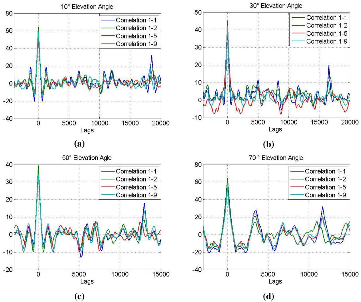
Figure 40 – Day-to-day autocorrelation functions for different elevation angles
