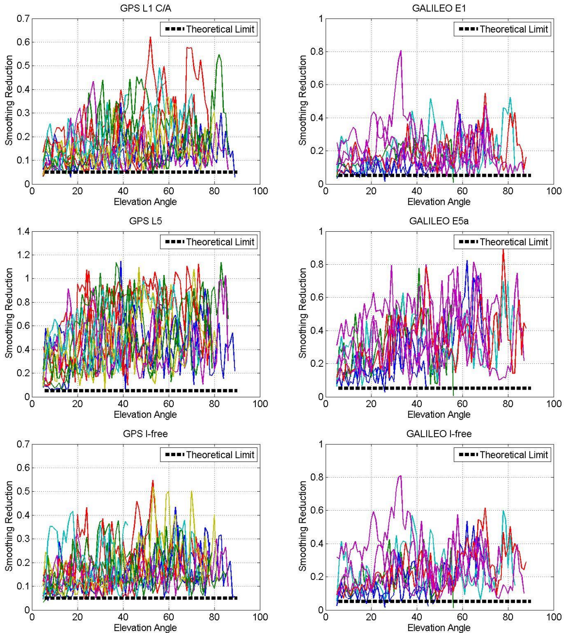
Figure 138 – Real Vs. theoretical smoothing gain for GPS (left side) and Galileo (right side) signals for Toulouse Blagnac
