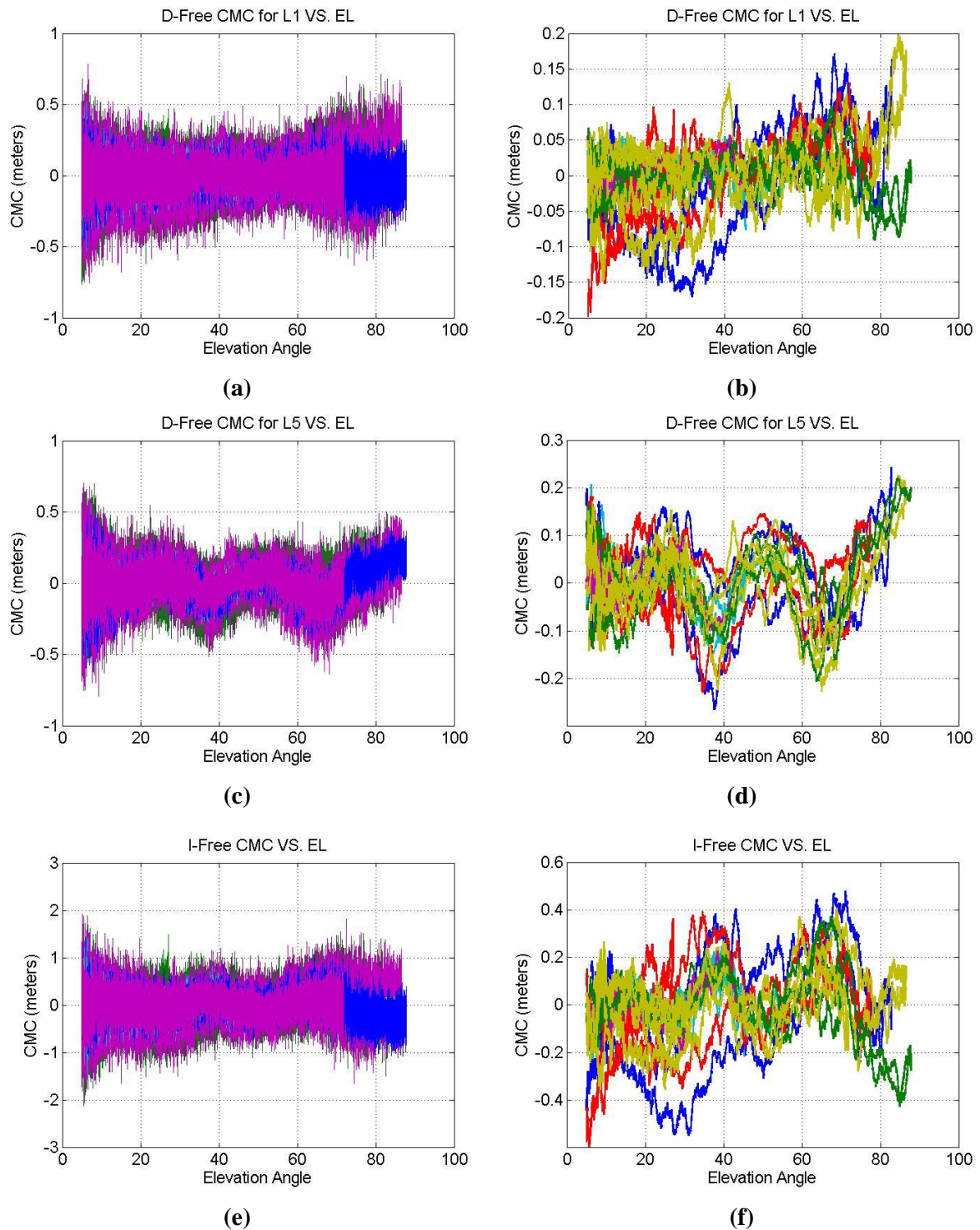
Figure 127 – Galileo E1, Galileo E5a and I-Free raw and 100 seconds smoothed CMCs for all satellites Toulouse Blagnac RRI 09/04/2016
