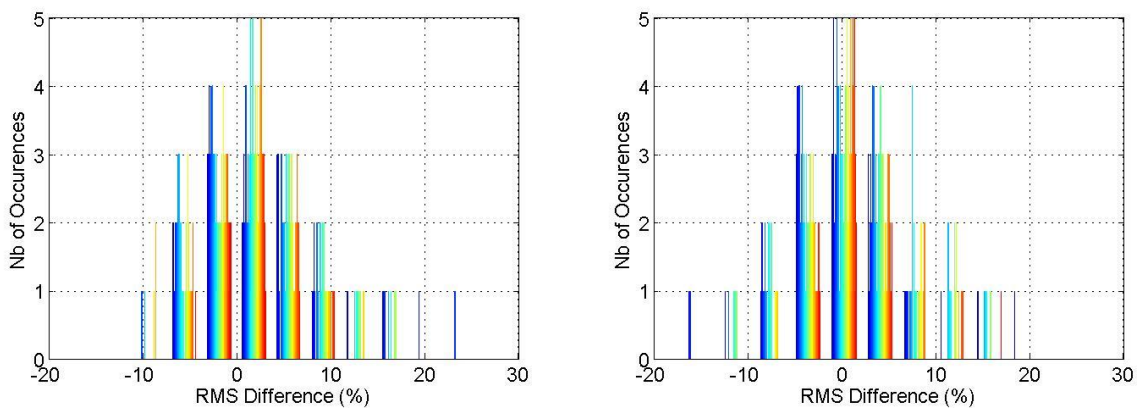
Figure 143 – RMS difference percentage distribution for GPS I-free for Pattonville 50 m (left side) and 100 m (right side), each color represents a satellite
