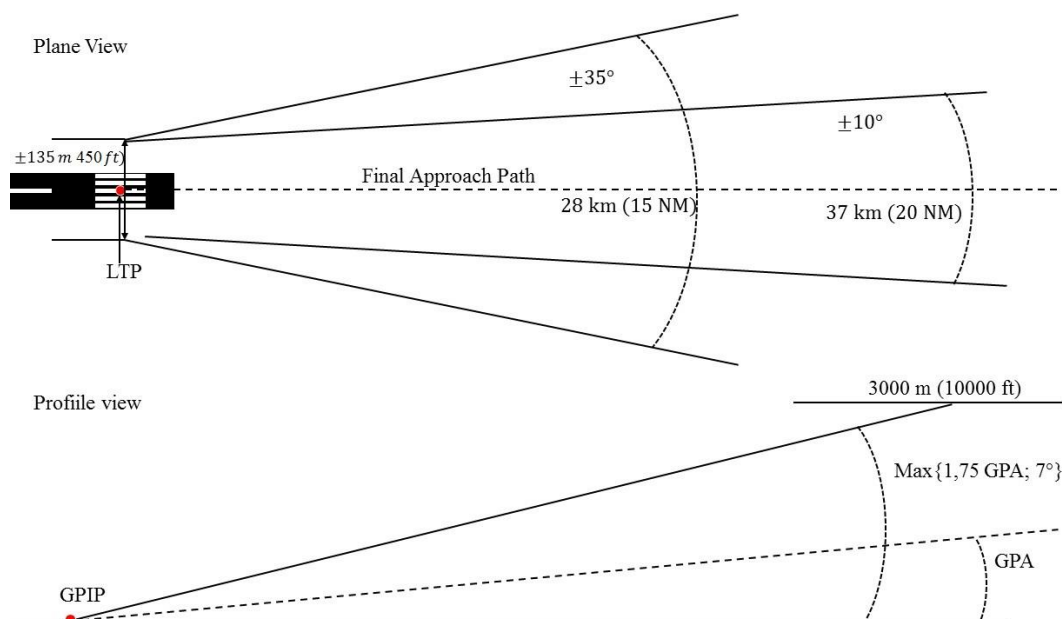
Figure 11 – GBAS Runway coverage
