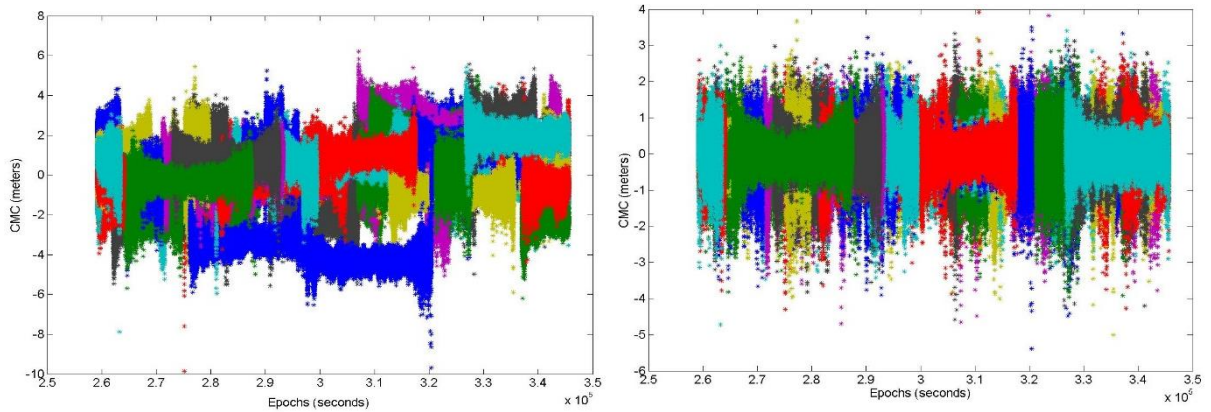
Figure 17 – CMCs before (left) and after (right) phase ambiguity term compensation (each color represent a PRN)
