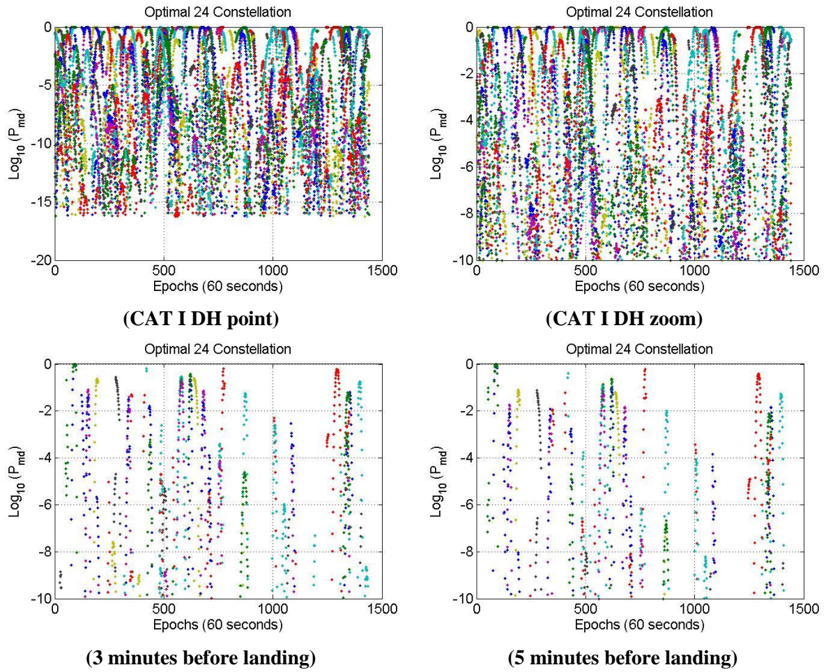
Figure 94 – DRAIM P_{md} of ionospheric front induced error for GPS Optimal 24 and \Delta v = 70 m/s for all airports
