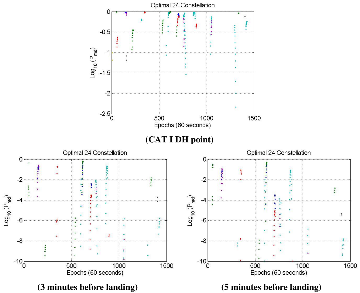
Figure 98 – DRAIM P_{md} for ionospheric front induced error for GPS optimal 24 and \Delta v = 0 m/s for all airports
