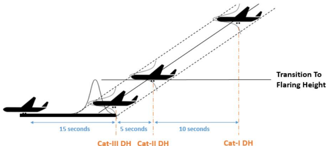
Figure 111 – Autoland method
