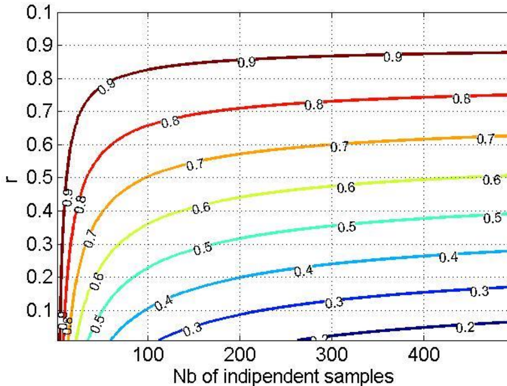
Figure 47 – \rho coefficients as function of n and r
