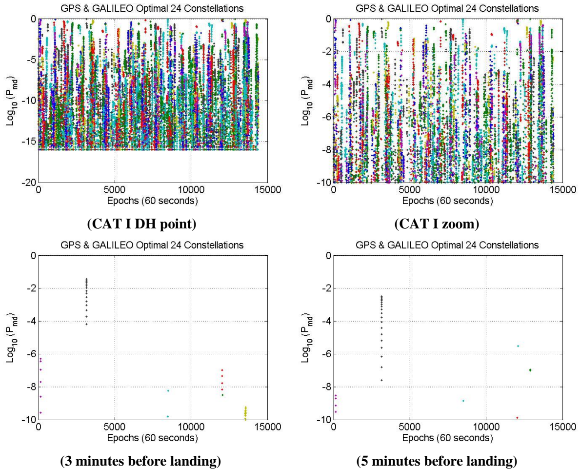
Figure 103 – DRAIM P_{md} for an ionospheric front induced error for GPS & Galileo Optimal 24 and \Delta v = 70 m/s for all airports
