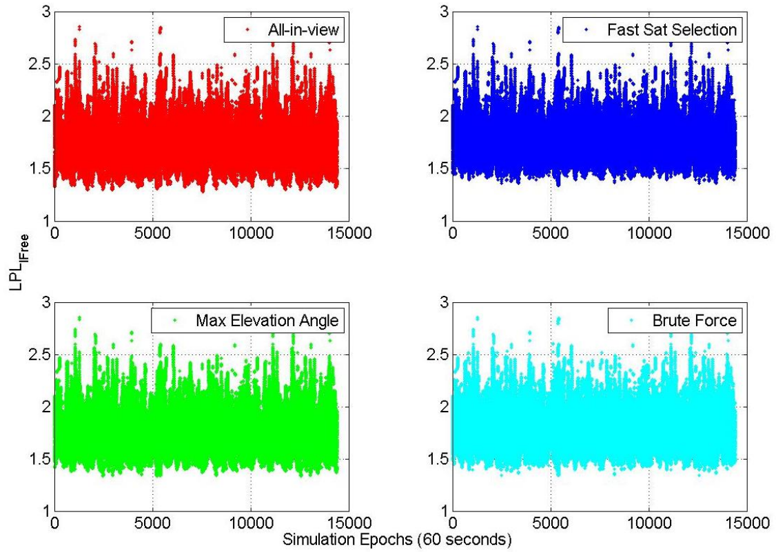
Figure 73 – I-Free LPL for all the epochs and airports for all the analyzed methods and all-in-view satellites
