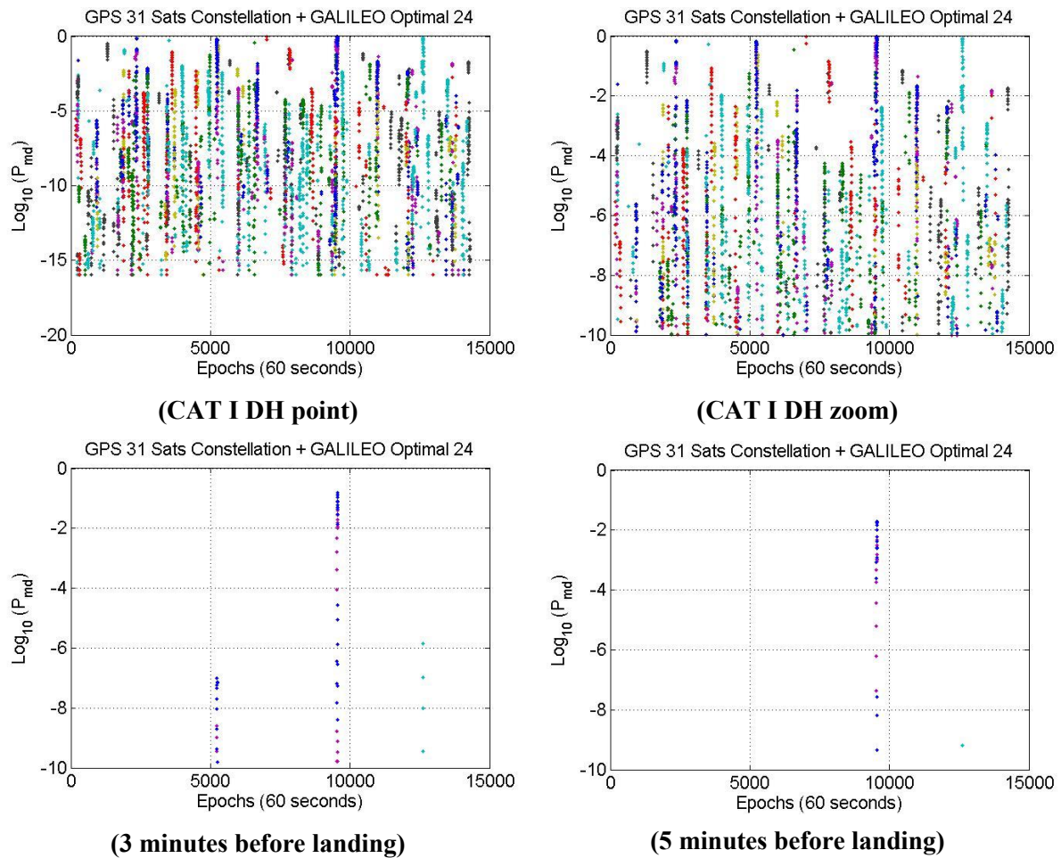
Figure 106 – DRAIM P_{md} for an ionospheric front induced error for GPS 31 satellites and Galileo Optimal 24 and \Delta v = 35 m/s for all airports
