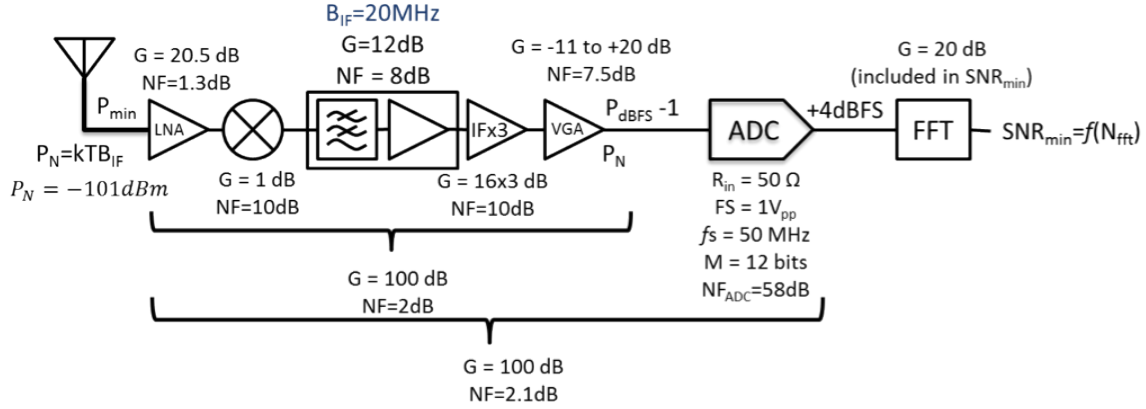
Fig. 2.16 Receiver design.
