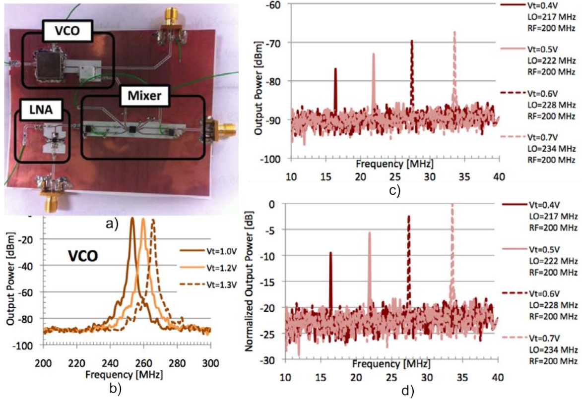
Fig. 4.9 Measurements of rollable radar module a) fabricated system b) VCO output c) full system measurements, mixer output d) full system measurements, mixer output (normalized).
