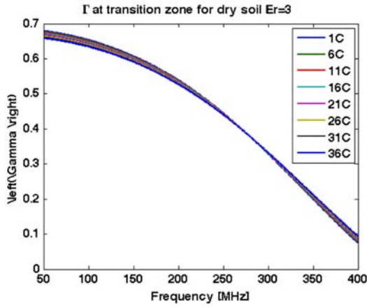
(a) dry soil ( \epsilon_r = 3 ), thin transition ( h = 0.1\text{m} )
