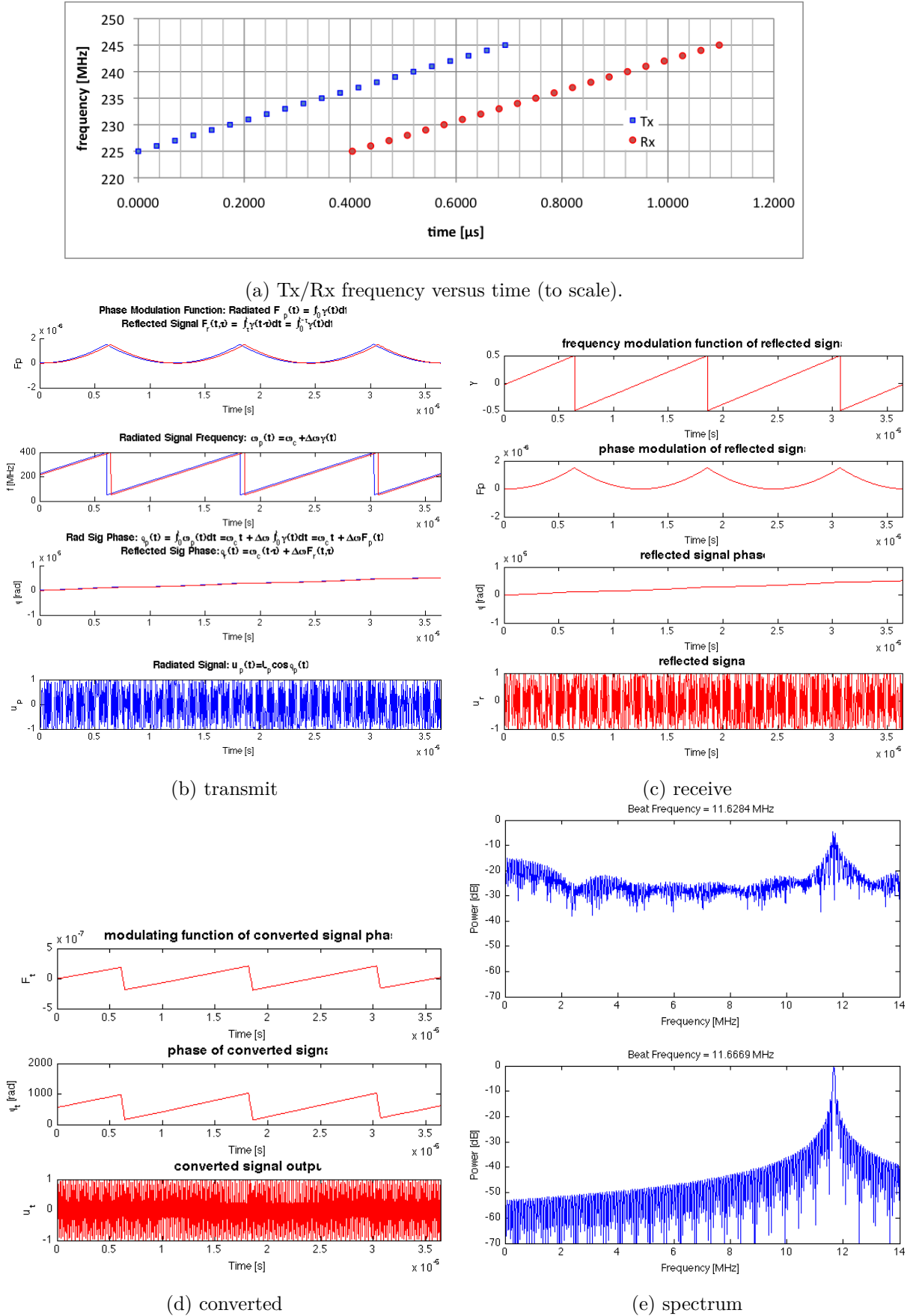
Fig. 2.7 Waveform properties to scale calculated using [60].
