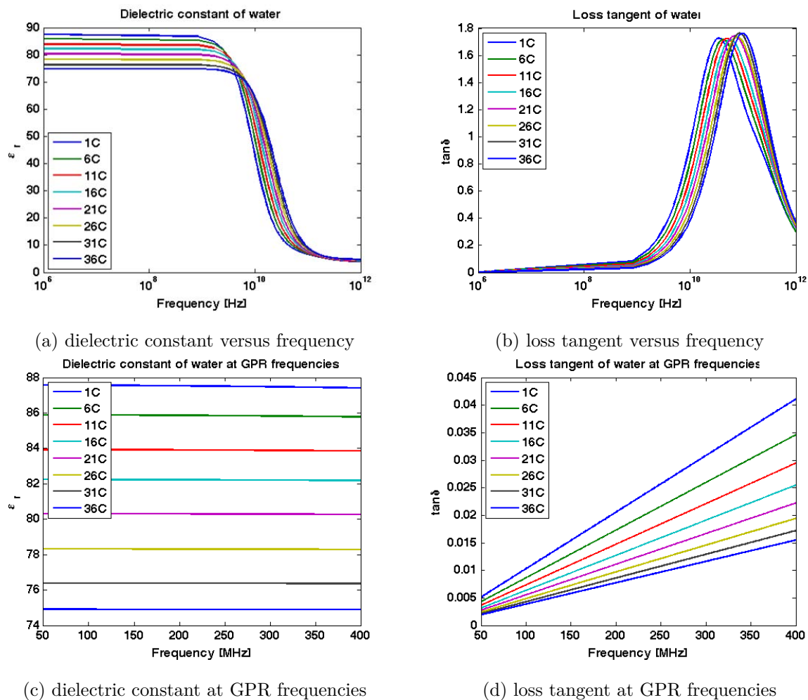
Fig. 2.8 Water properties.
