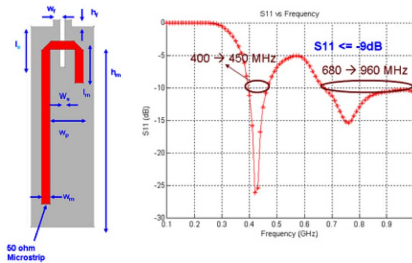
Fig. 4.21 Impedance matching.
