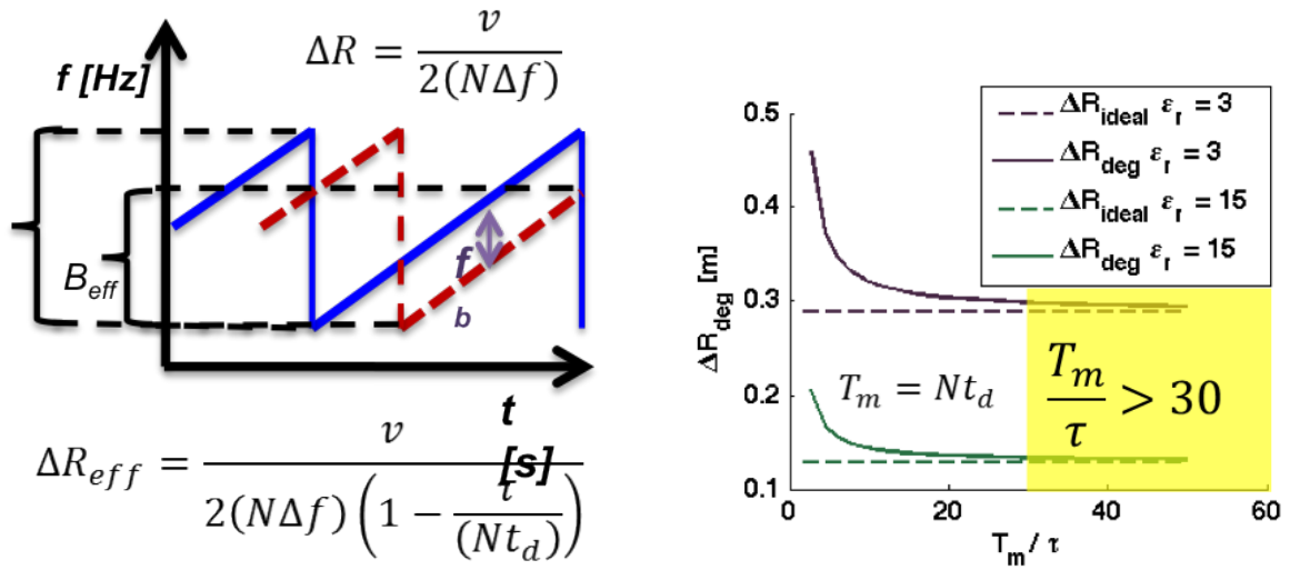
(a) effect of sweep rate on bandwidth and resolution
