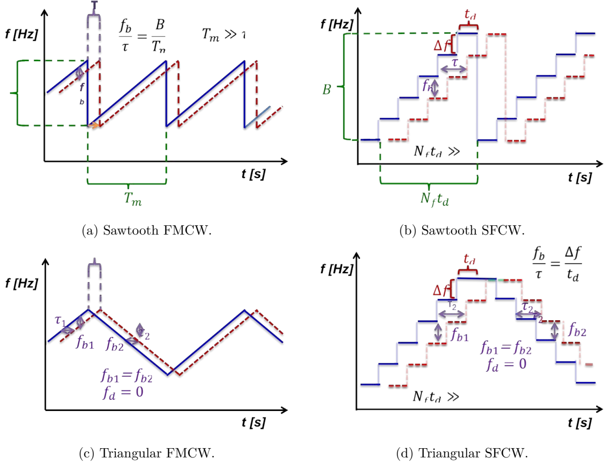
Fig. 2.3 Waveform.
