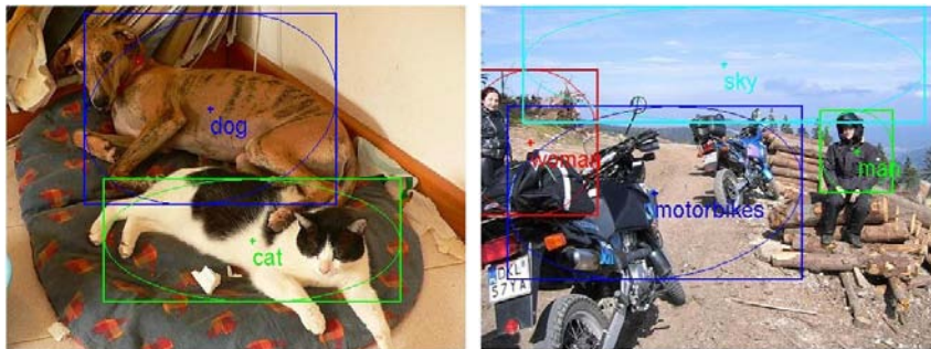
Figure 6.15: Results of our detection algorithm on images from the PASCAL VOC dataset.
