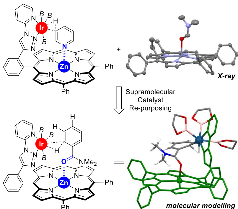
Figure 2. Previous supramolecular iridium catalyst displaying meta -selective C-H bond borylation of pyridines (top, left), ORTEP of assembly [ZnTPP ⊂ DMF] determined by single-crystal X-ray diffraction studies with thermal ellipsoids at 50% probability (all hydrogen atoms are omitted for clarity, top, right), re-purposed supramolecular iridium catalyst for the ortho -borylation of tertiary benzamides (bottom, left) and its PM3-minimized molecular modelling associated to a plausible intermediate (for clarity the methyl groups on the boryl ligand and all hydrogen atoms except those of the N,N-dimethylbenzamide substrate were omitted and the supramolecular ligand backbone is green color, bottom, right). B = (pinacolato)boron.
