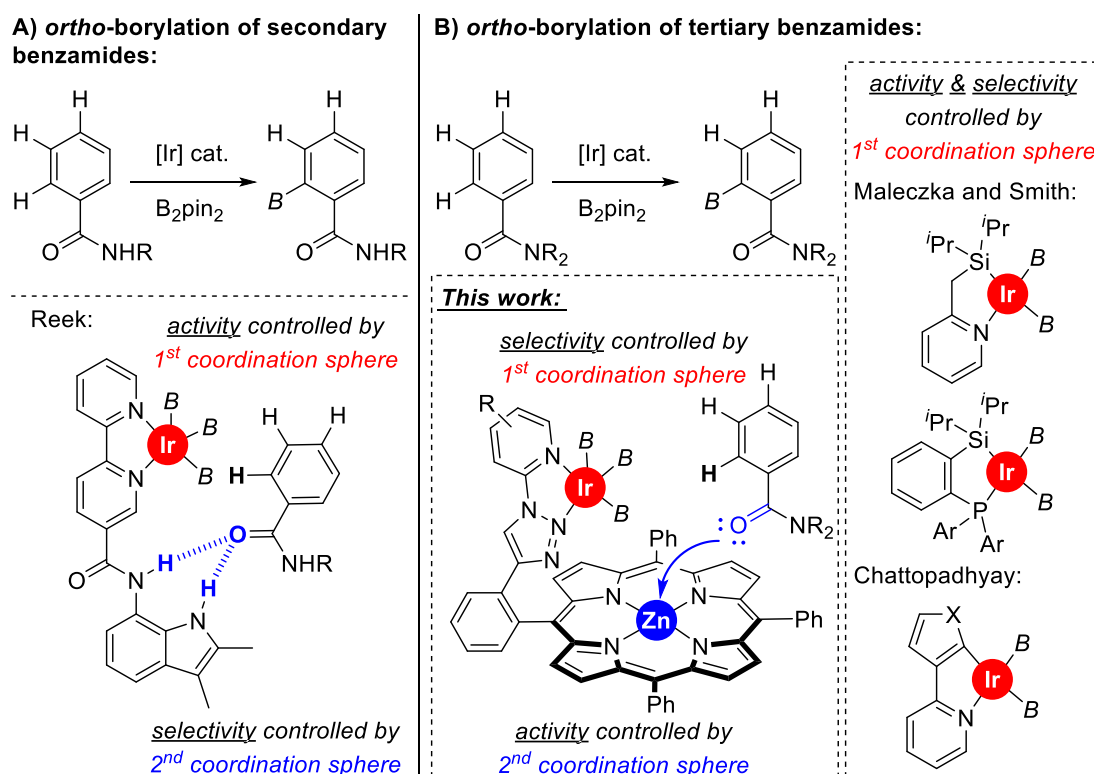
Figure 1. Previous catalysts enabling ortho -selective C-H borylation of benzamides ( A and B , right) and our supramolecular approach ( B , left). B 2 pin 2 = bis(pinacolato)diboron, B = (pinacolato)boron, Ar = para -tolyl.
