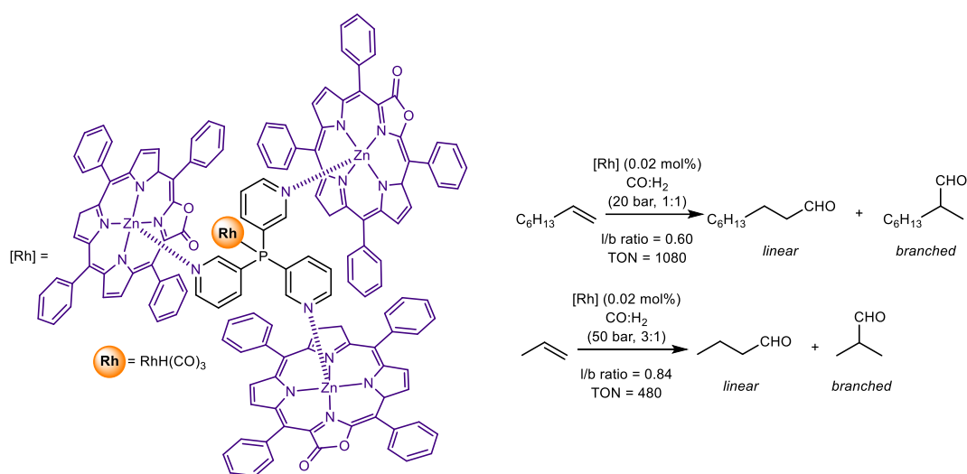
Scheme 31. The tris( meta -pyridyl)phosphine-ligated rhodium catalyst displays high branched selectivity and activity in the hydroformylation of olefins upon peripheral binding to zinc(II) porpholactone via Zn...N interactions.
