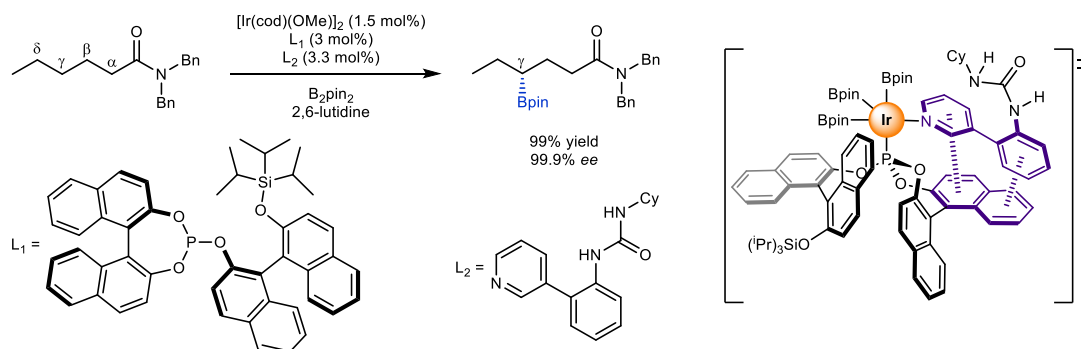
Scheme 20. Remote enantio-selectivity in the iridium-catalyzed C-H bond borylation with a ligand self-assembling by \pi\cdots\pi interactions.
