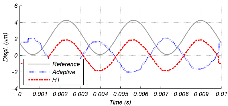
(c) Displacement reconstruction using proposed DAC algorithm.
