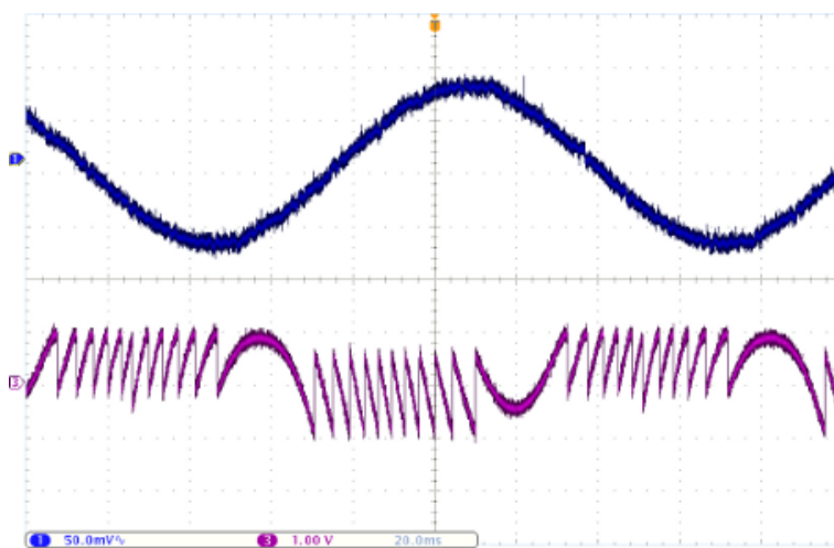
Figure 2.34 – Real-time reconstruction on top of simulated SM signal.
