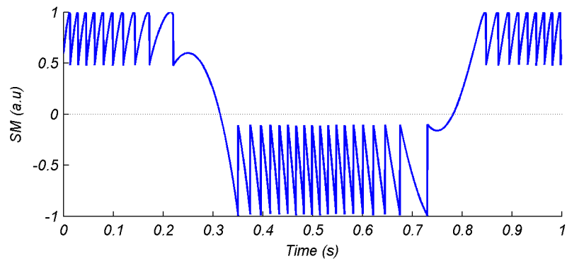
(a) Simulated SM signal with C = 7 and 10\lambda displacement.
