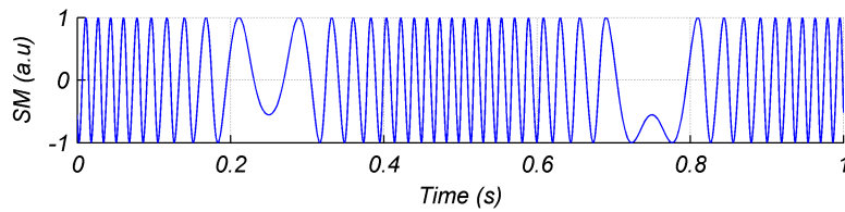
(a) Simulated SM with C = 0.2 from a target performing sinusoidal movement.
