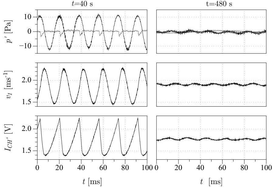
Figure 2.4: Simultaneous measurements of pressure (upper row), p'_0(t) (—) and p'_{M1}(t) (---), velocity signal (middle row) and heat release rate (bottom row). For two different instants left t = 40 s and right t = 480 s. Corresponding to T_s = 50 and 120 °C, respectively.
