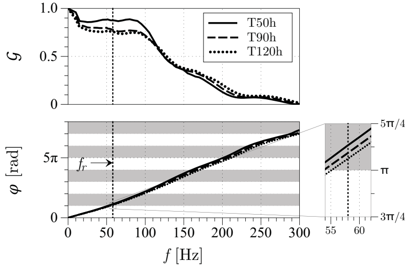
Figure 6.3: Flame transfer function for three different slot temperatures, T_s , corresponding to the cases T50h (—); T90h (----) and T120h (·····). Flow velocity and equivalent ratio are \bar{v} = 1.6 \text{ ms}^{-1} and \Phi = 0.95 , respectively. Velocity fluctuations are kept constant for all frequencies at \varepsilon = 0.1 . The reference point is located at y = -142 mm upstream of the flame.
