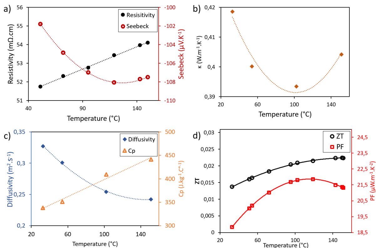
Figure-3.3.2. Dependence of TE properties of Bi 2 Te 3 /epoxy resin composite (prepared by infusion) on temperature measured in a heating mode: a) Resistivity and Seebeck coefficients; b) thermal conductivity (calculated); c) thermal diffusivity and specific heat; d) ZT and PF (calculated)
