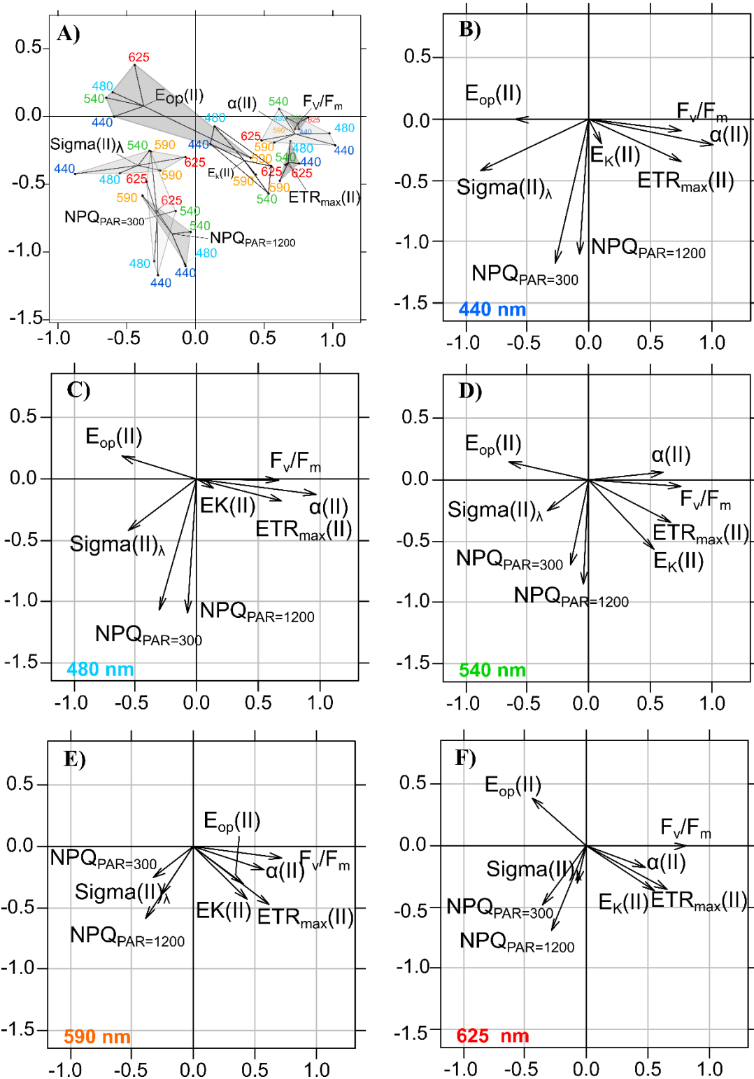
Figure II.9: Results of intrastructure of the partial triadic analysis of detrended photosynthetic parameters ETR_{max}(II) , E_k , \alpha(II) , E_{op}(II) , Sigma(II)_\lambda , F_v/F_m and NPQ at 300 and 1200 \mu\text{mol}\cdot\text{photons}\cdot\text{m}^{-2}\cdot\text{s}^{-1} projected on compromise coordinates (A). Each photosynthetic parameters coordinate is represented separately for each wavelength at 440 (B), 480 nm (C), 540 (D), 590 (E) and 625 (F) nm. See Table II.II for compromise contribution to total inertia and Table II.III for weight and \cos^2 of each of the wavelengths colors in PTA analysis.
