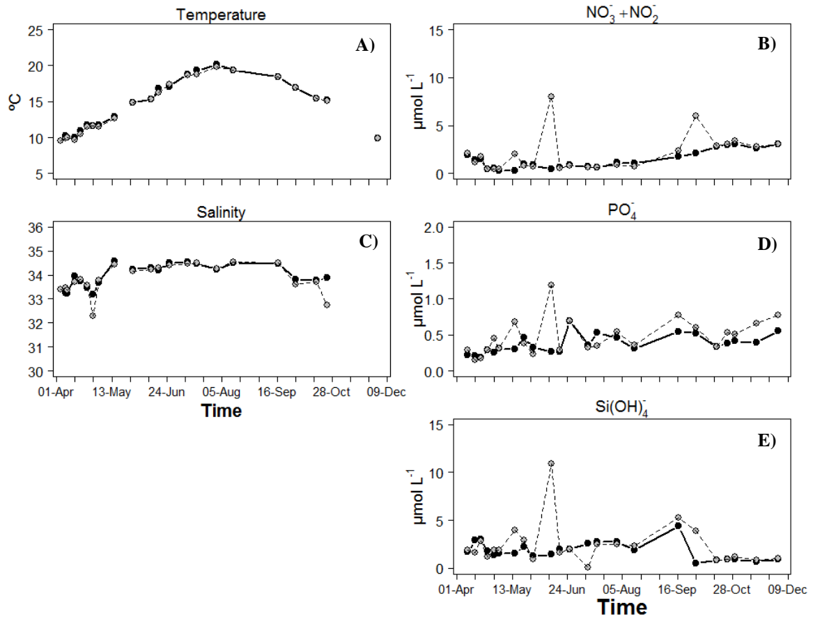
SM III-1 Abiotic parameters A) Temperature; B) \text{NO}_3^- + \text{NO}_2^- , C) Salinity; D) \text{PO}_4^- and E) \text{Si(OH)}_4 concentration in \mu\text{mol L}^{-1} . Gray and black symbols represent low and high tide values respectively.
