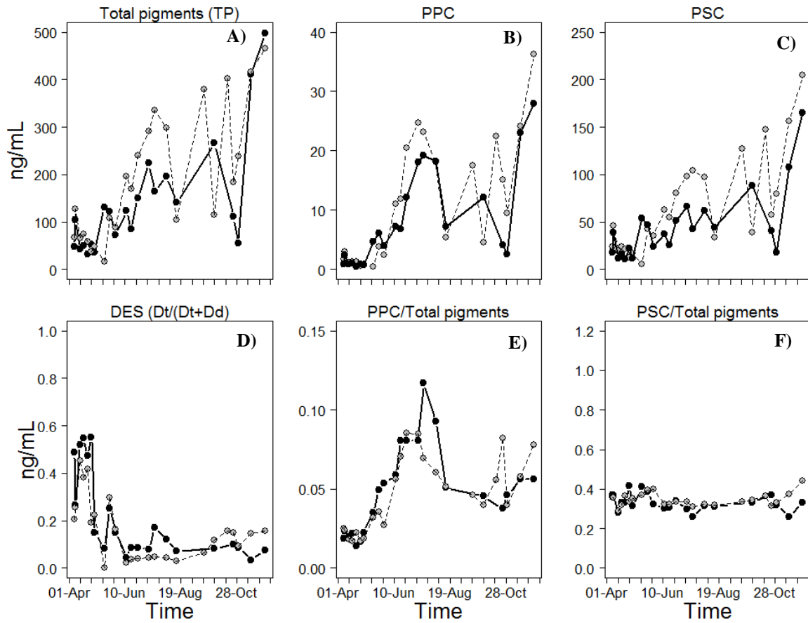
SM III-4: Temporal variations of A) Total Photosynthetic pigments (TP) , B) photoprotective carotenoids (PPC), C) Photosynthetic carotenoids (PSC), D) De-epoxidation state ( DES = Dt/(Dt+Dd) ); and the total pigments concentration weighted values of PPC (E) and PSC (F) for high tide samples (black circles and solid line) and low tide samples (gray circles and dashed line).
