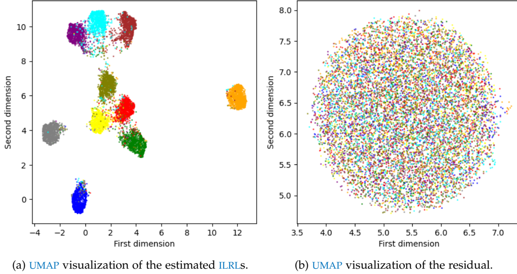
Figure 32: UMAP visualization of the MNIST testing data in the CDA ’s base space. The color indicates to which class a sample belongs: blue for 0, orange for 1, green for 2, red for 3, purple for 4, yellow for 5, gray for 6, brown for 7, olive for 8, and cyan for 9.
