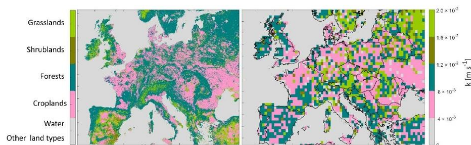
Figure 4. MODIS Land Cover Type, at a 500 \text{ m} \times 500 \text{ m} grid box (left panel), and interpolated mass transfer coefficient k on a horizontal resolution of 0.5^\circ \times 0.625^\circ grid box (right panel).
