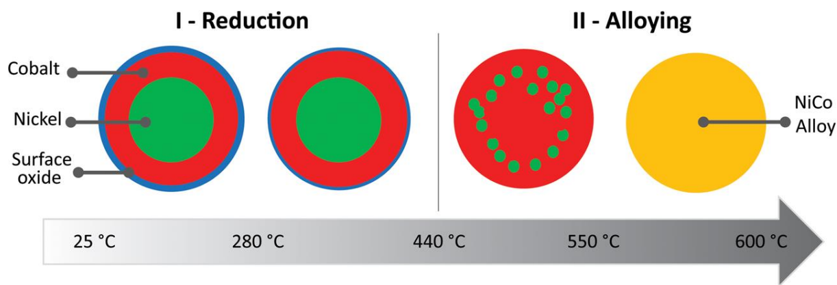
Figure 2. Evolution of the Ni-Co core-shell nanoparticles during heating under vacuum. Reproduced from 44 .
