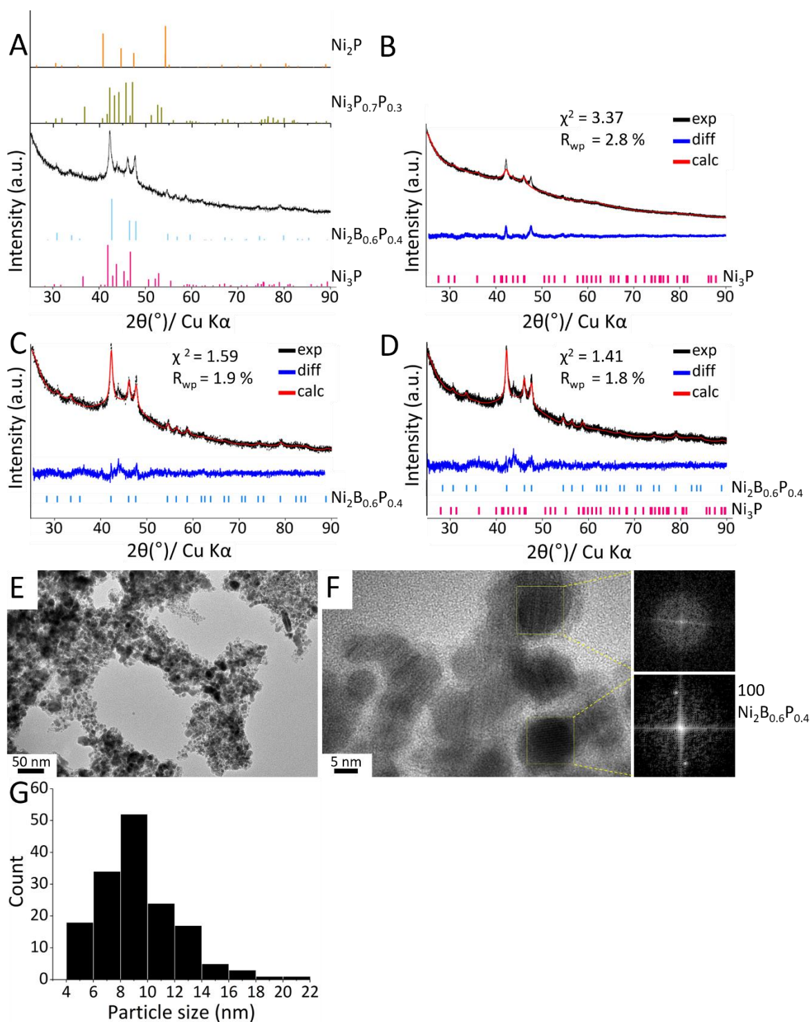
Figure 5. (A) Powder XRD pattern and corresponding Rietveld refinements performed by implementation of (B) \text{Ni}_3\text{P} , (C) \text{Ni}_2\text{B}_{0.6}\text{P}_{0.4} , (D) both \text{Ni}_3\text{P} and \text{Ni}_2\text{B}_{0.6}\text{P}_{0.4} . (E, F) TEM pictures including Fast Fourier Transform on selected particles, (G) Diagram of size distribution.
