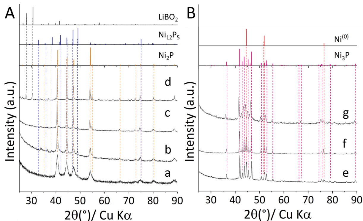
Figure 3. Powder XRD patterns of the products obtained by reacting (A) Ni 2 P nanoparticles and (B) Ni 3 P with NaBH 4 in a molten LiI:KI eutectic mixture syntheses: (a) initial Ni 2 P nanoparticles with minor amounts of Ni 12 P 5 , Ni 2 P:NaBH 4 atomic ratios of (b) 1:0.4 at 500 °C/1.5 h, (c) 1:1 at 500 °C/1.5 h, (d) 1:1 at 800 °C/1.5 h; (e) initial Ni 3 P nanoparticles, Ni 3 P:NaBH 4 atomic ratios of (f) 1:0.4 at 600 °C/3 h, (g) 1:1 at 600 °C/3 h.
