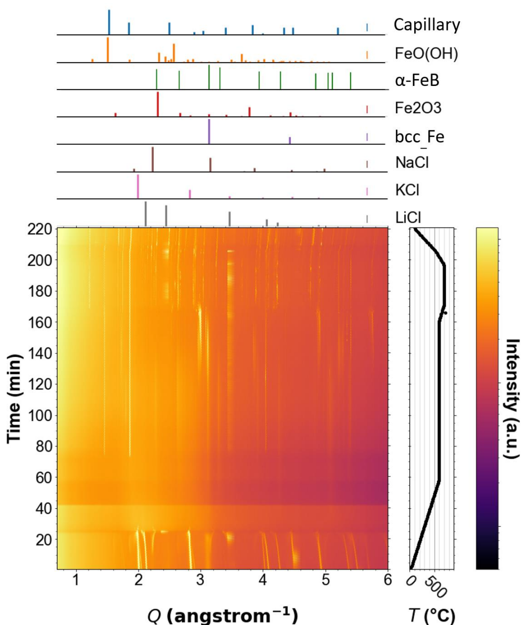
Figure 3. Synchrotron radiation-based in situ XRD diagrams recorded during the reaction of bcc-Fe nanoparticles with NaBH 4 (initial Fe:B = 1:1.3 at.) in the eutectic mixture LiCl:KCl.
