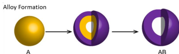
Figure 3. Mechanism of formation of an alloy at the nanoscale by reaction of a metal nanoparticle with atoms in solution. The void is represented by a white area. Adapted from 20 .
