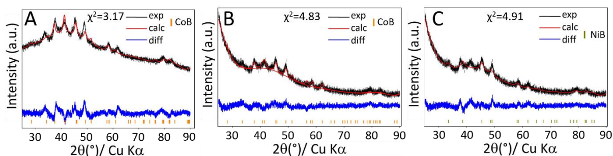
Figure S5-II. Powder XRD patterns and corresponding Rietveld refinements for the samples obtained by reacting Ni-Co nanoparticles with NaBH 4 (metal:B = 1:2.6 at.) at 600 °C for (A) 0.5 h by considering only CoB as constituent; for 1.5 h by considering (B) only CoB and (C) only NiB as references.
