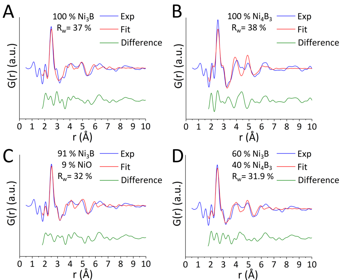
Figure S2-VII. PDFs of the amorphous intermediate to (A) \text{Ni}_3\text{B} fitted along the crystalline structure of \text{Ni}_3\text{B} , (B) \text{Ni}_4\text{B}_3 fitted along the crystalline structure \text{Ni}_4\text{B}_3 . PDF of the amorphous intermediate to \text{Ni}_3\text{B} fitted along the crystalline structure of (C) \text{Ni}_3\text{B} mixed with \text{NiO} , (D) \text{Ni}_3\text{B} mixed with \text{Ni}_4\text{B}_3 .
