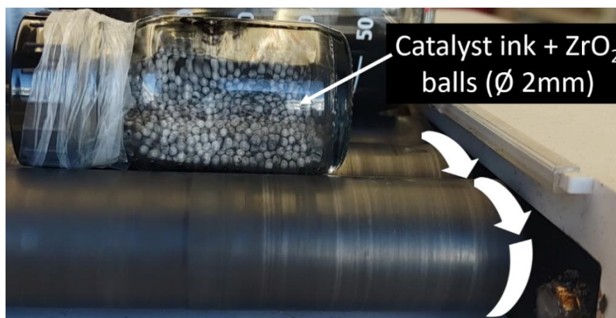
Figure 3. Experimental setup for ink dispersion studies by roll milling with zirconia balls.
