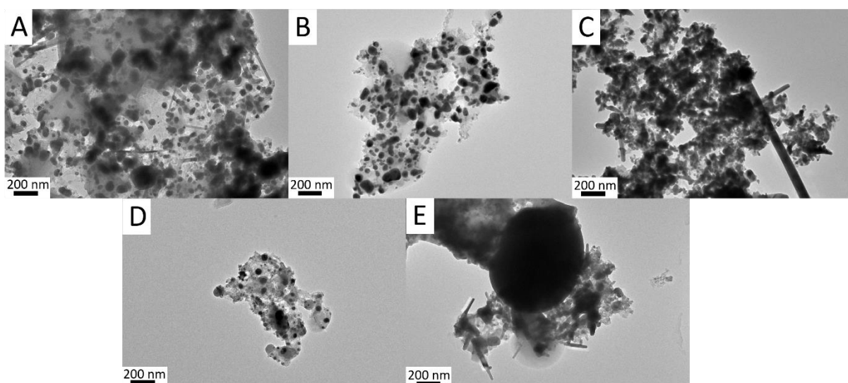
Figure S4-VI. TEM pictures of the products of reactions between nickel borides and red phosphorus into the molten eutectic mixture LiI:KI, from (A-C) Ni 3 B and (D-E) Ni 4 B 3 . Reaction conditions from Ni 3 B are (A) Ni 3 B:P red = 1:0.4 at 630 °C for 1.5 h, (B) Ni 3 B:P red = 1:0.6 at 630 °C for 1.5 h, (C) Ni 3 B:P red = 1:1 at 450 °C for 3 h. Reaction conditions from Ni 4 B 3 are (D) Ni 4 B 3 :P red = 1:0.5 at 630 °C for 1.5 h, (E) Ni 4 B 3 :P red = 1:0.94 at 630 °C for 1.5 h.
