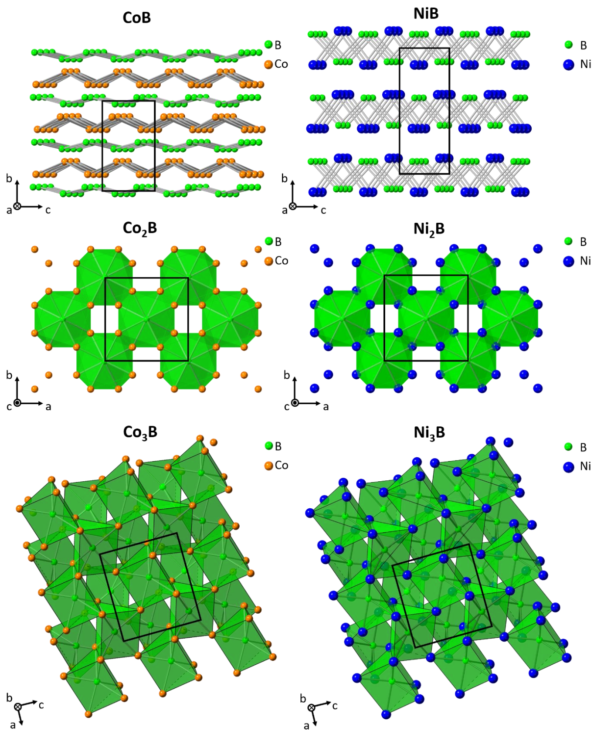
Figure 1. Schemes of the crystal structures of \text{Co}_x\text{B} and \text{Ni}_x\text{B} , for x= 1, 2 and 3 .
