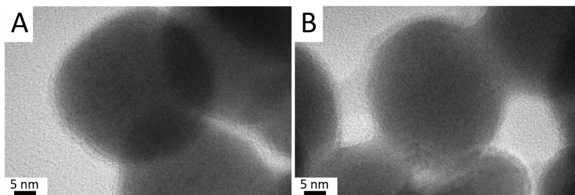
Figure S2-VIII. HRTEM images of \text{Ni}_3\text{B} nanoparticles obtained by synthesis at 475\text{ }^\circ\text{C} for 1.5 h: of (A) single amorphous nanoparticle, (B) coalesced amorphous nanoparticles.
