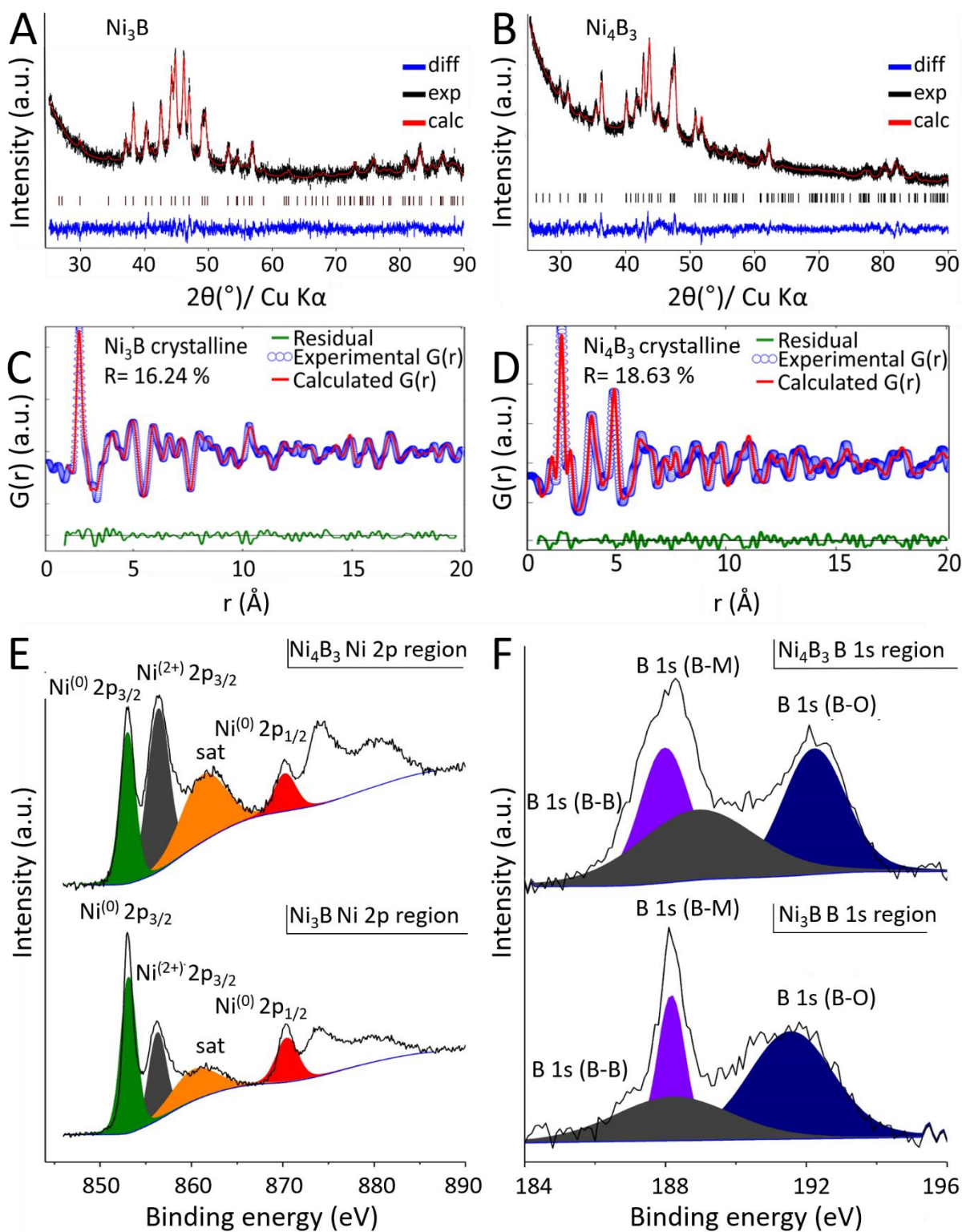
Figure 3. XRD patterns with corresponding Rietveld refinements of (A) \text{Ni}_3\text{B} and (B) \text{Ni}_4\text{B}_3 nanocrystals. Pair distribution functions of (C) \text{Ni}_3\text{B} and (D) \text{Ni}_4\text{B}_3 nanocrystals fitted along the corresponding crystal structures. XPS of \text{Ni}_3\text{B} and \text{Ni}_4\text{B}_3 in (E) Ni 2p (F) B 1s region.
