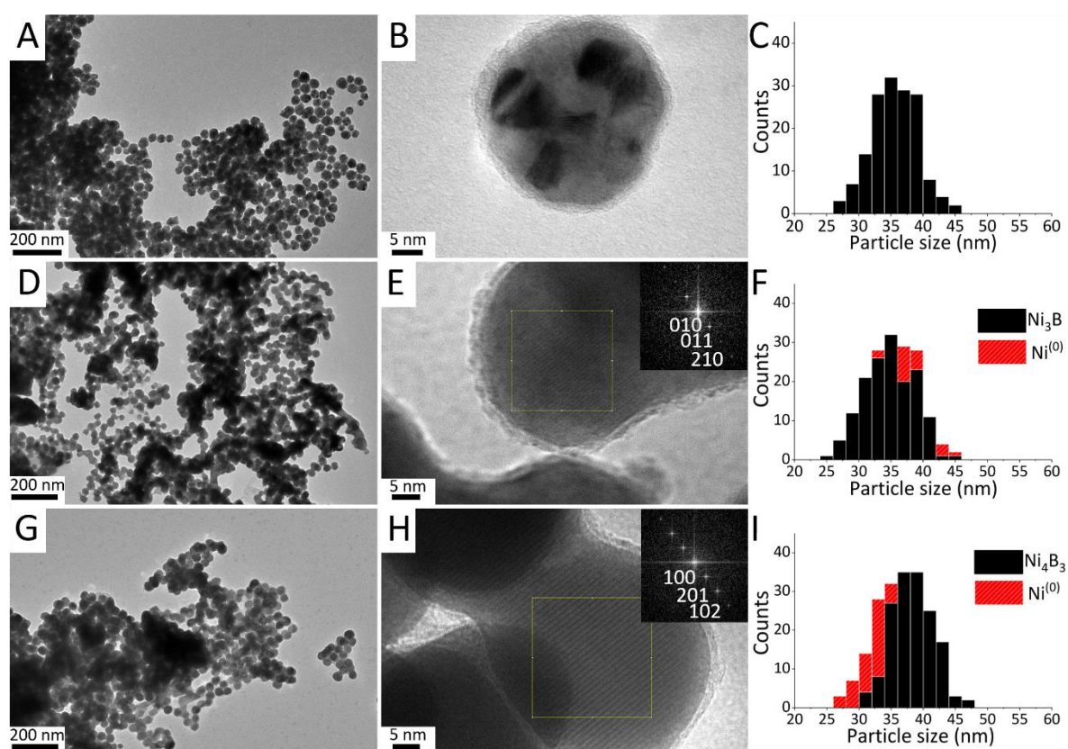
Figure 2. TEM study of (A-C) \text{Ni}^{(0)} nanoparticles, (D-F) \text{Ni}_3\text{B} nanocrystals and (G-I) \text{Ni}_4\text{B}_3 nanoparticles: (A, D, G) TEM images; (B, E, H) HRTEM images with FFTs of the squared areas, indexed along the corresponding crystal structures of borides; (C, F, I) particle size
