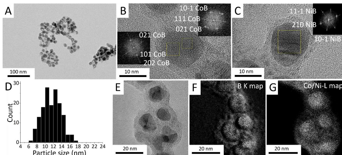
Figure 6. Morphology and composition study of bimetallic boride nanoparticles obtained by reacting Ni-Co nanoparticles with \text{NaBH}_4 (metal:B = 1:2.6 at.) at 600 °C for 0.5 h in molten LiI:KI. (A) TEM and (B, C) HRTEM images with corresponding FFTs. (D) Corresponding size distribution. (E) TEM and corresponding EFTEM images at the (F) B-K and (G) Co/Ni-L edges.
