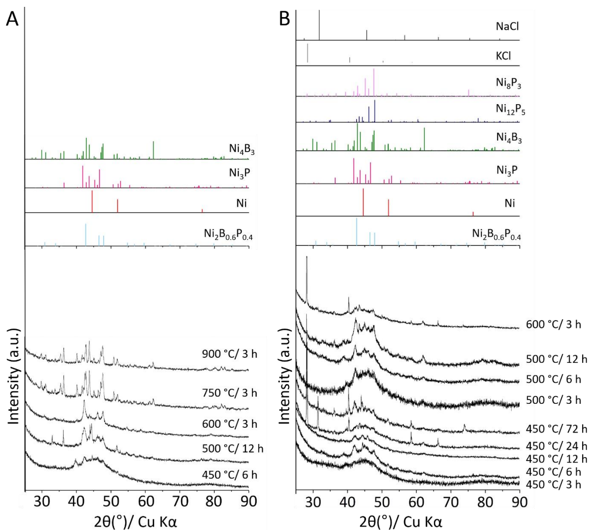
Figure S4-VII. Powder XRD patterns of the powders obtained from the reaction of \text{NiCl}_2 , \text{NaBH}_4 and \text{P}_{\text{red}} in the molten eutectic mixture \text{LiCl}:\text{KCl} performed to target reported Ni-B-P ternary phases using Ni:B:P atomic ratio of (A) 3:6:0.7 and (B) 2:4:0.4. Some KCl and NaCl remains in some powder due to inefficient washing.
