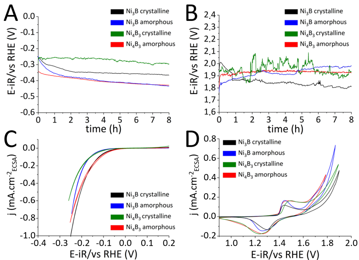
Figure S3-II. Chronopotentiometry (CP) for 8 h recorded at a current density of |10| \text{ mA}\cdot\text{cm}^{-2} on a 1 \text{ cm}^2 carbon paper working electrode during (A) HER, (B) OER. Surface area normalized CV curves at the 30 th cycle during (C) HER, (D) OER.
