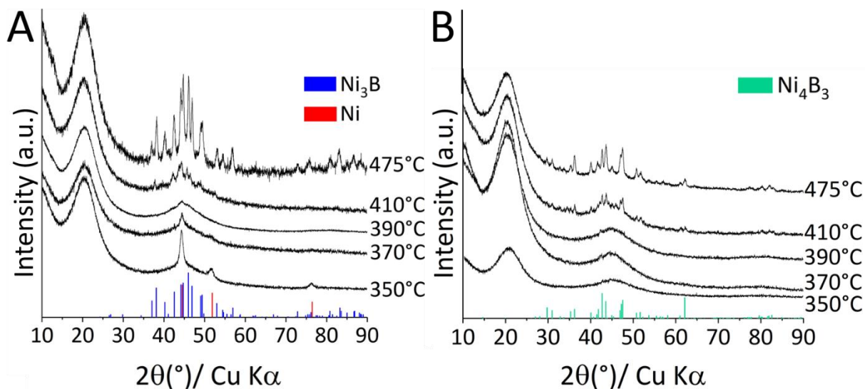
Figure S2-V. Ex situ powder XRD patterns of samples retrieved at different temperatures for 1.5 h plateaus from the (A) \text{Ni}_3\text{B} and (B) \text{Ni}_4\text{B}_3 reaction mixtures.
