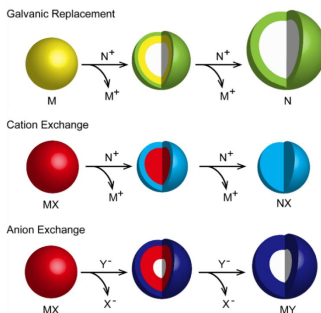
Figure 1. Schemes of exchange reactions in nanomaterials: galvanic replacement, cation exchange, anion exchange. The voids are represented by white areas. Adapted from 20 .
