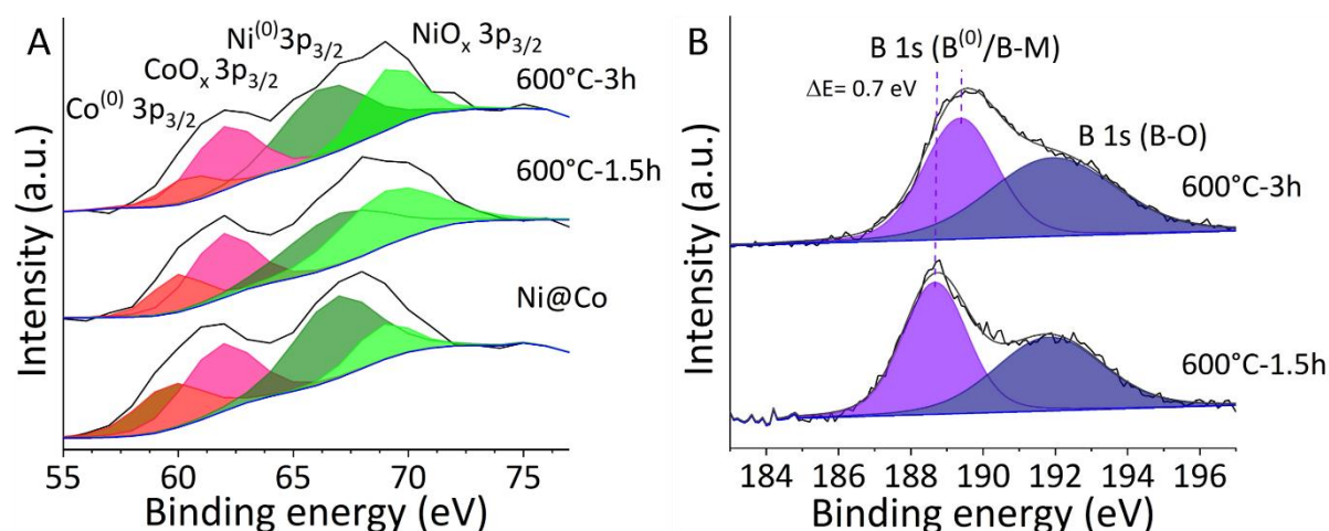
Figure 9. XPS spectra of Ni-Co nanoparticles and the products of their reaction with \text{NaBH}_4 in molten \text{LiI}:\text{KI} for a metal:B ratio of 1:2.6 at. at 600 °C for 1.5 and 3 h: (A) Ni, Co 3p region and (B) B 1s region.
