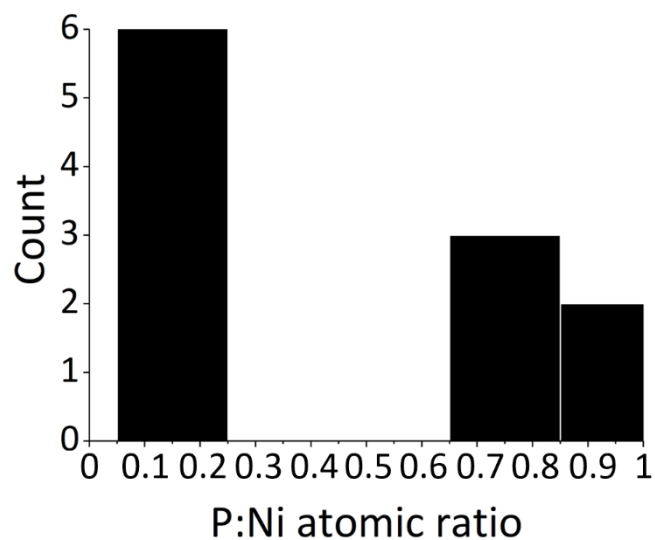
Figure S4-VIII. P:Ni atomic ratio distribution observed by STEM-EDX on 11 single particles from the sample obtained by the reaction of \text{NiCl}_2 , \text{NaBH}_4 and \text{P}_{\text{red}} (2:4:0.4 at. ratio) at 600 °C for 3h in the molten eutectic mixture LiCl:KCl.
