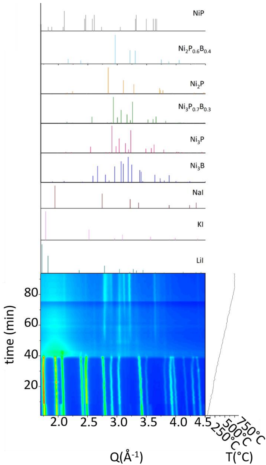
Figure S4-III. In situ XRD diagrams recorded during the reaction of \text{Ni}_3\text{B} with red phosphorus with the ratio \text{Ni}_3\text{B}:\text{P}_{\text{red}} = 1:0.7 at. in the eutectic mixture LiI:KI.
