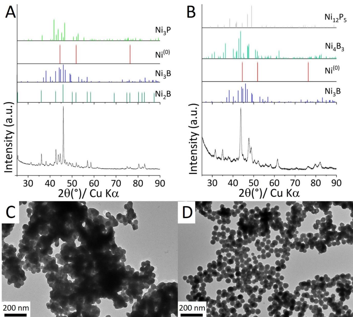
Figure S2-IX. Syntheses of borides nanoparticles without molten salts. XRD pattern and corresponding TEM images of (A, C) \text{Ni}_3\text{B} mixture, (B, D) \text{Ni}_4\text{B}_3 mixture.
