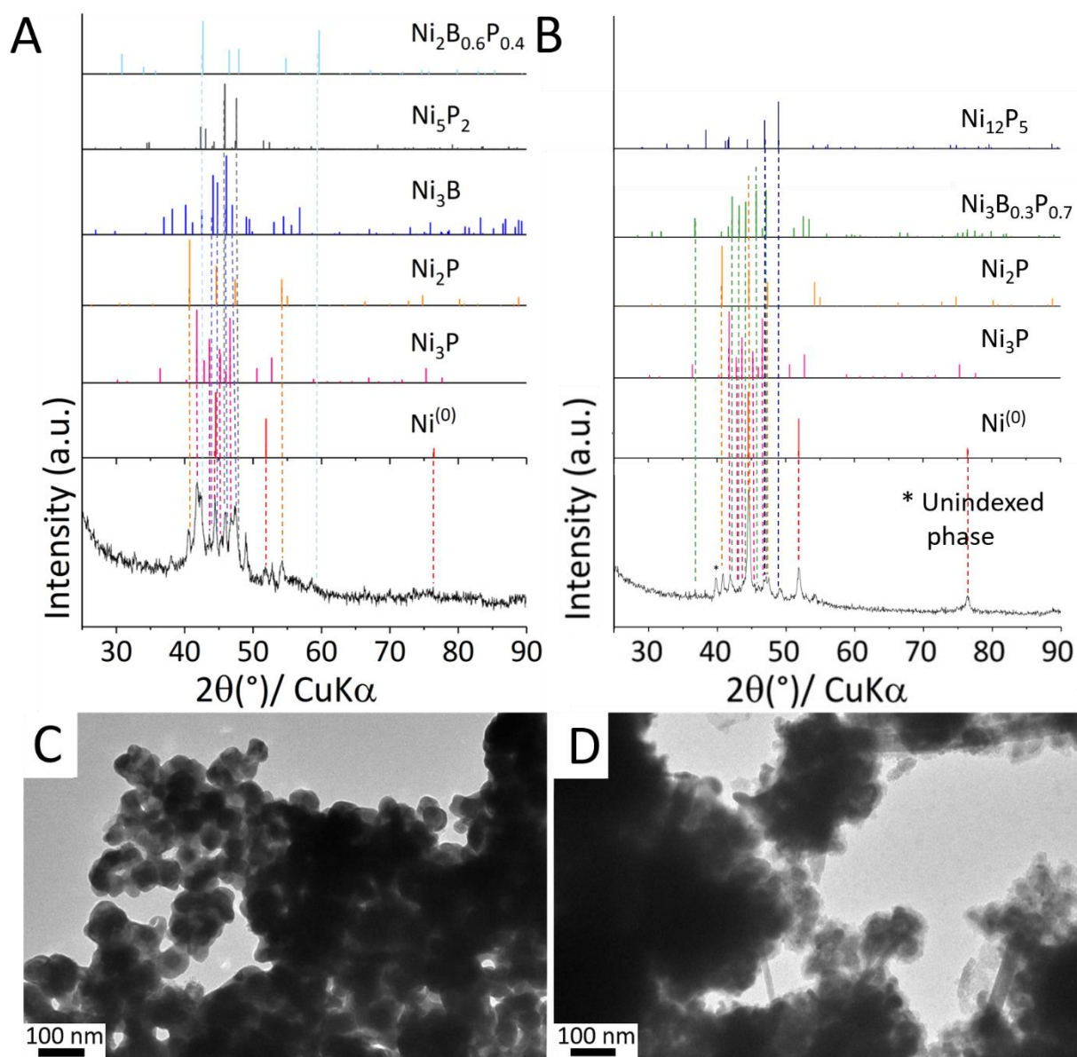
Figure 2. Powder XRD patterns of the samples prepared in the LiI:KI eutectic mixture at 475 °C for 1.5 h with initial Ni:B:P ratios (A) 2:1:0.4 and (B) 3:0.6:0.7. Corresponding TEM pictures in (C) and (D), respectively.
