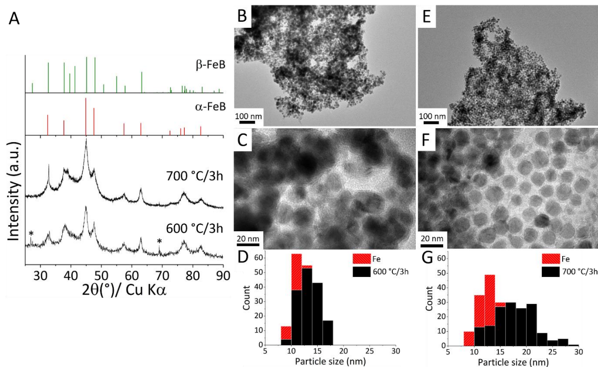
Figure 2. (A) Powder XRD patterns, (B, C, E, F) TEM images and (D, G) corresponding size distributions for the products obtained by reacting HDA-derived Fe nanoparticles with \text{NaBH}_4 (initial Fe:B atomic ratio 1:1.3) in the molten eutectic mixture LiCl:KCl. The products were obtained by reaction at (B-D) 600 and 700 °C (E-G). *: unindexed peaks.
