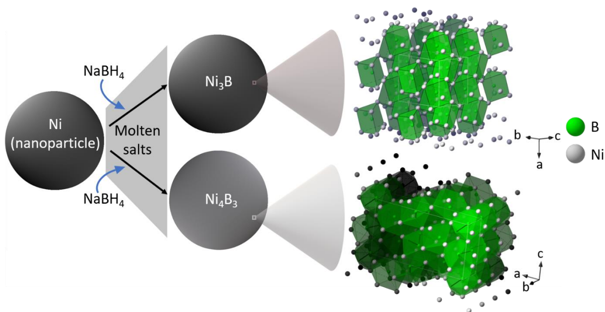
Figure 1. Schematic mechanisms of the syntheses of Ni 3 B and Ni 4 B 3 nanocrystals, with the corresponding crystal structures.
