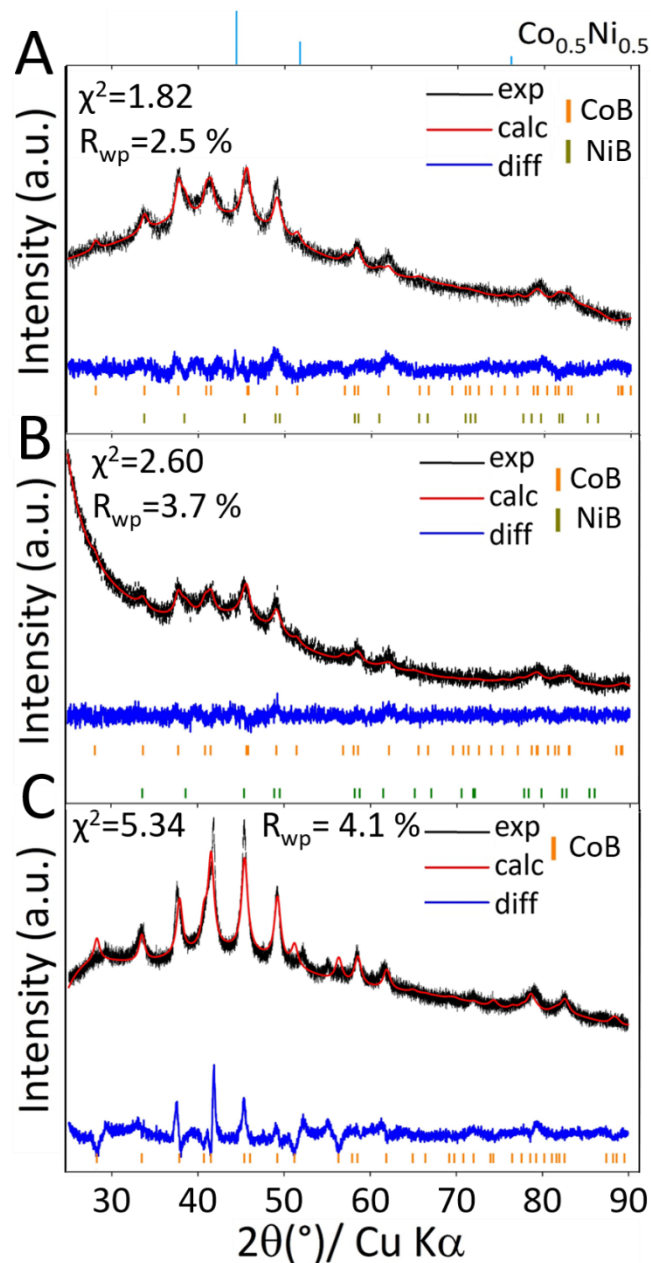
Figure 5. Rietveld refinements of the XRD pattern of powders obtained by reacting Ni-Co nanoparticles with \text{NaBH}_4 for metal:B = 1:2.6 at. in LiI:KI at 600 °C for (A) 0.5, (B) 1.5, and (C) 3 h. The phase indexed \text{Co}_{0.5}\text{Ni}_{0.5} in (A) was not accounted for in the refinement, as adding this third phase led to misinterpretation due to a large number of variables involved in the fit.
