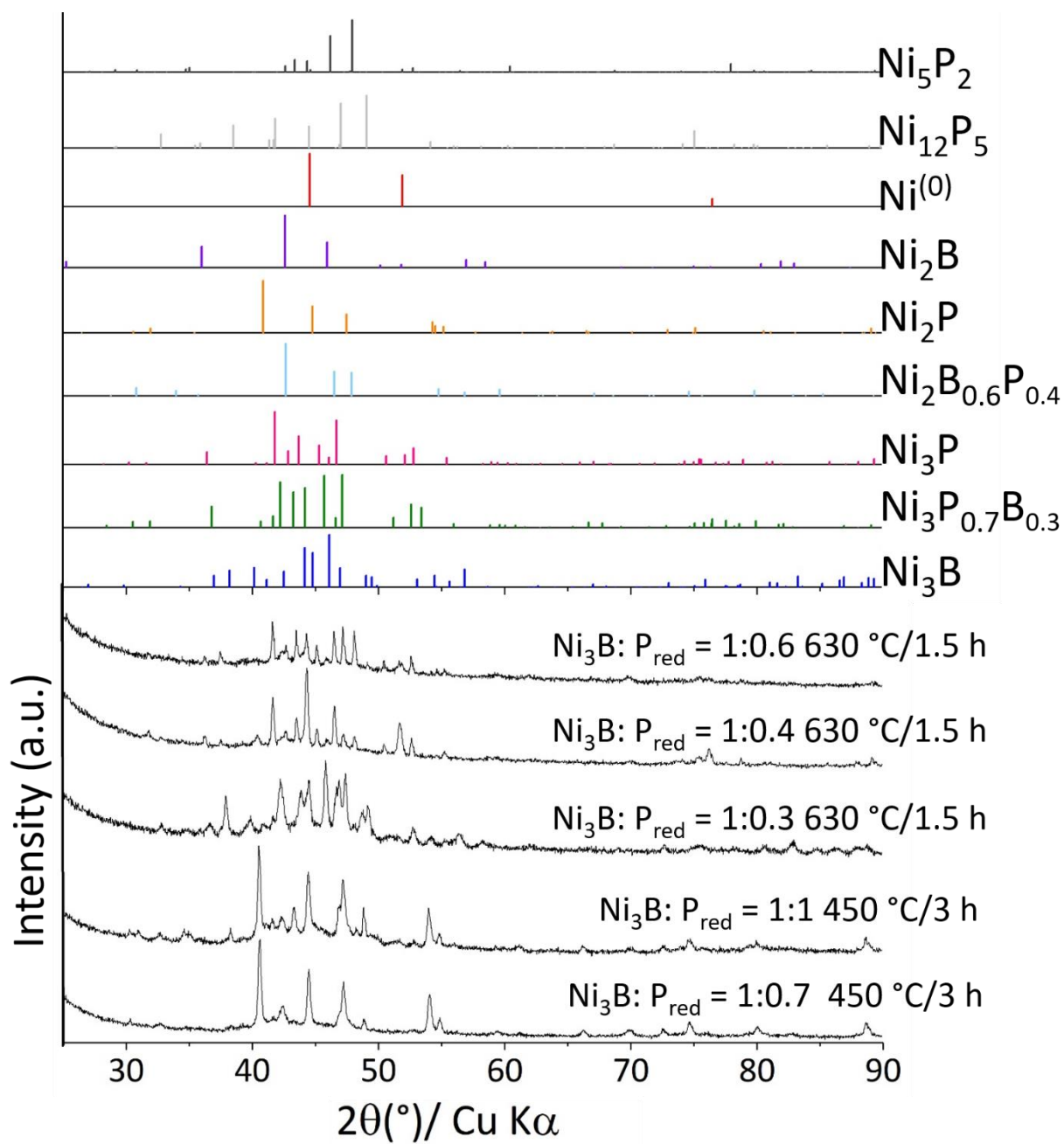
Figure S4-IV. Powder XRD patterns of the products obtained from the reaction of red phosphorus with \text{Ni}_3\text{B} nanoparticles in the molten eutectic mixture LiI:KI. and (B) nanoparticles.
