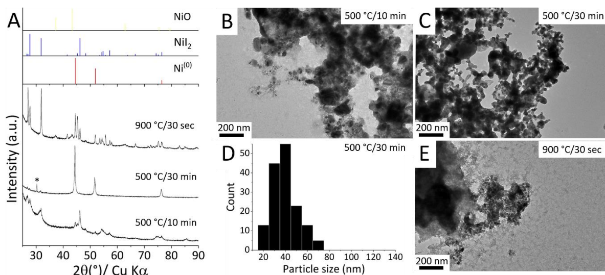
Figure 3. (A) XRD pattern and (B-E) TEM images of the powders obtained from mixtures NiI 2 :NaH (1:5 at.) reacted in the molten eutectic mixture LiI:KI heated by induction.
