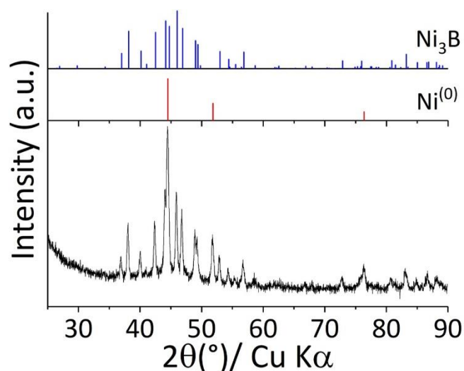
Figure S2-X. Powder XRD pattern of the sample obtained for B: Ni of 2.6 at 475 °C/ 1.5 h in LiI-KI (58:42 mass.).
