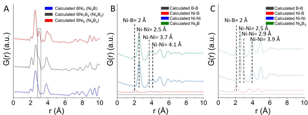
Figure 8. (A) Calculated PDF of the isolated polyhedra consisting of \text{Ni}_3\text{B} ( \text{BNi}_7 ) and \text{Ni}_4\text{B}_3 ( \text{BNi}_7\text{B}_2 , \text{BNi}_9 ). The rectangle highlights the 2.9 \text{ \AA} peak unobserved in the \text{BNi}_7 coordination of \text{Ni}_3\text{B} . Calculated PDF of the (B) \text{Ni}_3\text{B} and (C) \text{Ni}_4\text{B}_3 structures in a range of 9 \text{ \AA} and assignment of the contributions of B-B, Ni-B and Ni-Ni distances.
