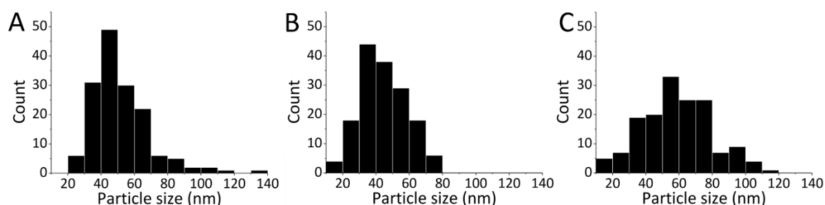
Figure S-I. Size distributions of nickel particles obtained by the reaction of \text{NiCl}_2 with \text{NaH} in molten \text{LiI}:\text{KI} (58:42 mass.) by induction heating at (A) 350 °C for 20 min, (B) 500 °C 30 s. and (C) 600 °C for 30 s.
