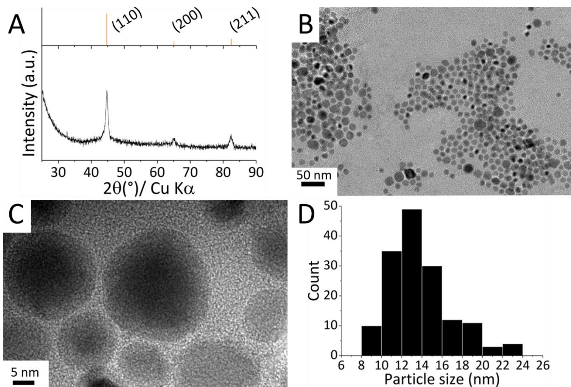
Figure 1. Crystalline bcc-Fe nanoparticles synthesized by adapting the method reported by L.-M. Lacroix et al. 18 . (A) Powder XRD pattern indexed along the bcc-Fe. (B) TEM and (C) HRTEM images showing spherical nanoparticles, with (D) the corresponding size distribution (D).
