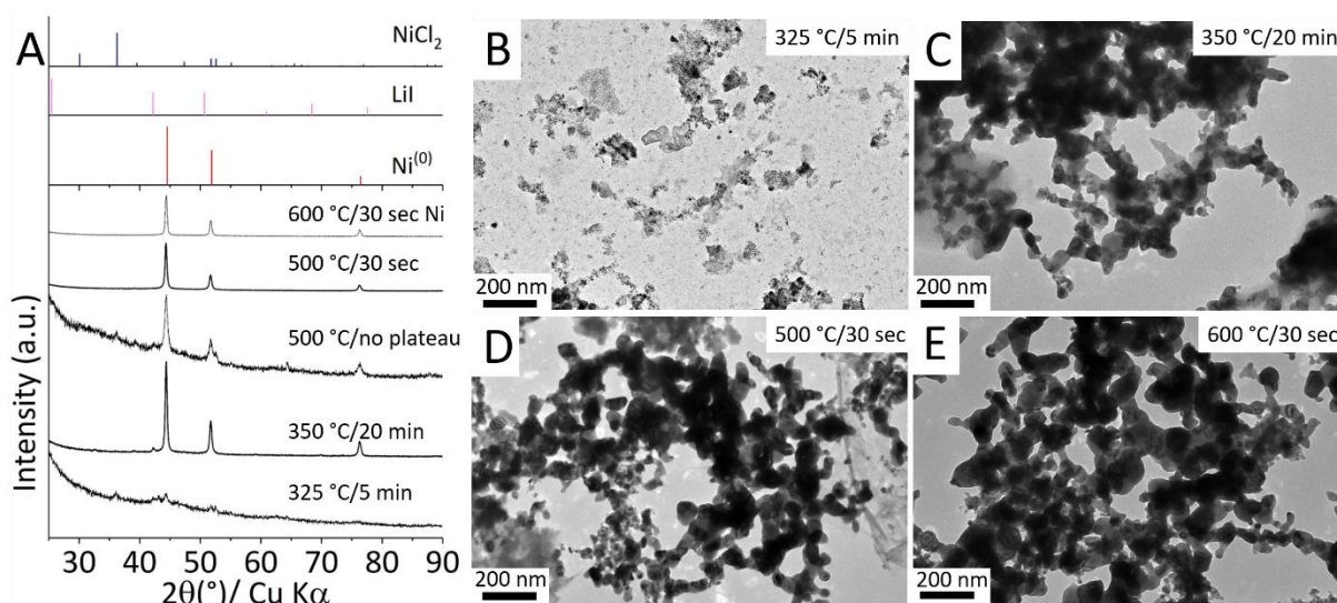
Figure 2. (A) XRD patterns and (B-E) TEM images of the powders obtained from mixtures NiCl 2 :NaH (1:5 at.) reacted in the molten eutectic mixture LiI:KI heated by induction.
