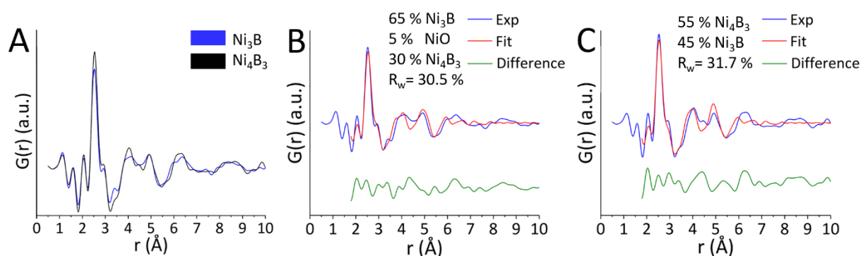
Figure 7. (A) Ex situ PDFs of the amorphous intermediates retrieved in the course of the syntheses of Ni 3 B and Ni 4 B 3 . (B) PDF of Ni 3 B refined as a mixture of Ni 3 B, Ni 4 B 3 and NiO crystal structures. (C) PDF of Ni 4 B 3 refined as a mixture of Ni 4 B 3 and Ni 3 B.
