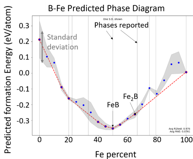
Figure S6-II. Predicted phase diagram at 0 K of Fe-B from the machine learning tool Matlearn 15 . The red dotted line corresponds to the convex hull. The blue point are phases predicted and the continuous vertical lines correspond to the phases reported.
