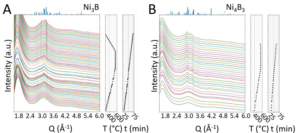
Figure S2-IV. In situ powder X-ray diagrams in total X-ray scattering configuration for (A) \text{Ni}_3\text{B} and (B) \text{Ni}_4\text{B}_3 mixtures.
