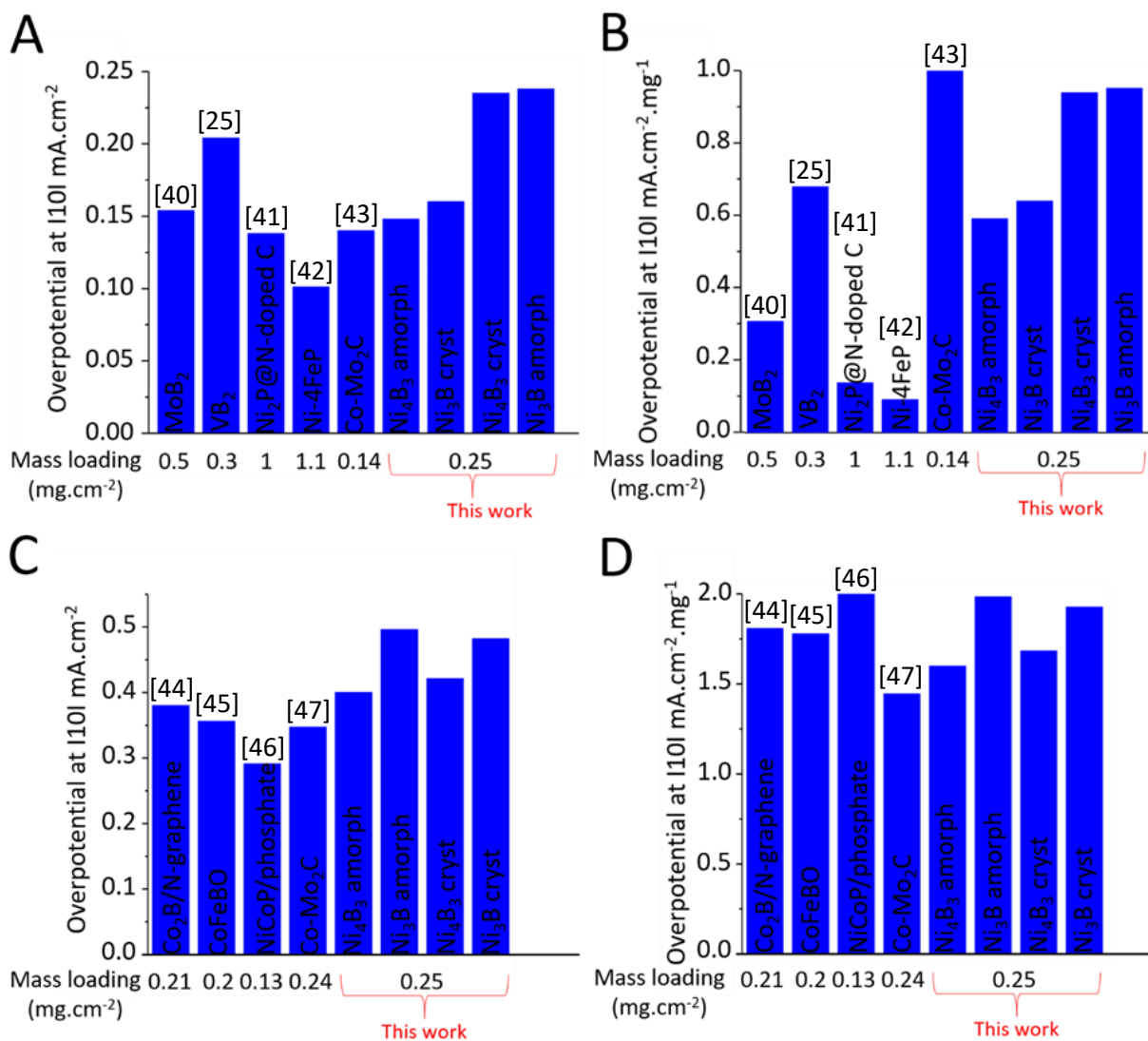
Figure S3-III. Overpotentials and mass normalized overpotentials measured at 10 mA cm -2 in (A-B) HER and (C-D) OER conditions, for selected transition metal borides, phosphides and carbides from the literature and from the present work. Data reported for (A-B) HER and (C-D) OER correspond to 0.5 M H 2 SO 4 and 0.1 M KOH electrolytes, respectively.
