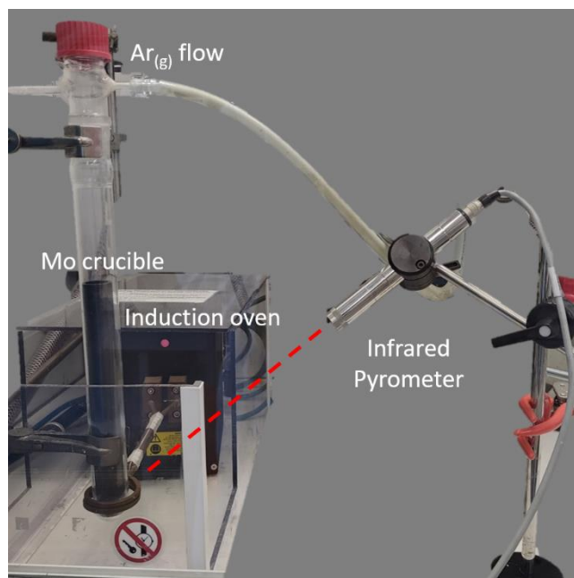
Figure 1: Experimental setup for induction heating. The temperature is measured by infrared pyrometry.
