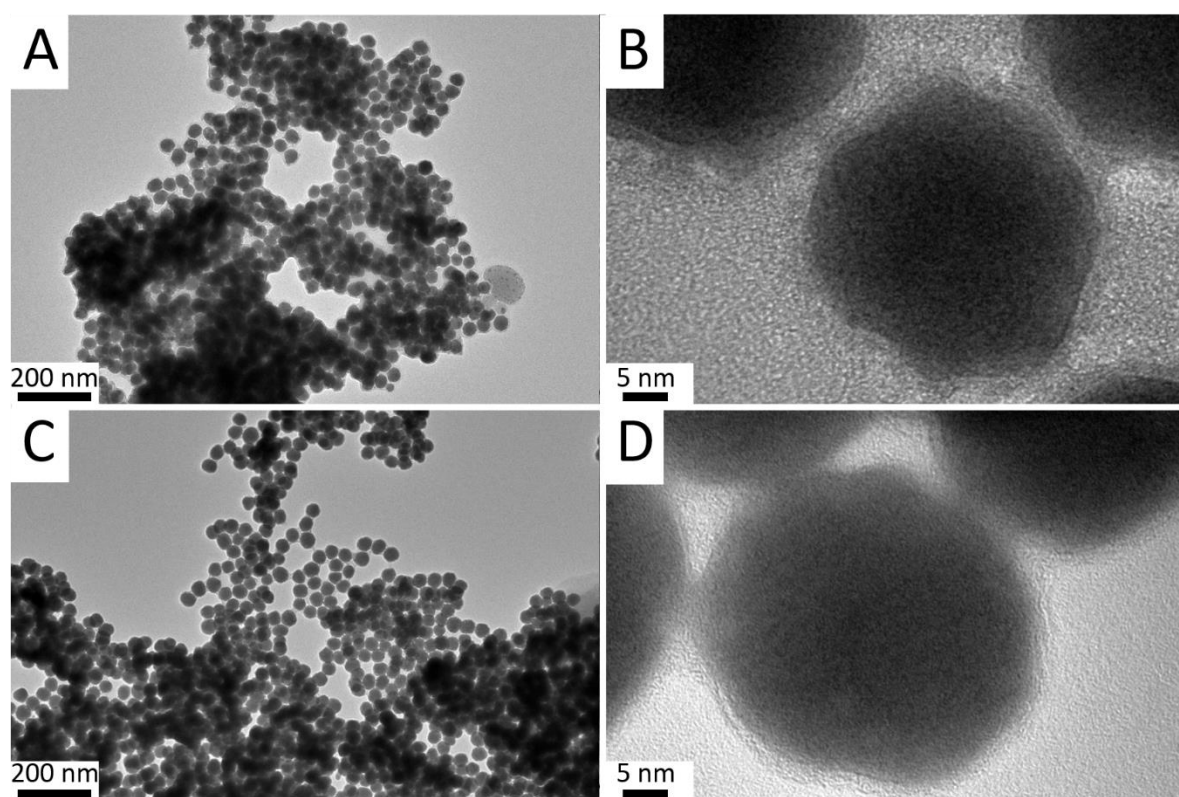
Figure 6. TEM pictures of the amorphous nanoparticles formed during the synthesis of (A, B) Ni 3 B and (C, D) Ni 4 B 3 nanocrystals. (A, C) Low and (B, D) high magnification images.
