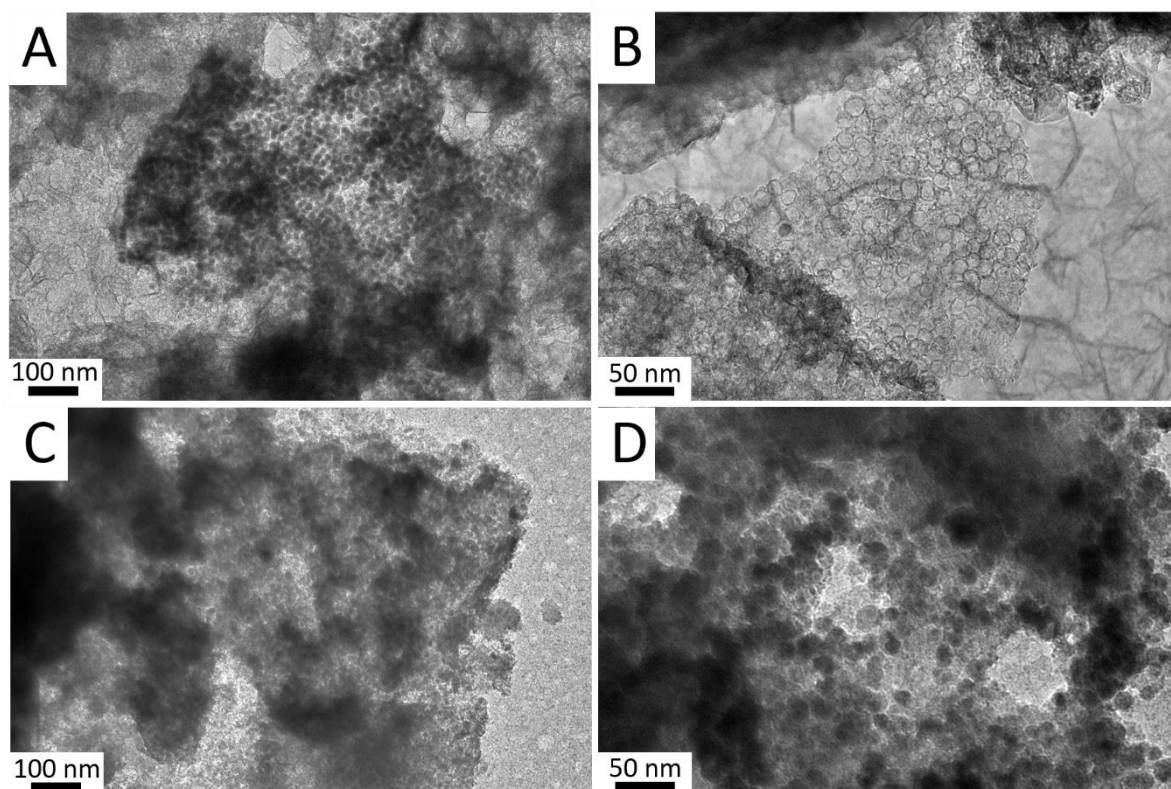
Figure S6-V. TEM images of \alpha -FeB nanoparticles synthesized at (A, B) 600 °C for 3 h, (C, D) 700 °C for 3 h by dispersion of the nanoparticles into methanol before deposition on a TEM carbon-coated copper grid and drying under air.
