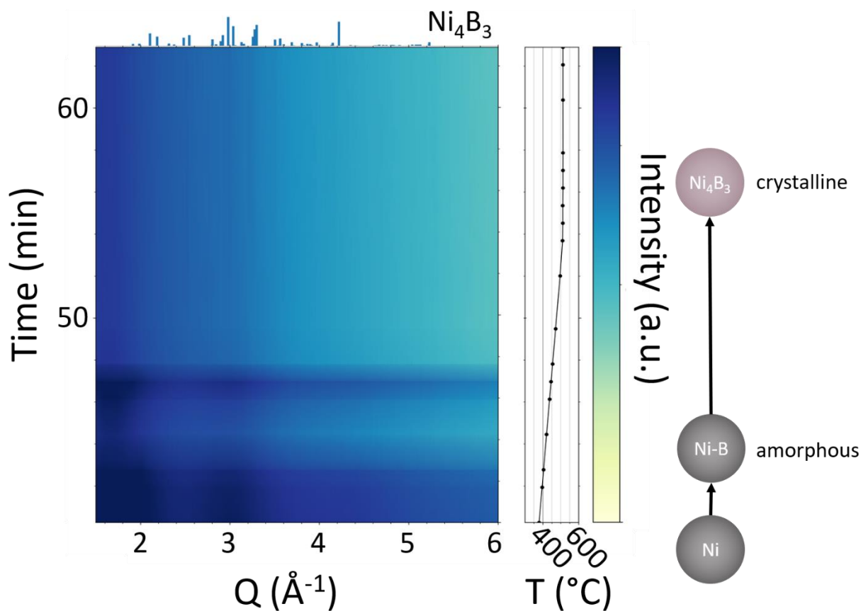
Figure S2-III. In situ XRD diagrams recorded during the synthesis of \text{Ni}_4\text{B}_3 nanocrystals after melting of the eutectic salt mixture.
