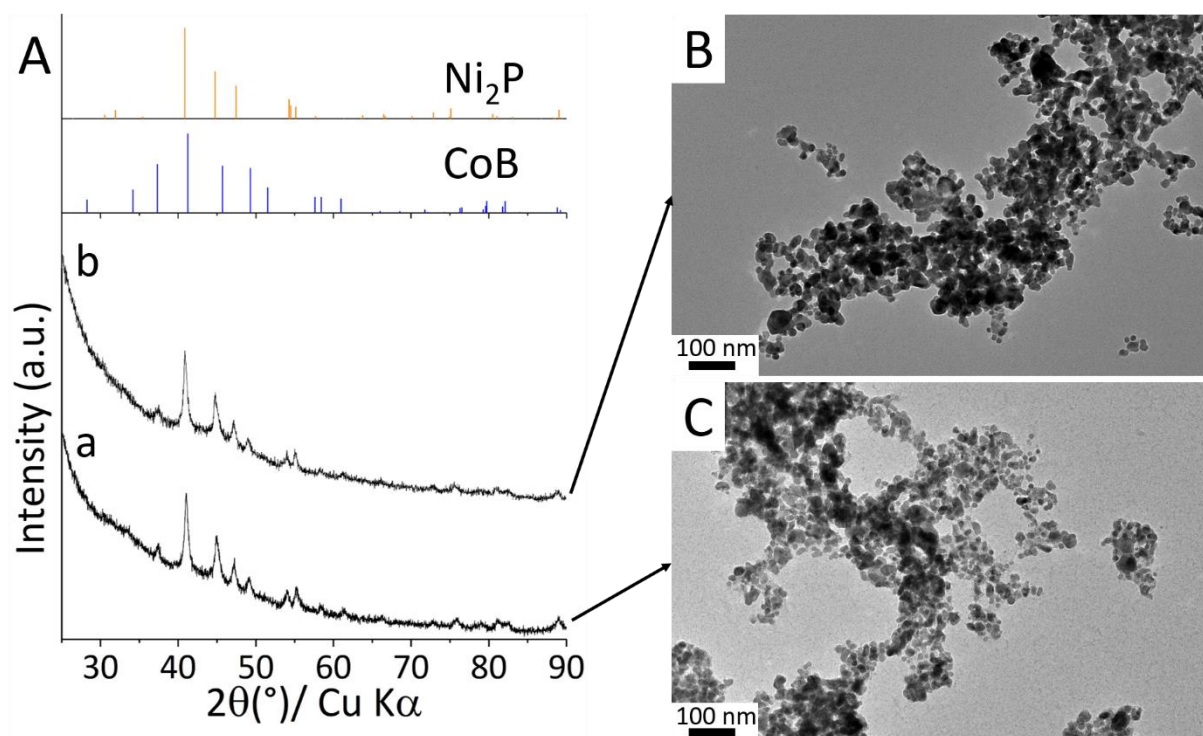
Figure S5-I. (A) Powder XRD patterns and (B, C) corresponding TEM images of nanoparticles obtained with the reagent ratio Metal:B = 1:1.3 at 600 °C for 3 h in molten (a) LiI:KI (58:42 mass.), (b) LiCl:KCl (44:56 mass.).
