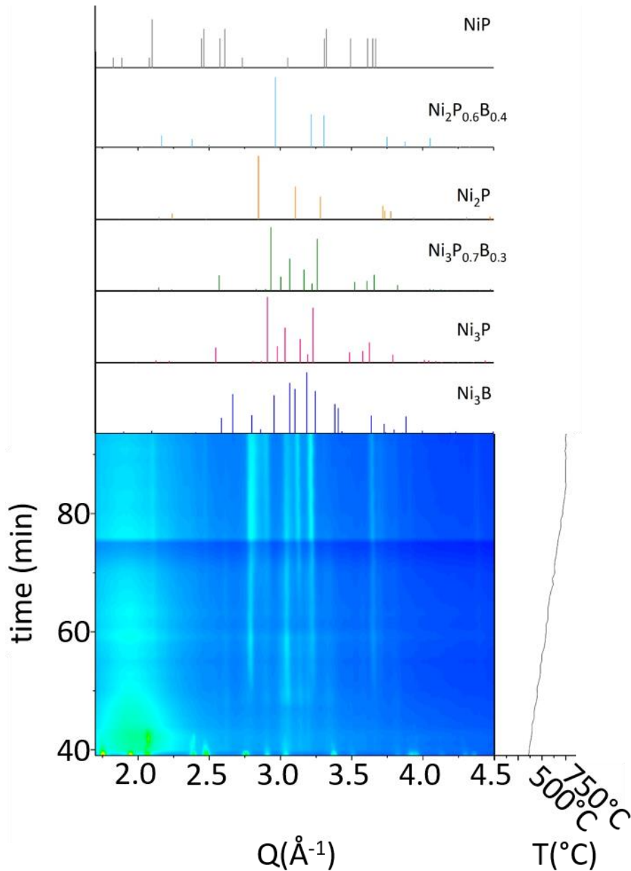
Figure 4. Synchrotron in situ XRD diagrams recorded during heating of a reaction mixture containing \text{Ni}_3\text{B} nanoparticles and red phosphorus in proportions \text{Ni}_3\text{B}:\text{P}_{\text{red}} = 1:0.7 at. in the molten eutectic mixture LiI:KI.
