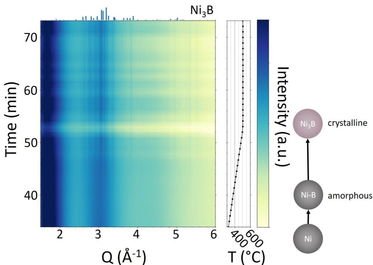
Figure 5. In situ XRD diagrams recorded during the synthesis of Ni 3 B nanocrystals after melting of the eutectic salt mixture.
