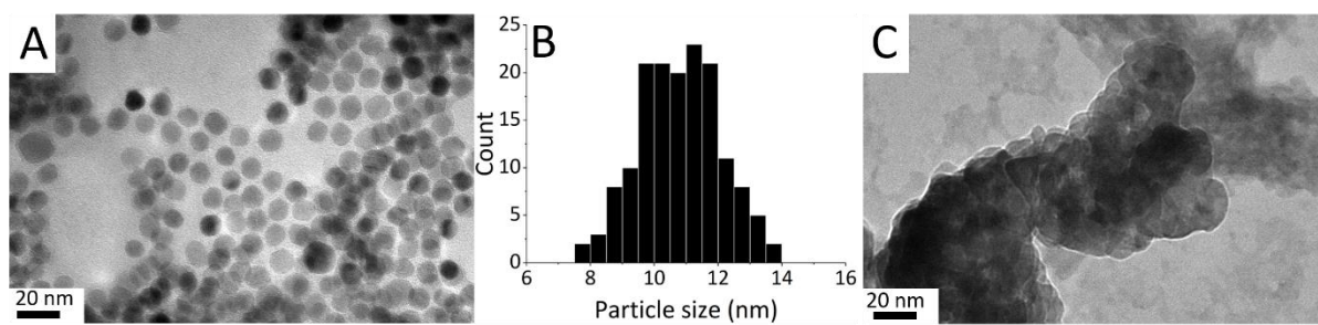
Figure S4-II. TEM image of (A) Ni 2 P nanoparticles with (B) corresponding size distribution. (C) TEM image of a Ni 3 P sample.
