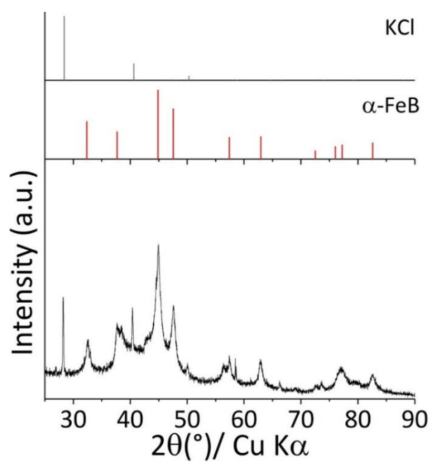
Figure S6-VI. Powder XRD pattern of the particles synthesized with Fe:B = 2:1.3 at. ratio at 700 °C for 3 h in molten LiCl:KCl.
