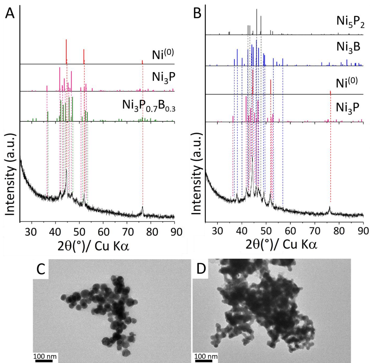
Figure S4-I. Powder XRD patterns of sample prepared in the LiI:KI eutectic mixture at 475 °C for 1.5 h with initial Ni:B:TOP ratios (A) 2:1:0.4 and (B) 3:0.6:0.7. Corresponding TEM pictures in (C) and (D), respectively.
