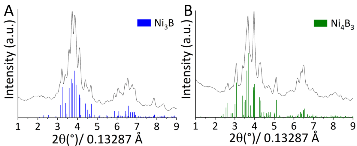
Figure S2-I. Powder XRD diagrams of (A) \text{Ni}_3\text{B} and (B) \text{Ni}_4\text{B}_3 nanocrystals acquired in total X-ray scattering configuration by using synchrotron-based radiation, with wavelength 0.13287 \text{ \AA} .
