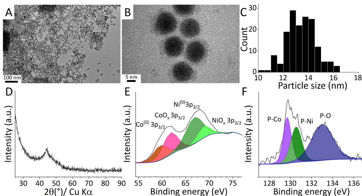
Figure 3. Ni-Co core-shell nanoparticles. (A) TEM image, (B) high magnification TEM image showing no local order and (C) size distribution of the particles, (D) powder XRD pattern, (E) XPS in the Co/Ni 3p_{3/2} region, (F) XPS in the P 2p region.
