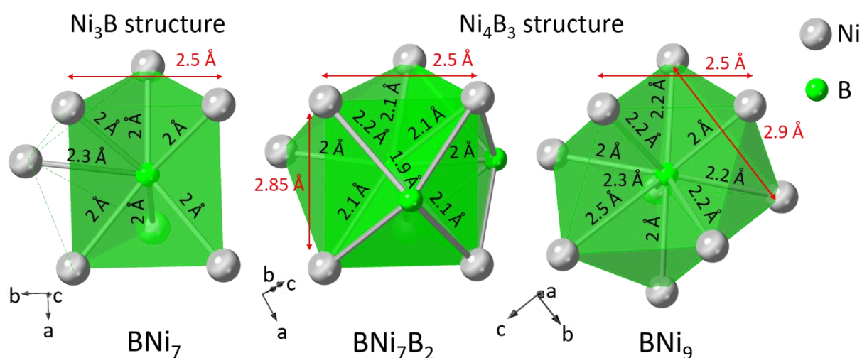
Figure 4. Single boron polyhedra constituting the \text{Ni}_3\text{B} and \text{Ni}_4\text{B}_3 crystal structures. The red marks indicate the distances between nickel atoms not directly engaged in a binding.
