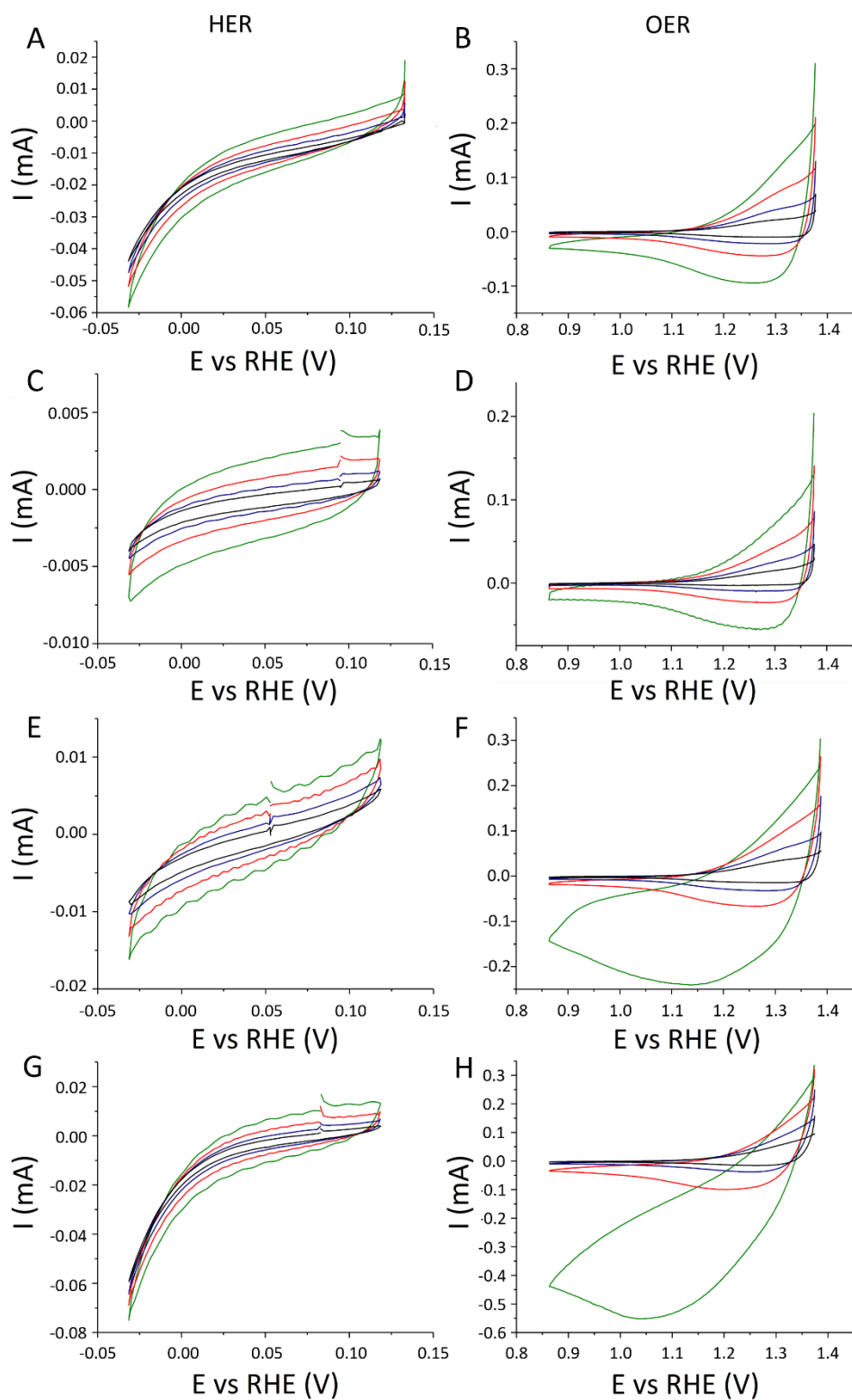
Figure S3-IV. Cyclic voltammety curves recorded at scan rates of 2.5, 5, 10, 20 \text{mV s}^{-1} in a low faradic region in HER and OER to estimate the double layer capacitance ( C_{\text{DL}} ). (A, B) \text{Ni}_3\text{B} crystalline, (C, D) \text{Ni}_3\text{B} amorphous, (E, F) \text{Ni}_4\text{B}_3 crystalline, (G, H) \text{Ni}_4\text{B}_3 amorphous.
