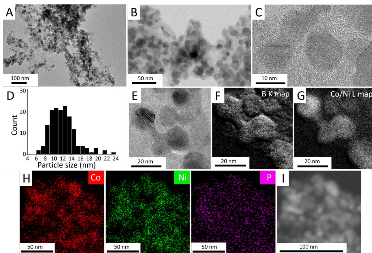
Figure 8. Transmission electron microscopy study of Ni-Co-B nanoparticles obtained by reacting Ni-Co nanoparticles with \text{NaBH}_4 (metal:B = 1:2.6 at.) at 600 °C for 1.5 h in molten LiI:KI. (A-C) TEM and HRTEM images and (D) corresponding size distribution. (E) TEM and corresponding EFTEM images at the (F) B-K and (G) Co-L edge. (H) STEM-EDS chemical maps of Co, Ni and P with (I) the corresponding TEM image.
