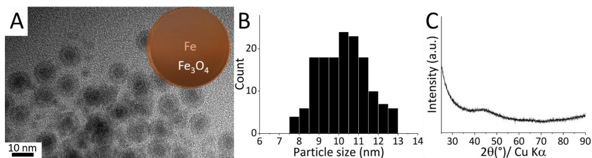
Figure S6-I. Fe nanoparticles synthesized by colloidal chemistry 13 using Fe(CO) 8 as precursor. (A) TEM image and the corresponding scheme of the core-shell Fe-Fe 3 O 4 structure, corresponding (B) size distribution and (C) powder XRD pattern.
