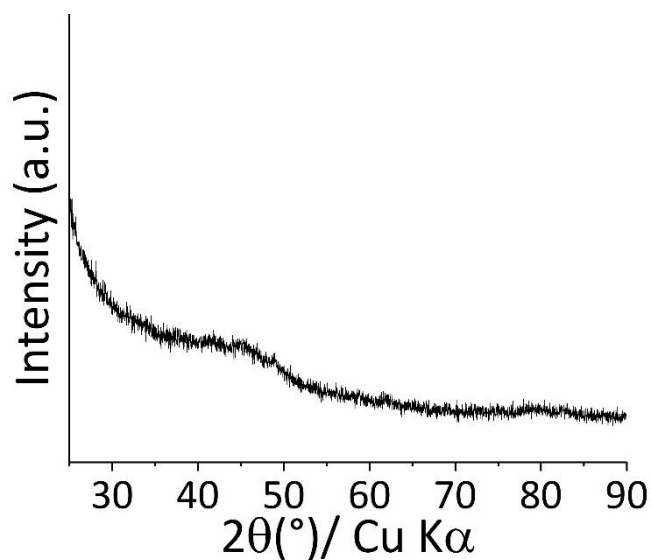
Figure S5-IV. XRD pattern of the powder obtained by reacting Ni-Co nanoparticles with NaBH 4 (metal:B = 1:2.6 at.) at 450 °C for 6 h in LiI/KI.
