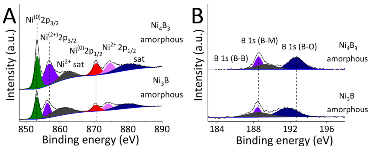
Figure S2-VI. XPS of amorphous \text{Ni}_3\text{B} and \text{Ni}_4\text{B}_3 nanoparticles: (A) Ni 2p region, (B) B 1s region.
