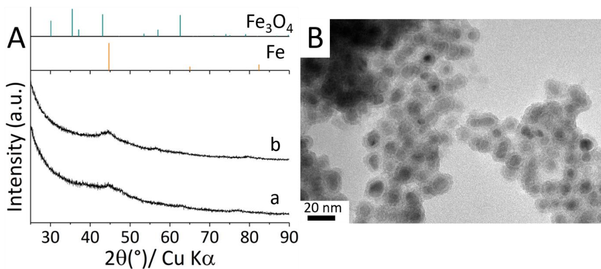
Figure S6-III. (A) Powder XRD patterns of the powders obtained from the reaction of Fe-Fe 3 O 4 nanoparticles with NaBH 4 in the molten eutectic mixture LiCl:KCl at 600 °C for 3 h with initial Fe:B atomic ratios (a) 1:1.3 and (b) 2:1.3. (B) TEM image of the sample obtained with Fe:B = 2:1.3.
