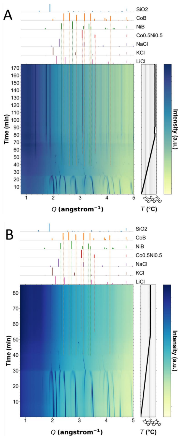
Figure 10. Synchrotron radiation in situ XRD diagrams recorded during the reaction of Ni-Co nanoparticles with NaBH 4 (Metal:B = 1:2.6 at.) in LiCl:KCl (44/56 mass.): (A) Ramping up to 800 °C, (B) ramping up to 555 °C.
