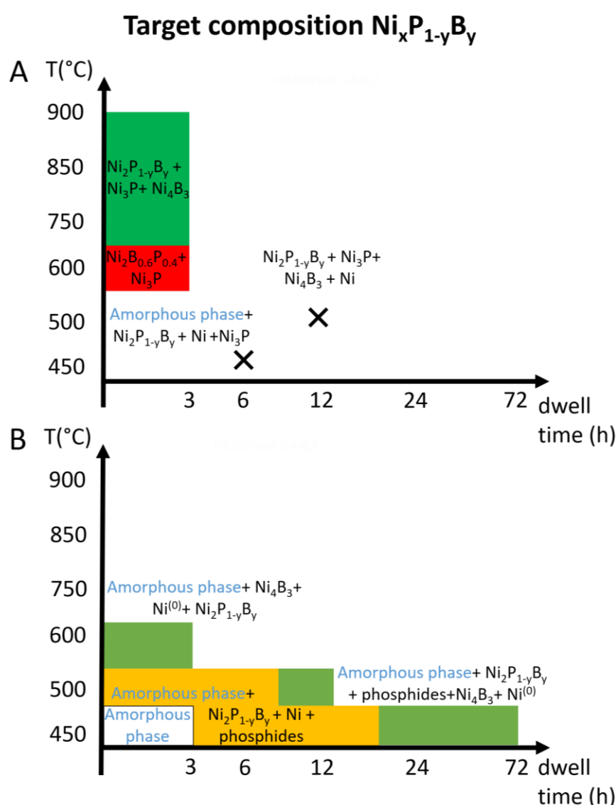
Figure 6. Screening of experimental conditions (dwell time, temperature T ) performed to target reported Ni-B-P ternary phases using Ni:B:P ratios of (A) 3:6:0.7, (B) 2:4:0.4. The red area corresponds to the conditions of the Rietveld refinement described above, the green areas
