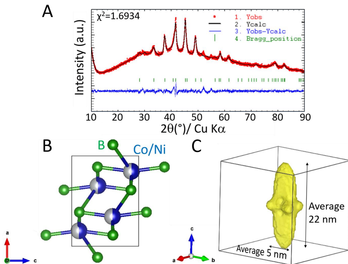
Figure 7. (A) Powder XRD pattern and corresponding Rietveld refinement of Ni-Co-B (M:B = 1:2.6 at.) in LiI:KI (58:42 mass.) at 600 °C for 3 h. The refinement is performed by maintaining the CoB space group and the atomic positions. (B) corresponding crystal structure and (C) model of particle morphology.
