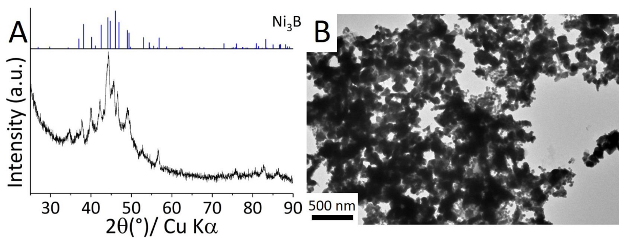
Figure S2-XI. (A) Powder XRD pattern (A) and (B) TEM image of Ni 3 B nanoparticles synthesized without impregnation using a hexane dispersion of nickel nanoparticles.
