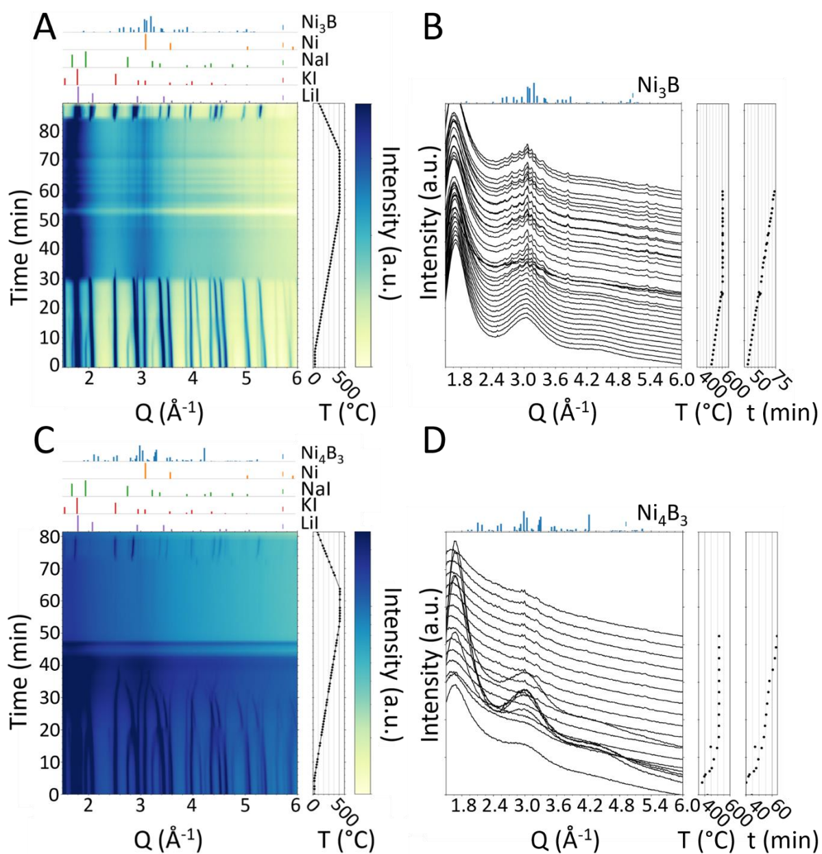
Figure S2-II. In situ XRD diagrams recorded during the synthesis of (A, B) \text{Ni}_3\text{B} and (C, D) \text{Ni}_4\text{B}_3 nanocrystals.
