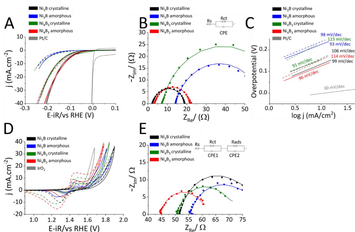
Figure 2. Electrochemical properties of \text{Ni}_3\text{B} and \text{Ni}_4\text{B}_3 nanocrystals and of their corresponding amorphous nanoparticle intermediates. HER study in aqueous Ar saturated 0.5 M \text{H}_2\text{SO}_4 electrolyte: (a) CV curves at the 1 st cycle (continuous lines) and 30 th cycle (dashed lines), (b) Nyquist plot (dots) and fitting curve (continuous line) recorded at -0.23 V vs RHE after activation by 30 cyclic voltammograms, (C) Tafel slopes before (continuous lines) and after (dashed line) activation. OER study in aqueous \text{O}_2 -saturated 0.1 M KOH Fe purified electrolyte: (D) CV curves at the 1 st cycle (continuous lines) and 30 th cycle (dashed lines), (E) Nyquist plot
