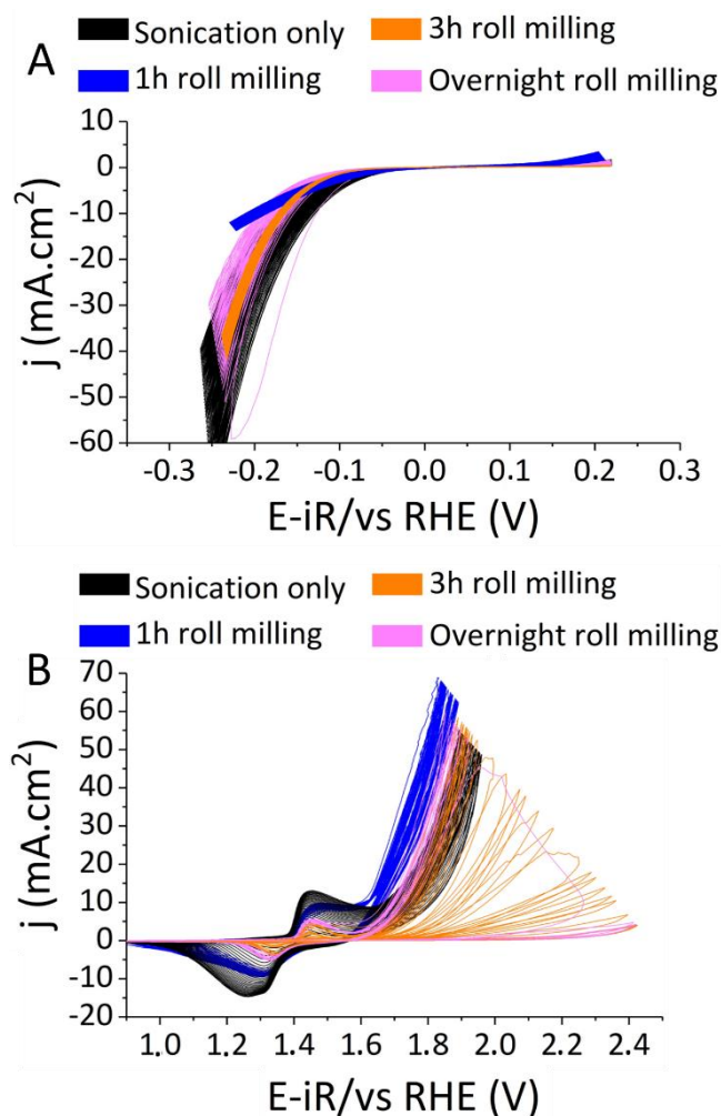
Figure 4. Cyclic voltammetry recorded under (A) HER in 0.5 M \text{H}_2\text{SO}_4 , (B) OER in Fe purified 0.1 M KOH with roll milling under argon for 1h, 3h and overnight in comparison to the case of sonication only.
