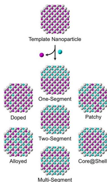
Figure 2. Examples of diverse structures reported by cation exchange reactions. Reproduced from 37 .
