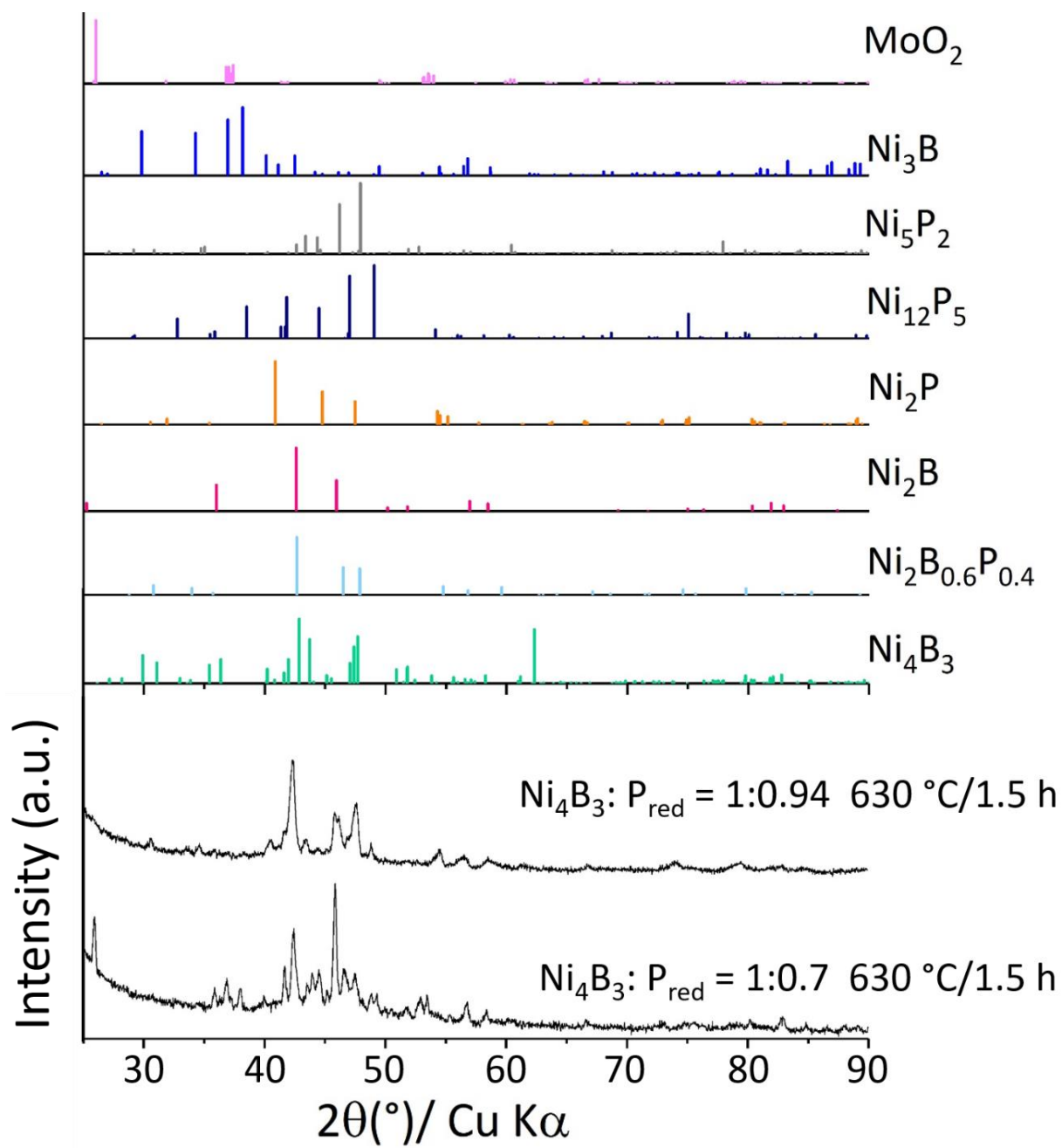
Figure S4-V. Powder XRD patterns of the products obtained from the reaction of red phosphorus with Ni 4 B 3 nanoparticles in the molten eutectic mixture LiI:KI.
