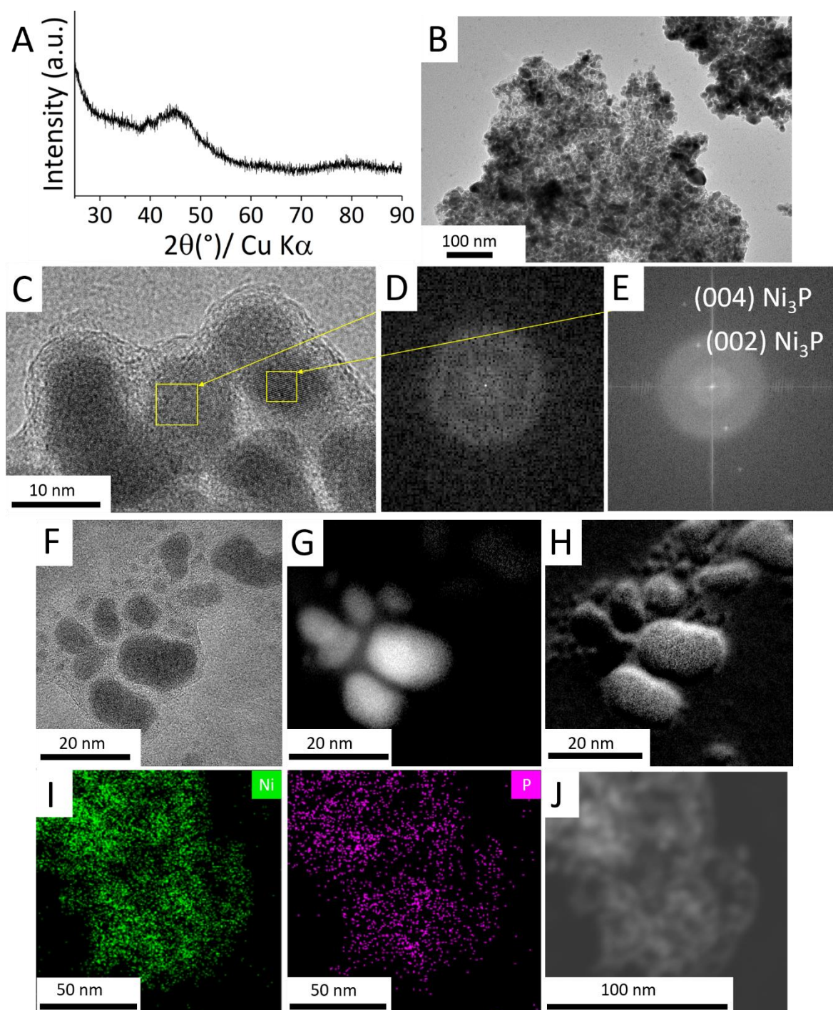
Figure 7. Nickel borophosphide obtained by reacting \text{NiCl}_2 , \text{NaBH}_4 and \text{P}_{\text{red}} (2:4:0.4 at. ratio) at 450\text{ }^\circ\text{C}/3\text{ h} in the molten eutectic mixture \text{LiCl}:\text{KCl} . (A) Powder XRD pattern, (B) TEM and (C) HRTEM images with (D-E) corresponding FFTs. (F) TEM and corresponding EFTEM images at the (G) Ni-L and (H) B-K edges. (I) STEM-EDX chemical maps of Ni and P with (J) the corresponding TEM image.
