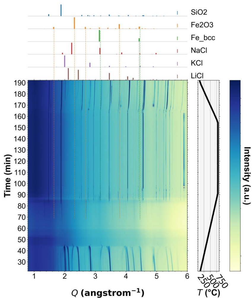
Figure S6-IV. Synchrotron radiation-based in situ XRD diagrams recorded during the reaction of bcc-Fe nanoparticles from the Peng et al. procedure 13 with NaBH 4 (initial Fe:B = 1:1.3 at.) in the eutectic mixture LiCl:KCl. The heating ramp was recalibrated based on the heating point of the salt mixture.
