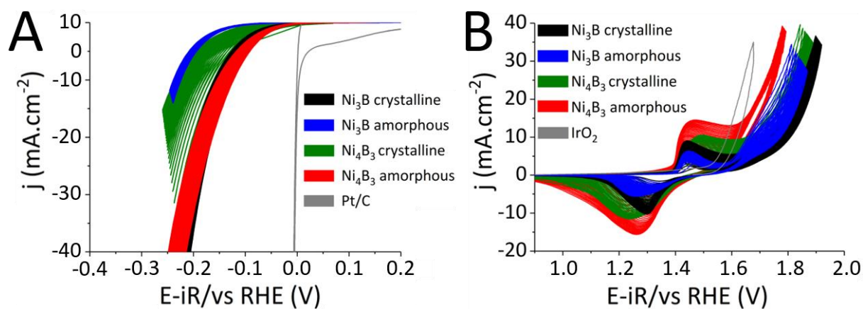
Figure S3-I. Cyclic voltammetry recorded with boride catalysts for 30 cycles until stabilization of the electrochemical response, under (A) HER conditions in Ar-saturated 0.5 M H 2 SO 4 , (B) OER in Fe purified O 2 -saturated 0.1 M KOH. For comparison, The Pt/C and IrO 2 benchmark curves corresponding to the first CV cycle are also plotted.
