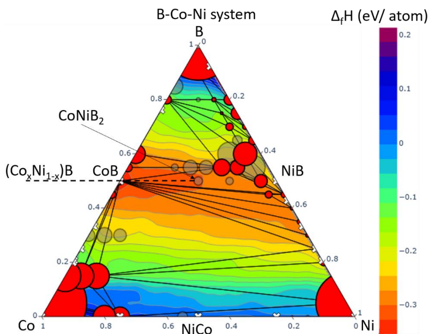
Figure 4. Predicted formation energy diagram of Ni-Co-B according to Matlearn 49 . White crosses indicate reported compositions in the training database. Red areas show the low formation energy zones. Red circles indicate predicted compositions on the convex hull, grey circles indicate compositions slightly above the convex hull, hence potentially metastable. The dotted line represents the targeted compositions.
