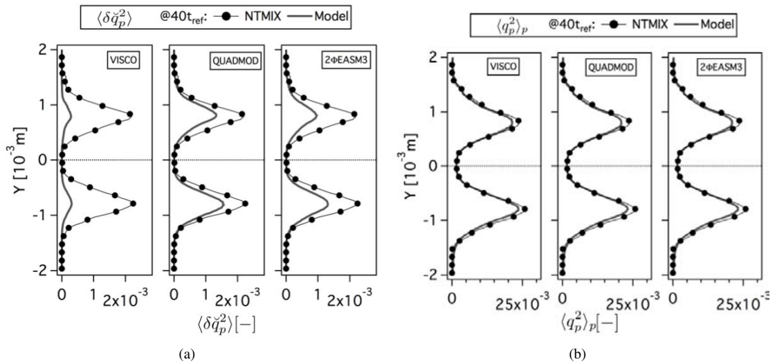
Figure E.11: Comparison of Eulerian and Lagrangian (a) mean Random Uncorrelated Energy ( \langle \delta \check{q}_p^2 \rangle ) and (b) mean mesoscopic ( \langle \check{q}_p^2 \rangle_p ) particle energies at 40t_{ref} . Normalized by the square of the initial particle velocity in X-direction at the center of the slab. LR_St033_# case.
