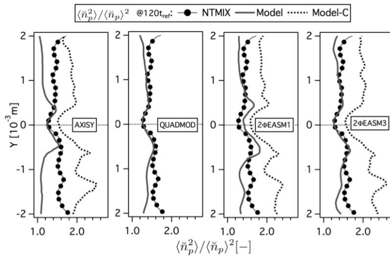
Figure 5.41: Comparison of Eulerian and Lagrangian RMS particle segregation ( \langle \check{n}_p^2 \rangle / \langle \check{n}_p \rangle^2 ) at 120t_{ref} . LR_St3_# case.
