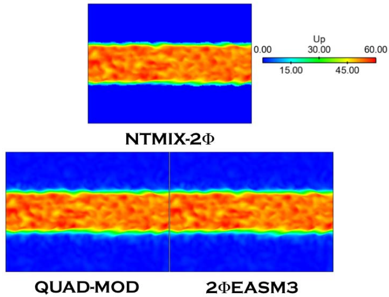
Figure F.17: Comparison of Lagrangian (NTMIX-2 \Phi ) and Eulerian particle velocity magnitude ( U_p ) at 5t_{ref} . HR_St1_# case.
