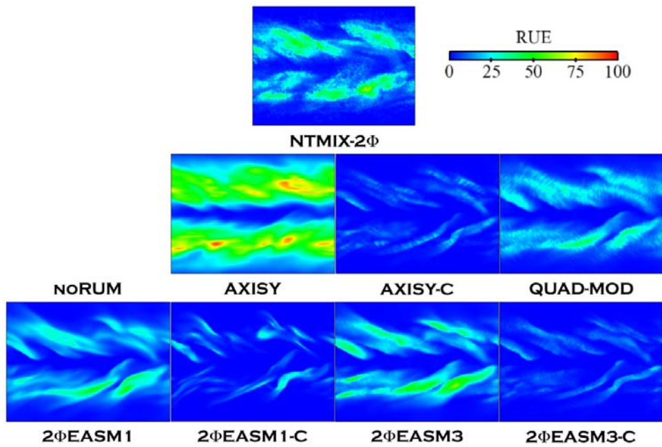
Figure D.22: Comparison of Lagrangian (NTMIX-2 \Phi ) and Eulerian Random Uncorrelated Energy at 80t_{ref} . LR_St3_# case.
