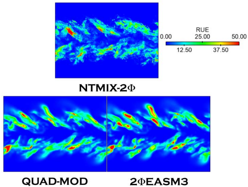
Figure F.20: Comparison of Lagrangian (NTMIX-2 \Phi ) and Eulerian Random Uncorrelated Energy at 40t_{ref} . HR_St1_# case.
