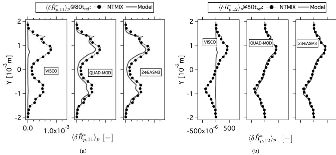
Figure 5.58: Comparison of Eulerian and Lagrangian (a) mean deviatoric RUM stress tensor XX component ( \langle \delta \check{R}_{p,11}^* \rangle_p ) and (b) mean deviatoric RUM stress tensor XY component ( \langle \delta \check{R}_{p,12}^* \rangle_p ) at 80t_{ref} . Normalized by the square of the initial particle velocity in X-direction at the center of the slab. LR_St033_# case.
