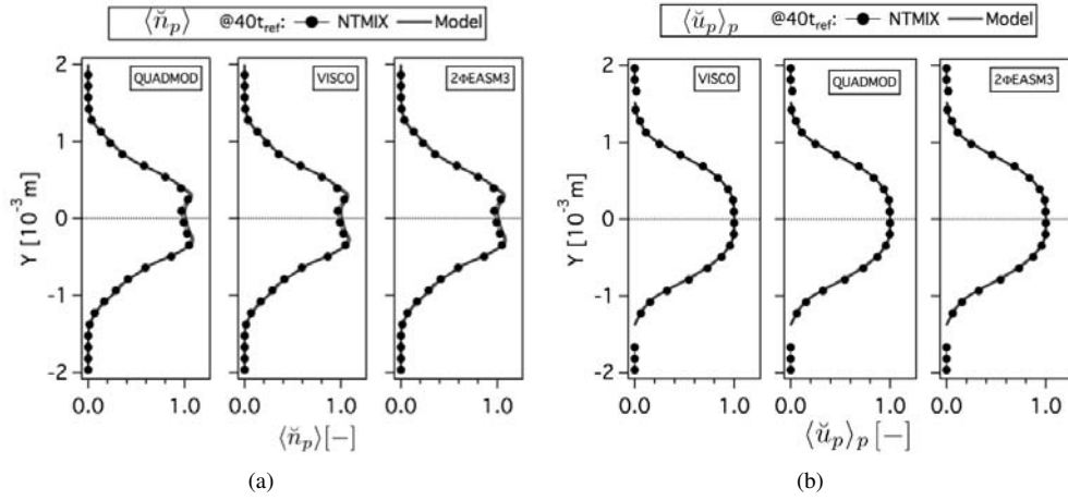
Figure E.8: Comparison of Eulerian and Lagrangian (a) mean particle number density ( \langle \check{n}_p \rangle , normalized by the initial particle number density at the center of the slab) and (b) mean particle velocity in X-direction ( \langle \check{u}_p \rangle_p , normalized by the initial particle velocity in X-direction at the center of the slab) at 40t_{ref} . LR_St033_# case.
