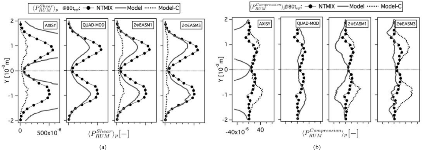
Figure D.13: Comparison of Eulerian and Lagrangian (a) mean production of RUM energy by shear components ( \langle P_{RUM}^{Shear} \rangle_p ) and (b) mean productions of RUM energy by compression ( \langle P_{RUM}^{Compression} \rangle_p ) at 80t_{ref} . Normalized by the square of the initial particle velocity in X-direction at the center of the slab and the reference time ( t_{ref} ). LR_St3_# case.
