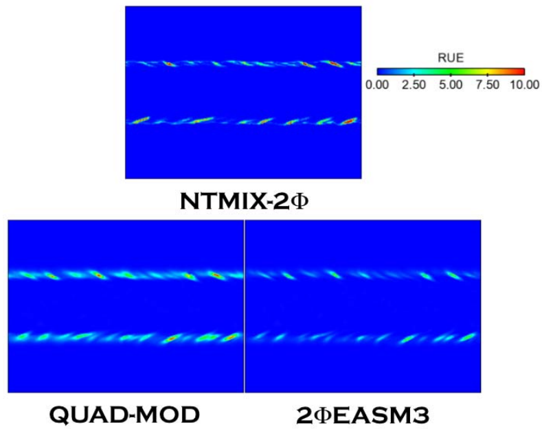
Figure F.19: Comparison of Lagrangian (NTMIX-2 \Phi ) and Eulerian Random Uncorrelated Energy at 5t_{ref} . HR_St1_# case.
