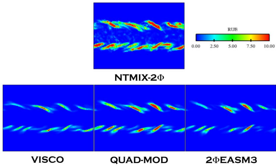
Figure E.19: Comparison of Lagrangian ( NTMIX-2\Phi ) and Eulerian Random Uncorrelated Energy at 20t_{ref} . LR_St033_# case.
