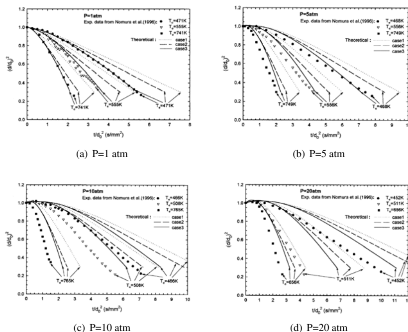
Figure 6.2: Computational results from Yang & Wong (2002) on evaporation of single isolated n -heptane droplets at different pressures and temperatures. Comparison with the experimental results of Nomura et al. (1996). Extracted from Yang & Wong (2002).
