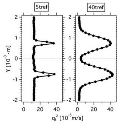
Figure B.4: Comparison of Eulerian and Lagrangian carrier phase turbulent kinetic energy ( q_t^2 ) at 5 and 40t_{ref} . HR_St1_# case. Simulations performed with AVBP (—) and NTMIX- 2\Phi (—●—).
