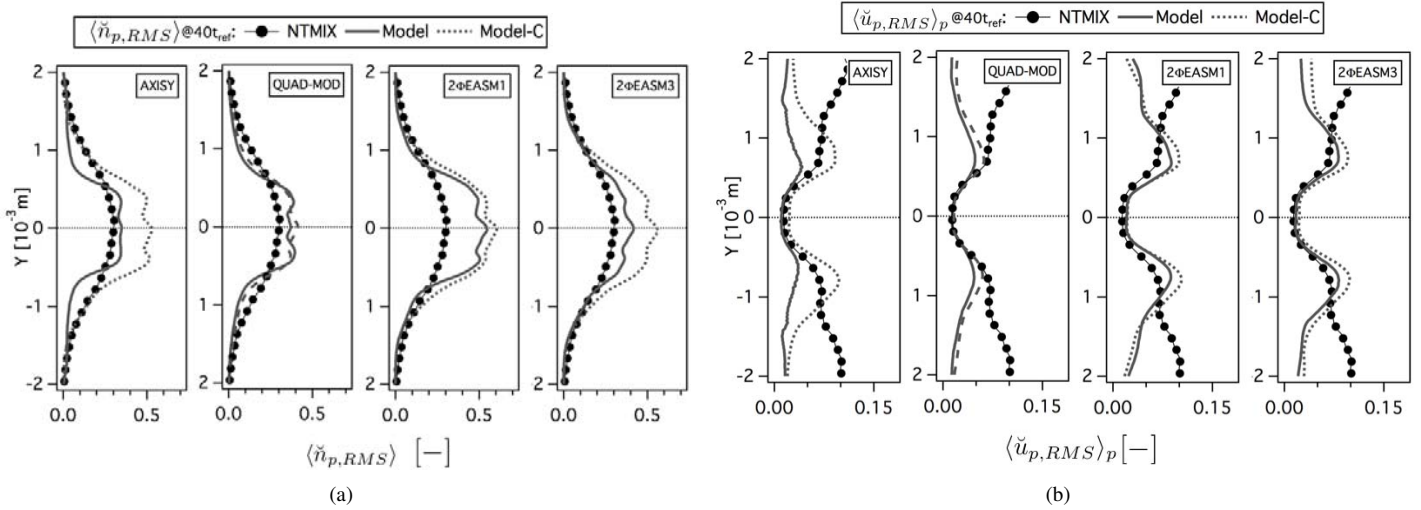
Figure D.2: Comparison of Eulerian and Lagrangian (a) RMS particle number density ( \langle \check{n}_{p,RMS} \rangle , normalized by the initial particle number density at the center of the slab) and (b) RMS particle velocity in X-direction ( \langle \check{u}_{p,RMS} \rangle_p , normalized by the initial particle number density at the center of the slab) at 40t_{ref} . LR_St3_# case.
