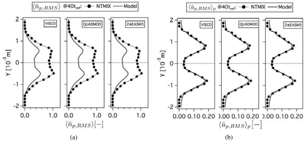
Figure E.9: Comparison of Eulerian and Lagrangian (a) RMS particle number density ( \langle \check{n}_{p,RMS} \rangle , normalized by the initial particle number density at the center of the slab) and (b) RMS particle velocity in X-direction ( \langle \check{u}_{p,RMS} \rangle_p , normalized by the initial particle number density at the center of the slab) at 40t_{ref} . LR_St033_# case.
