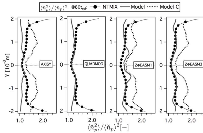
Figure D.11: Comparison of Eulerian and Lagrangian RMS particle segregation ( \langle \check{n}_p^2 \rangle / \langle \check{n}_p \rangle^2 ) at 80t_{ref} . LR_St3_# case.
