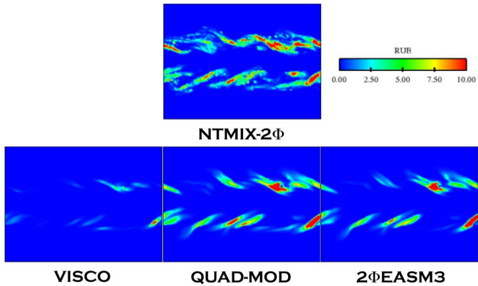
Figure E.20: Comparison of Lagrangian ( NTMIX-2\Phi ) and Eulerian Random Uncorrelated Energy at 40t_{ref} . LR_St033_# case.
