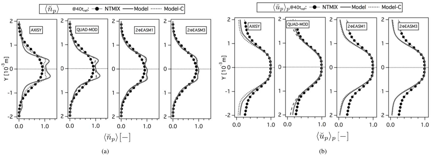
Figure D.1: Comparison of Eulerian and Lagrangian (a) mean particle number density ( \langle \check{n}_p \rangle , normalized by the initial particle number density at the center of the slab) and (b) mean particle velocity in X-direction ( \langle \check{u}_p \rangle_p , normalized by the initial particle velocity in X-direction at the center of the slab) at 40t_{ref} . LR_St3_# case.
