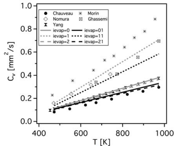
Figure 7.9: Comparison of the vaporization rate of n -heptane isolated droplets, versus temperature. Experimental results of Chauveau et al. (2008) , Nomura et al. (1996) , Yang & Wong (2001) , Morin et al. (2000) and Ghassemi et al. (2006)
