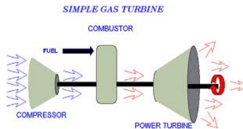
Figure 1.2: Simplified sketch of the thermodynamic cycle of a gas turbine. Source Wikipedia.
