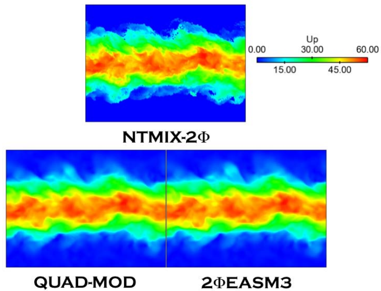
Figure F.18: Comparison of Lagrangian (NTMIX-2 \Phi ) and Eulerian particle velocity magnitude ( U_p ) at 40t_{ref} . HR_St1_# case.
