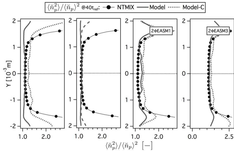
Figure D.3: Comparison of Eulerian and Lagrangian RMS particle segregation ( \langle \check{n}_p^2 \rangle / \langle \check{n}_p \rangle^2 ) at 40t_{ref} . LR_St3_# case.
