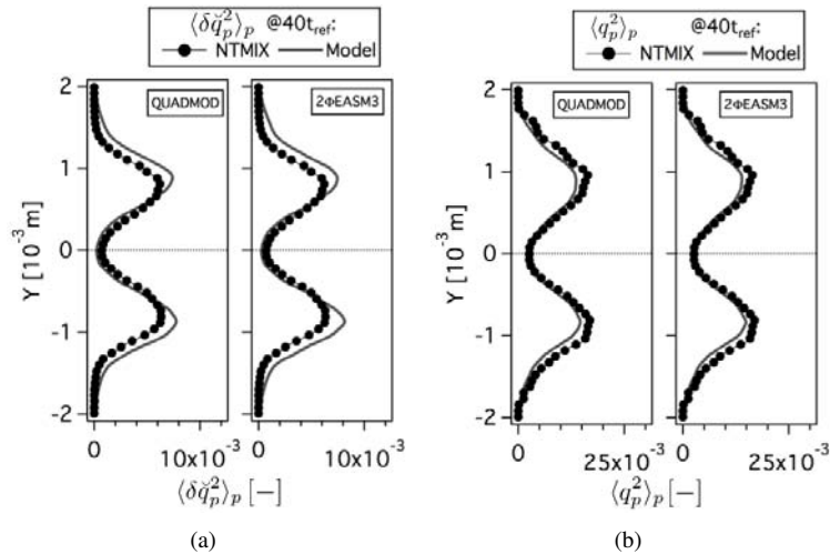
Figure F.11: Comparison of Eulerian and Lagrangian (a) mean Random Uncorrelated Energy ( \langle \delta \check{q}_p^2 \rangle_p ) and (b) mean mesoscopic ( \langle \check{q}_p^2 \rangle_p ) particle energies at 40t_{ref} . Normalized by the square of the initial particle velocity in X-direction at the center of the slab. HR_St1_# case.
