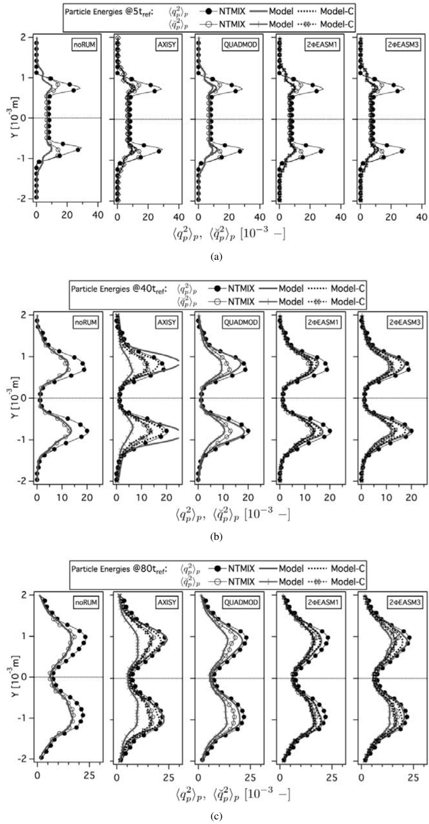
Figure 5.22: Comparison of Eulerian and Lagrangian mean total energy ( \langle q_p^2 \rangle_p ) and mean mesoscopic energy ( \langle \check{q}_p^2 \rangle_p ) at 5, 40 and 80t_{ref} . Normalized by the square of the initial particle velocity in X-direction at the center of the slab. LR_St1_# case.
