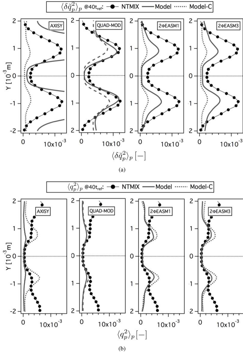
Figure D.4: Comparison of Eulerian and Lagrangian (a) mean Random Uncorrelated Energy ( \langle \delta \tilde{q}_p^2 \rangle_p ) and (b) mean mesoscopic ( \langle \text{meso}q_p^2 \rangle_p ) and mesoscopic ( \langle q_p^2 \rangle_p ) particle energies at 40t_{ref} . Normalized by the square of the initial particle velocity in X-direction at the center of the slab. LR_St3_# case.
