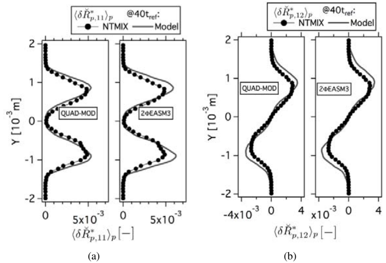
Figure F.13: Comparison of Eulerian and Lagrangian (a) mean deviatoric RUM stress tensor XX component ( \langle \delta \check{R}_{p,11}^* \rangle_p ) and (b) mean deviatoric RUM stress tensor XY component ( \langle \delta \check{R}_{p,12}^* \rangle_p ) at 40t_{ref} . Normalized by the square of the initial particle velocity in X-direction at the center of the slab. HR_St1_# case.
