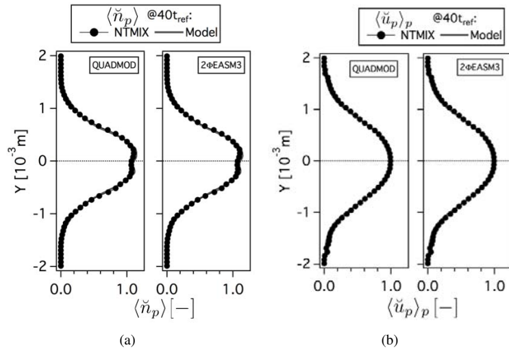
Figure F.8: Comparison of Eulerian and Lagrangian (a) mean particle number density ( \langle \check{n}_p \rangle , normalized by the initial particle number density at the center of the slab) and (b) mean particle velocity in X-direction ( \langle \check{u}_p \rangle_p , normalized by the initial particle velocity in X-direction at the center of the slab) at 40t_{ref} . HR_St1_# case.
