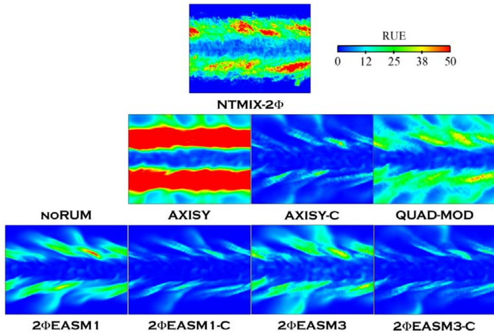
Figure D.21: Comparison of Lagrangian (NTMIX-2 \Phi ) and Eulerian Random Uncorrelated Energy at 40t_{ref} . LR_St3_# case.
