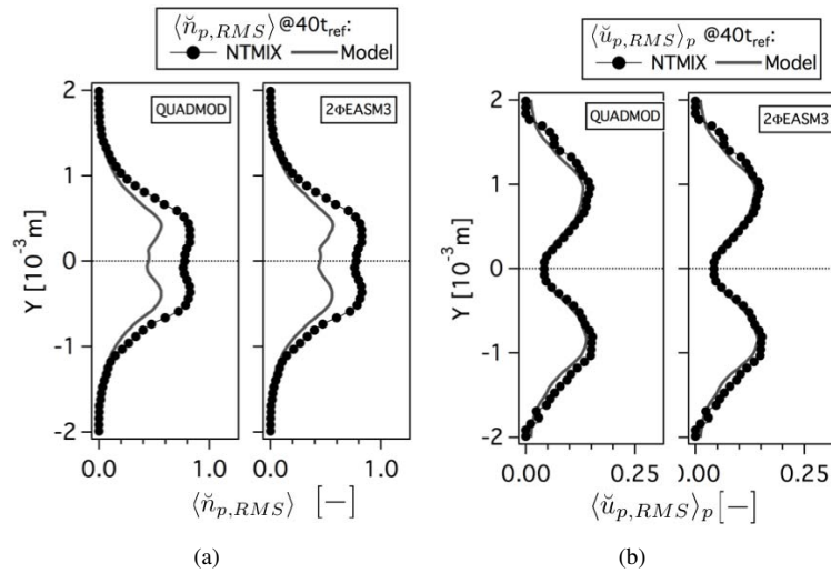
Figure F.9: Comparison of Eulerian and Lagrangian (a) RMS particle number density ( \langle \check{n}_{p,RMS} \rangle , normalized by the initial particle number density at the center of the slab) and (b) RMS particle velocity in X-direction ( \langle \check{u}_{p,RMS} \rangle_p , normalized by the initial particle number density at the center of the slab) at 40t_{ref} . HR_St1_# case.
