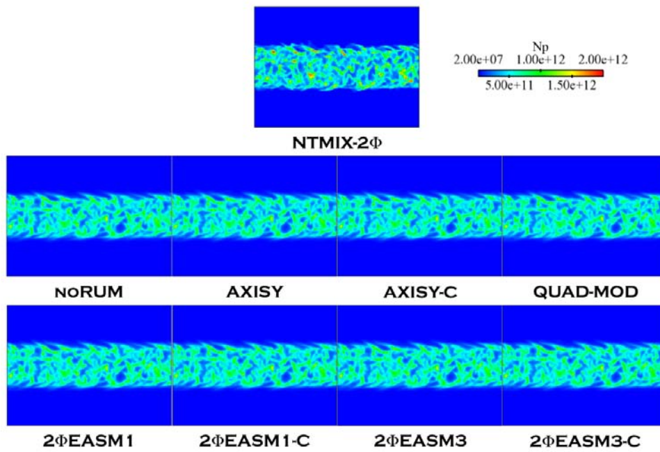
Figure C.1: Comparison of Lagrangian (NTMIX-2 \Phi ) and Eulerian particle number density ( N_p ) at 5t_{ref} . LR_St1_# case.
