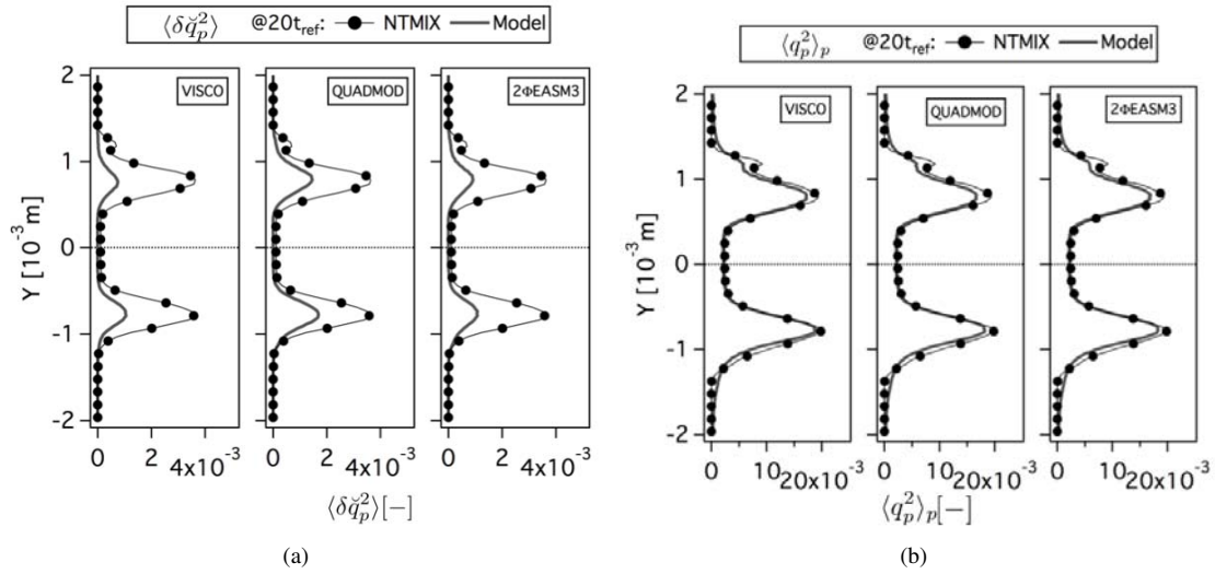
Figure E.4: Comparison of Eulerian and Lagrangian (a) mean Random Uncorrelated Energy ( \langle \delta \tilde{q}_p^2 \rangle_p ) and (b) mean mesoscopic ( \langle (q_p^2)_p \rangle ) particle energies at 20t_{ref} . Normalized by the square of the initial particle velocity in X-direction at the center of the slab. LR_St033_# case.
