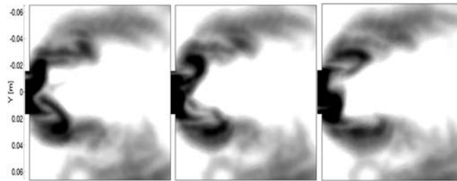
Figure 9.18: Instantaneous field of liquid volume fraction at t = 48 ms. Case RUM_Ev21
