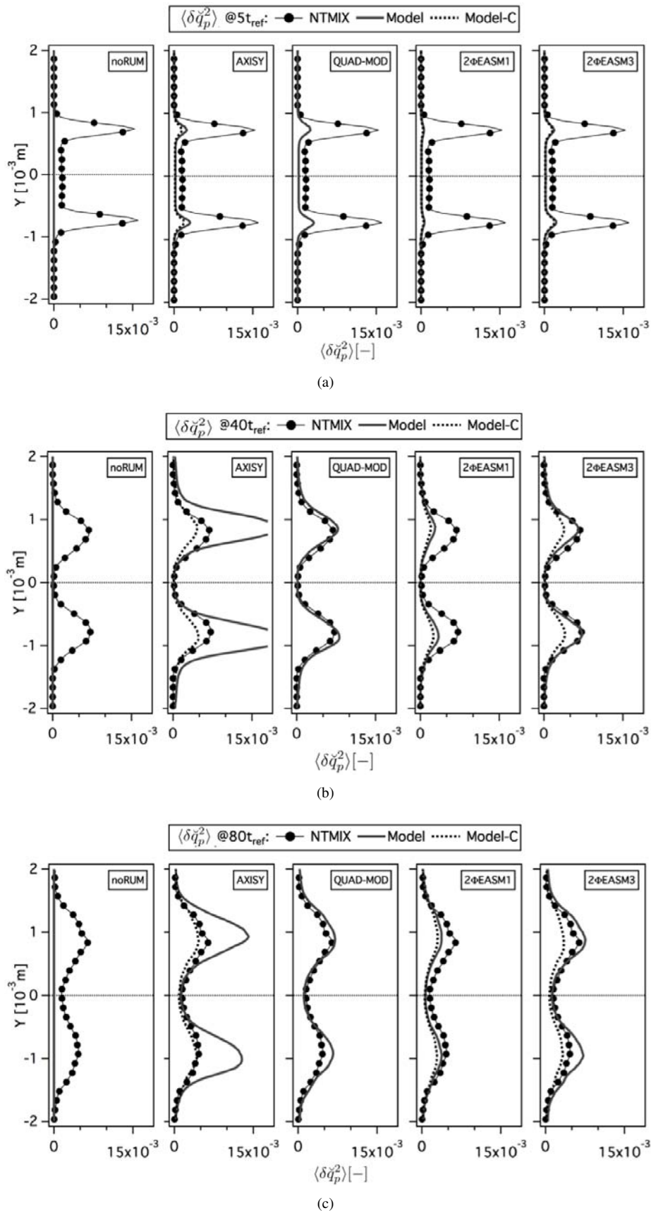
Figure 5.21: Comparison of Eulerian and Lagrangian mean Random Uncorrelated Energy ( \langle \delta \tilde{\theta}_p \rangle_p ) at 5, 40 and 80 t_{ref} . Normalized by the square of the initial particle velocity in X-direction at the center of the slab. LR_St1_# case.
