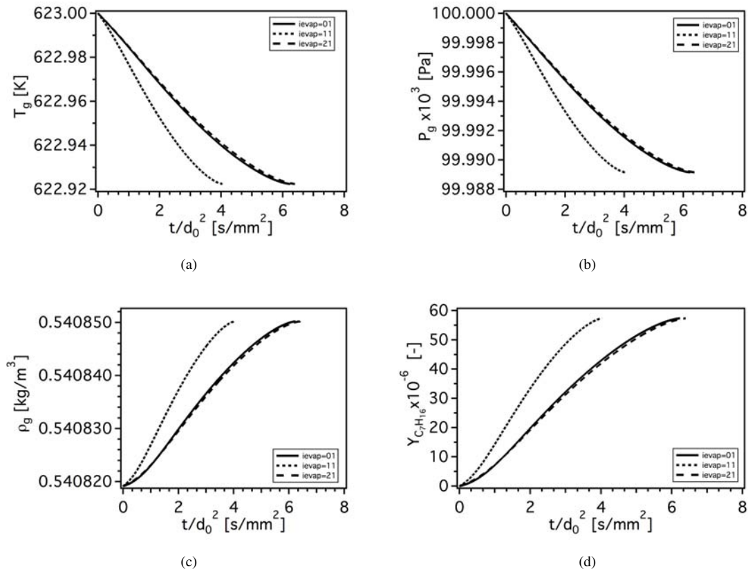
Figure 7.6: Temporal evolution of the main gaseous mixture properties: (a) gaseous temperature, (b) pressure, (c) gaseous density and (d) mass fraction of gaseous fuel. n -heptane, T_g = 623K , P_g = 1bar . Numerical simulations performed using the AS evaporation model.
